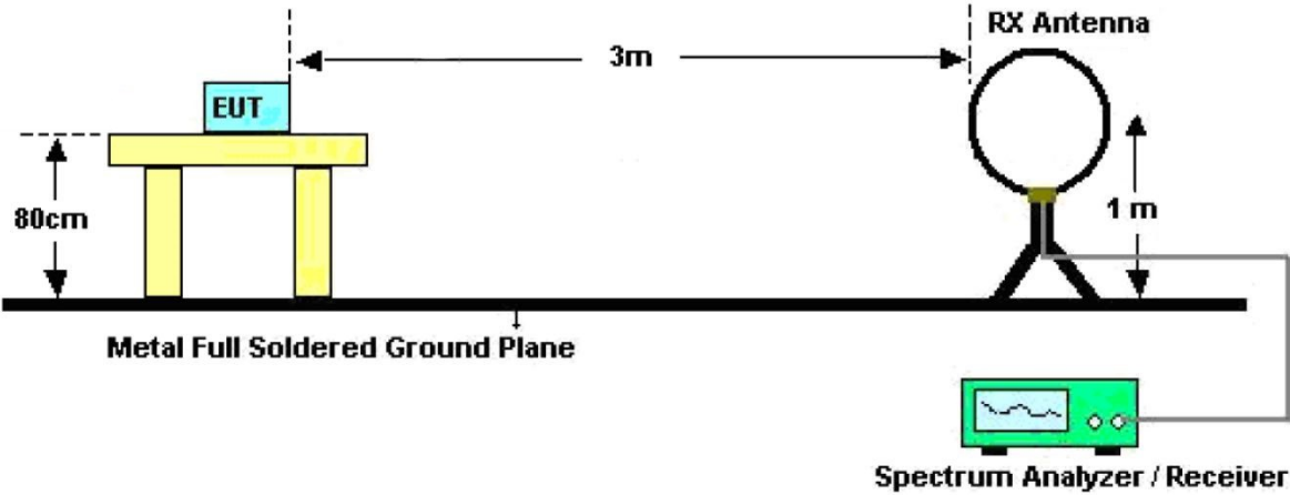
Figure 1. Below 30MHz
