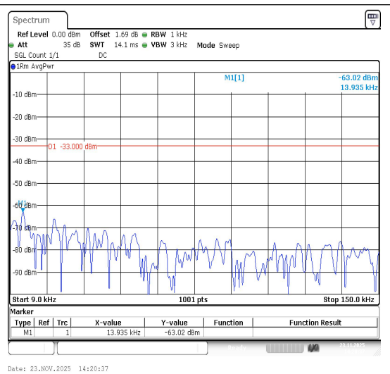
Band12-1.4MHz-16QAM-23017-1RB#0-0.009~0.1 5-PASS
