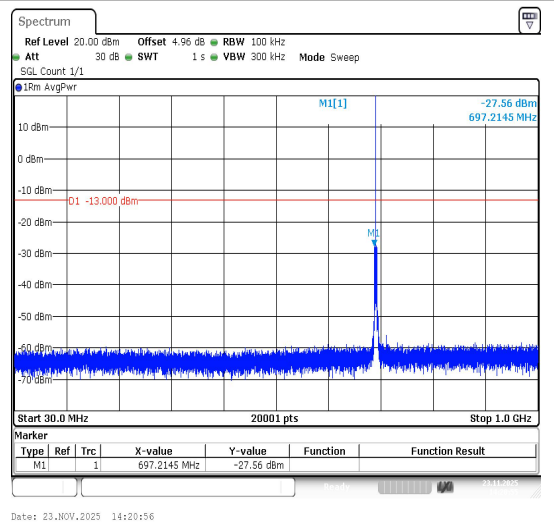
Band12-1.4MHz-16QAM-23017-1RB#0-30~1000-PASS
