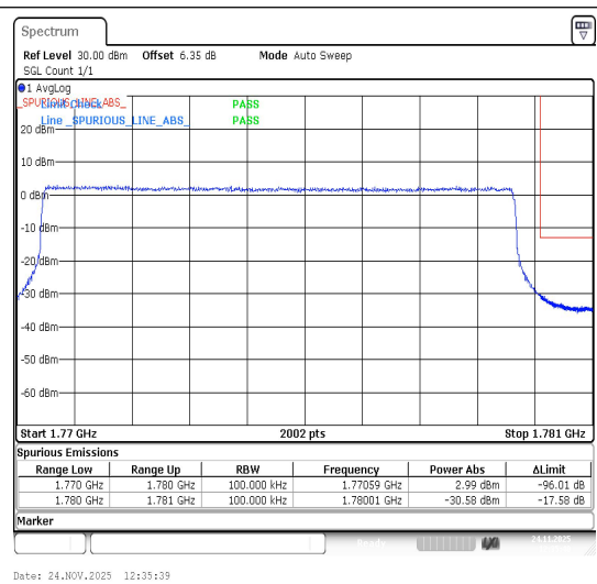
Band66-10MHz-16QAM-132622-50RB#0-PASS
