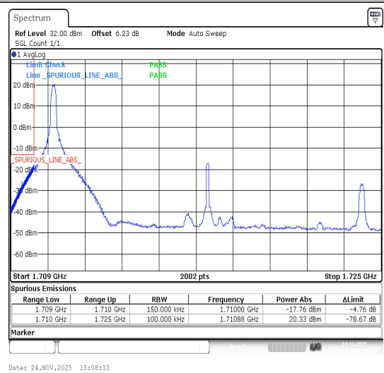
Band66-15MHz-16QAM-132047-1RB#0-PASS
