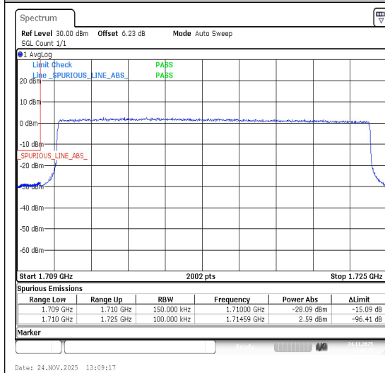
Band66-15MHz-QPSK-132047-75RB#0-PASS
