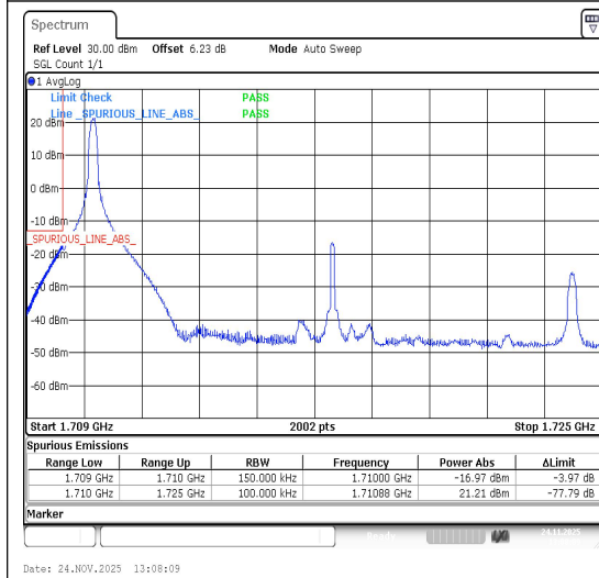
Band66-15MHz-QPSK-132047-1RB#0-PASS
