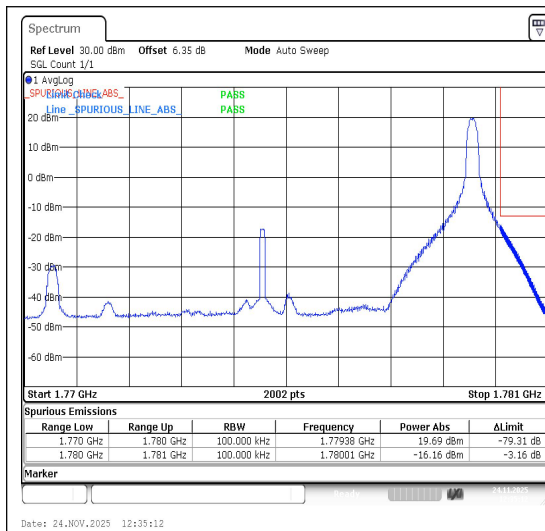
Band66-10MHz-16QAM-132622-1RB#49-PASS
