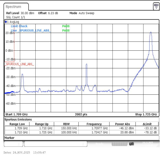
Band66-15MHz-QPSK-132047-1RB#74-PASS
