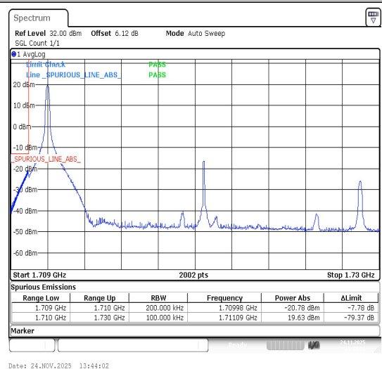
Band66-20MHz-16QAM-132072-1RB#0-PASS
