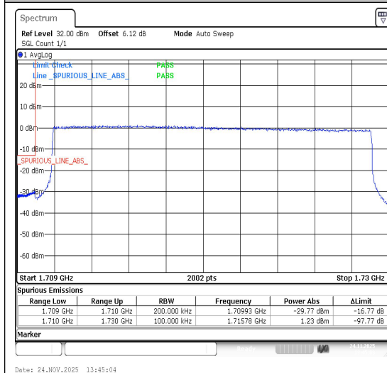
Band66-20MHz-QPSK-132072-100RB#0-PASS
