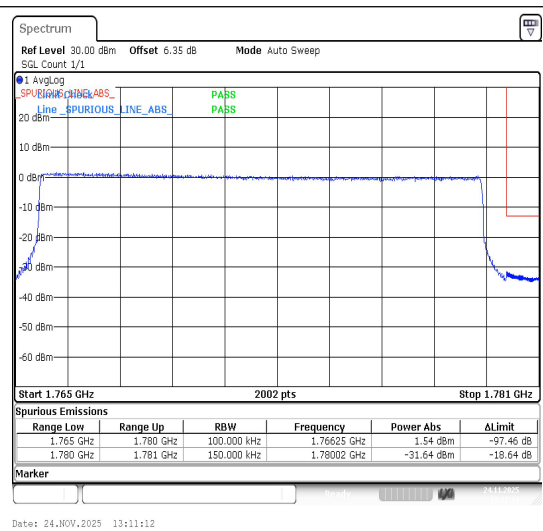
Band66-15MHz-16QAM-132597-75RB#0-PASS
