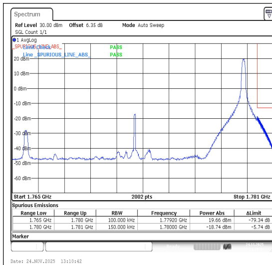
Band66-15MHz-16QAM-132597-1RB#74-PASS
