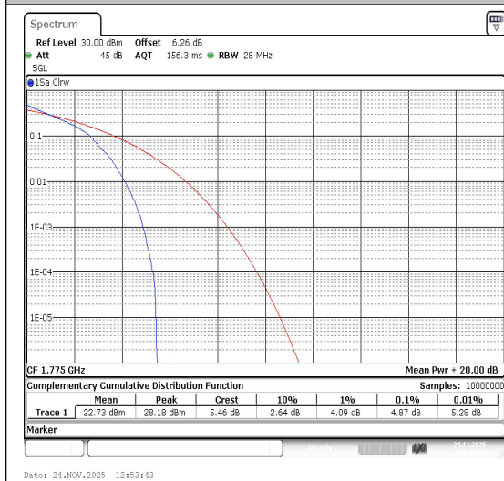
Band66-10MHz-QPSK-132622-1RB#0-PASS
