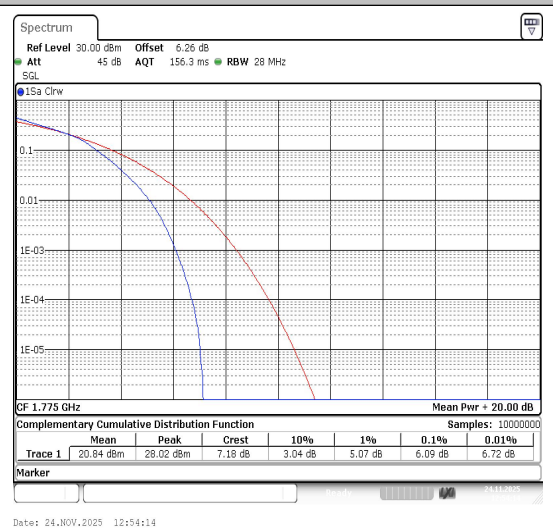
Band66-10MHz-16QAM-132622-50RB#0-PASS
