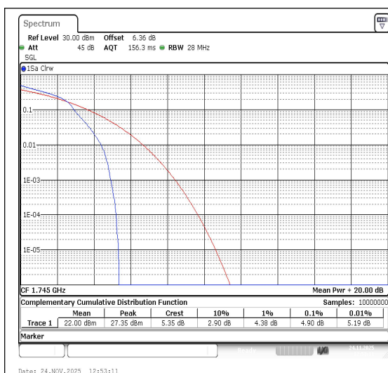
Band66-10MHz-16QAM-132322-1RB#0-PASS
