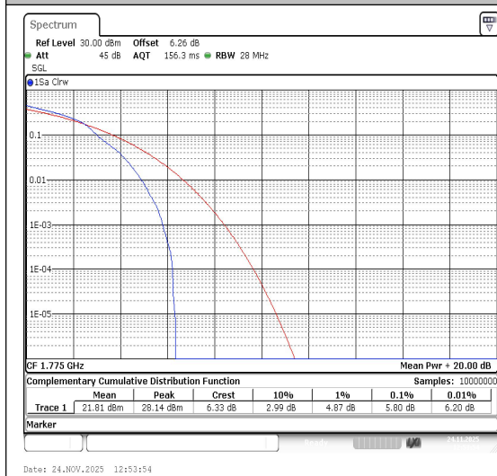
Band66-10MHz-16QAM-132622-1RB#0-PASS
