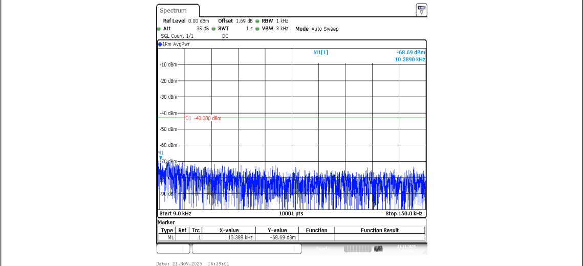
Band2-9262-5-0.009~0.15MHz-PASS
