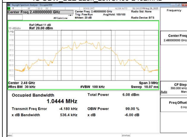
IC OBW_BLE 125k_HighCH39-2480MHz
