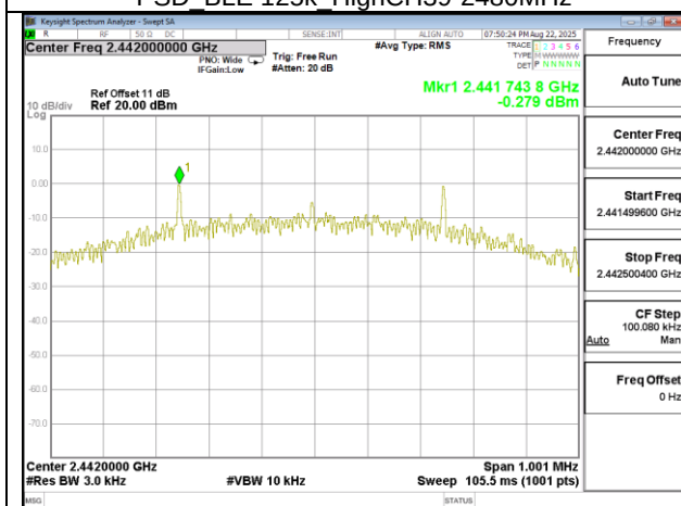
PSD_BLE 500k_MidCH20-2442MHz
