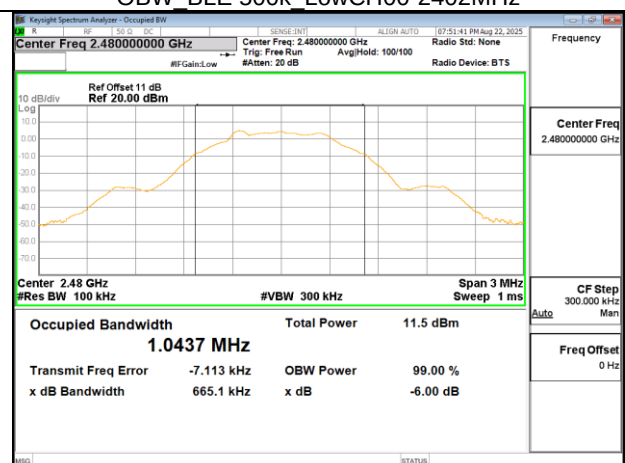
OBW_BLE 500k HighCH39-2480MHz
