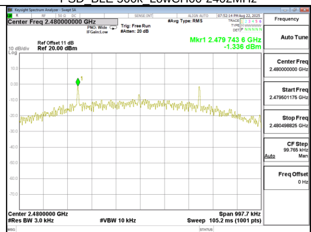
PSD_BLE 500k_HighCH39-2480MHz
