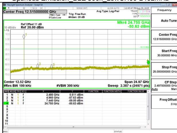
Spurious Emission BLE 500k HighCH39-2480MHz
