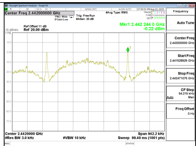
PSD_BLE 125k_MidCH20-2442MHz
