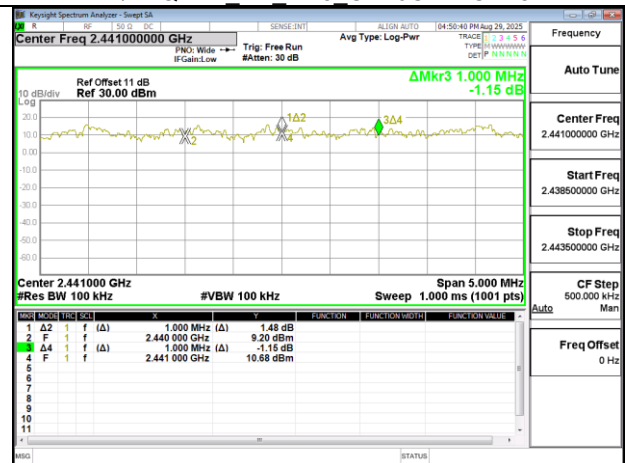
8DPSK 3M DH5 CH38CH39CH40
