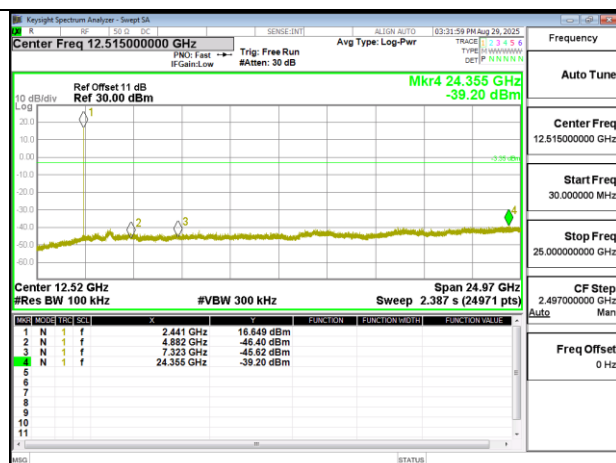
Spurious Emission \pi/4 DQPSK 2M DH5 2441MHz
