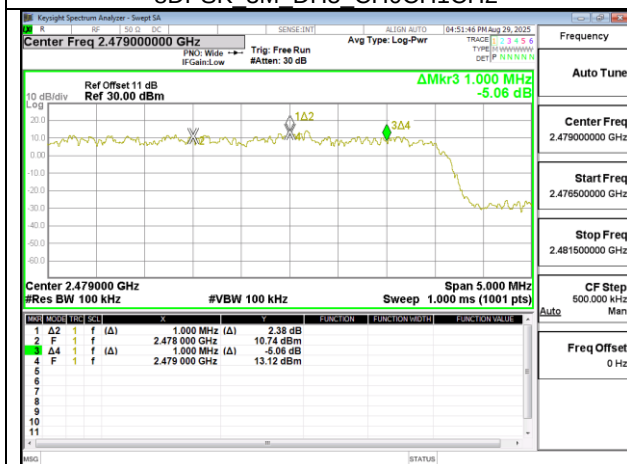
8DPSK 3M DH5 CH76CH77CH78
