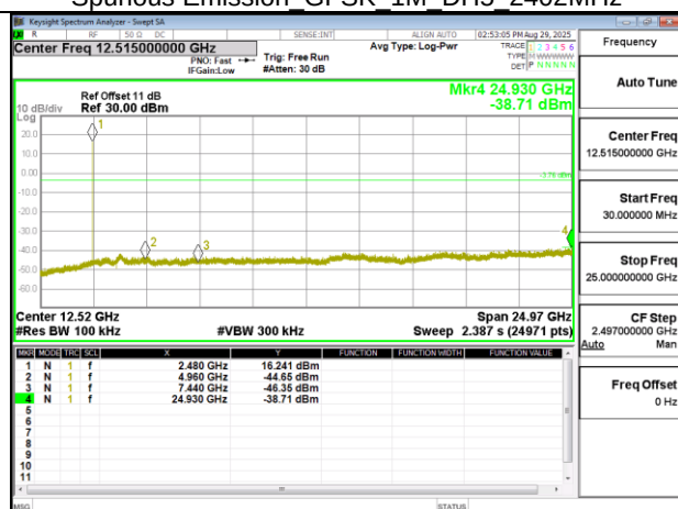
Spurious Emission GFSK 1M DH5 2480MHz
