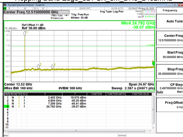
Spurious Emission GFSK 1M DH5 2402MHz
