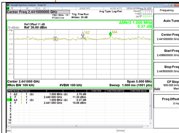
π/4DQPSK 2M DH5 CH38CH39CH40
