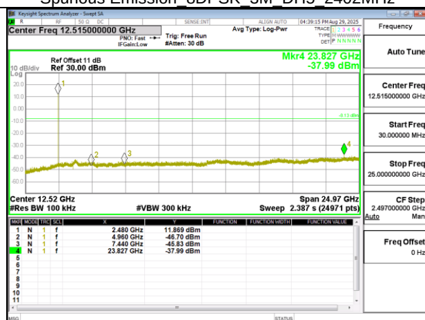
Spurious Emission 8DPSK 3M DH5 2480MHz
