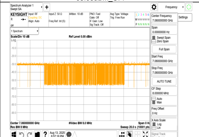
802.11ax_160MHz_CF 6985MHz_Interference_7060MHz_- 74.05dBm_ON
