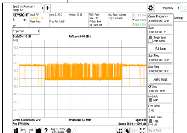
802.11ax_160MHz_CF 6985MHz_Interference_6985MHz_- 68.04dBm_ON
