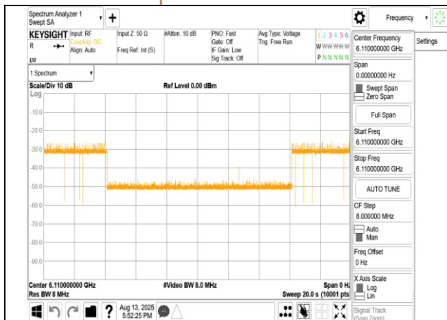
802.11ax_160MHz_CF 6185MHz_Interference_6110MHz_- 70.06dBm_OFF
