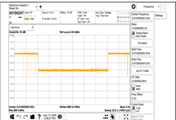
802.11ax_160MHz_CF 6985MHz_Interference_6910MHz_- 68.14dBm_OFF
