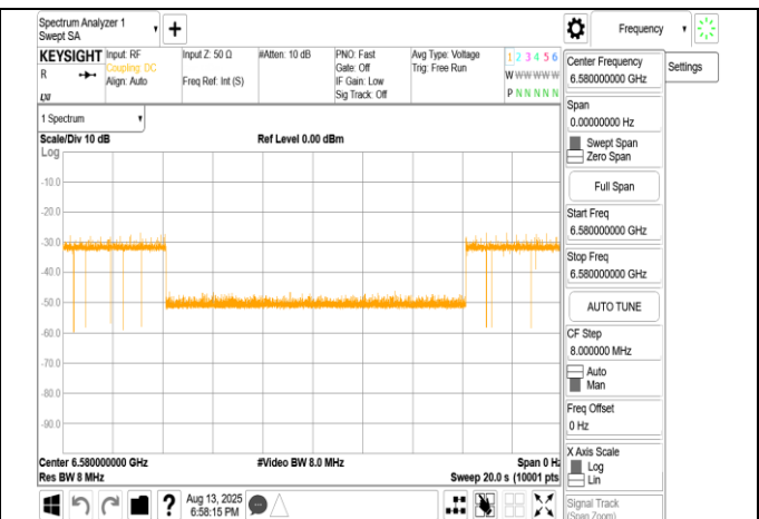
802.11ax_160MHz_CF 6505MHz_Interference_6580MHz_- 68.03dBm_OFF
