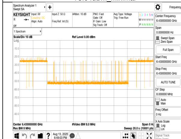
802.11ax_160MHz_CF 6505MHz_Interference_6430MHz_- 71.08dBm_Minimal
