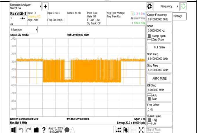
802.11ax_160MHz_CF 6985MHz_Interference_6910MHz_- 74.14dBm_ON
