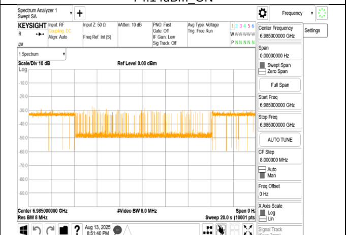
802.11ax_160MHz_CF 6985MHz_Interference_6985MHz_- 65.04dBm_Minimal
