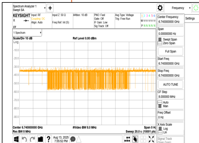
802.11ax_160MHz_CF 6665MHz_Interference_6740MHz_- 78.06dBm_ON
