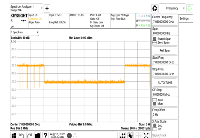
802.11ax_160MHz_CF 6985MHz_Interference_7060MHz_- 68.05dBm_OFF
