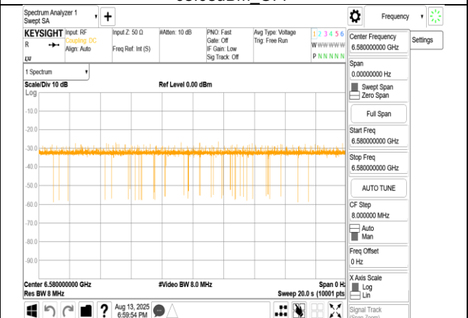
802.11ax_160MHz_CF 6505MHz_Interference_6580MHz_- 77.03dBm_ON
