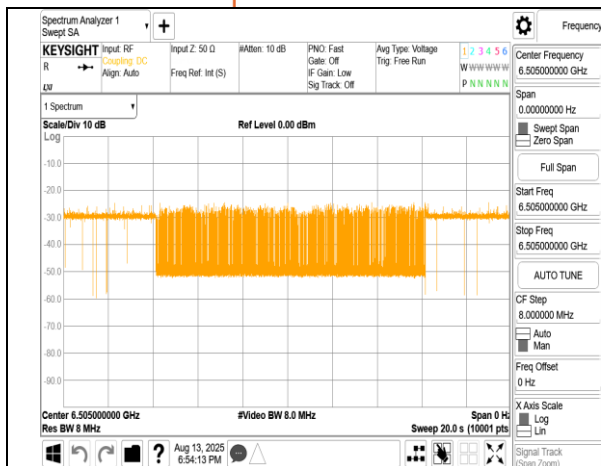
802.11ax_160MHz_CF 6505MHz_Interference_6505MHz_- 68.16dBm_ON
