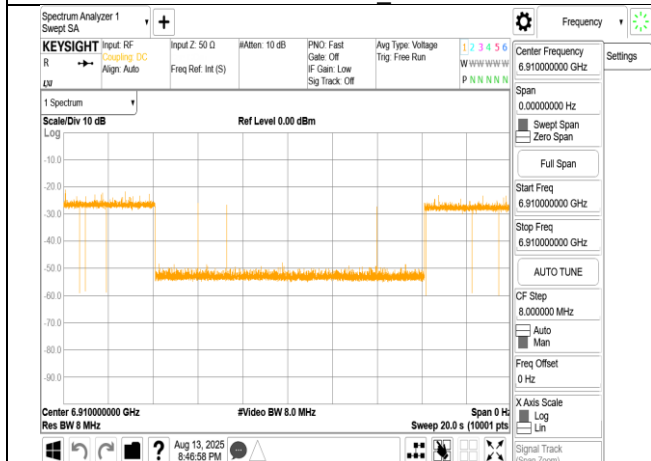
802.11ax_160MHz_CF 6985MHz_Interference_6910MHz_- 71.14dBm_Minimal
