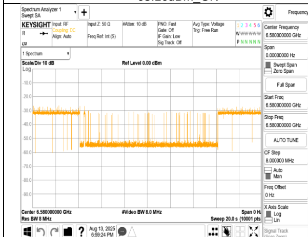
802.11ax_160MHz_CF 6505MHz_Interference_6580MHz_- 74.03dBm_Minimal
