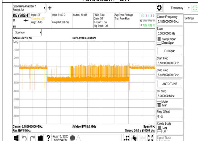
802.11ax_160MHz_CF 6185MHz_Interference_6185MHz_- 67.02dBm_Minimal
