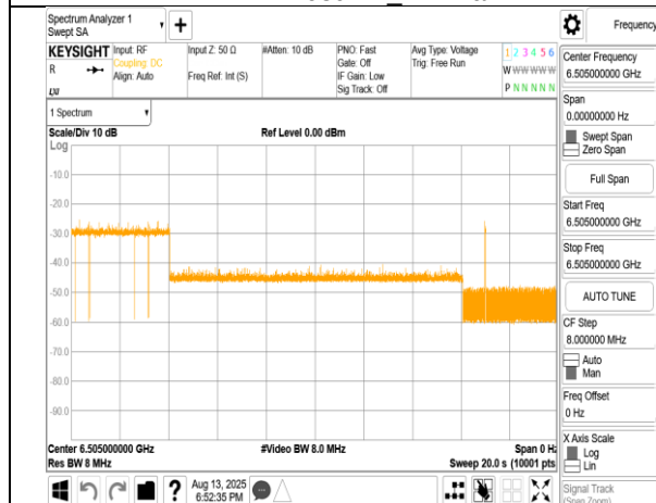
802.11ax_160MHz_CF 6505MHz_Interference_6505MHz_- 62.16dBm_OFF
