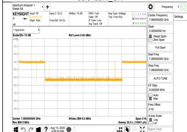
802.11ax_160MHz_CF 6985MHz_Interference_7060MHz_- 71.05dBm_Minimal
