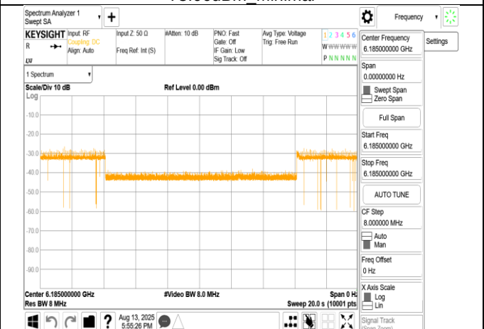
802.11ax_160MHz_CF 6185MHz_Interference_6185MHz_- 62.02dBm_OFF
