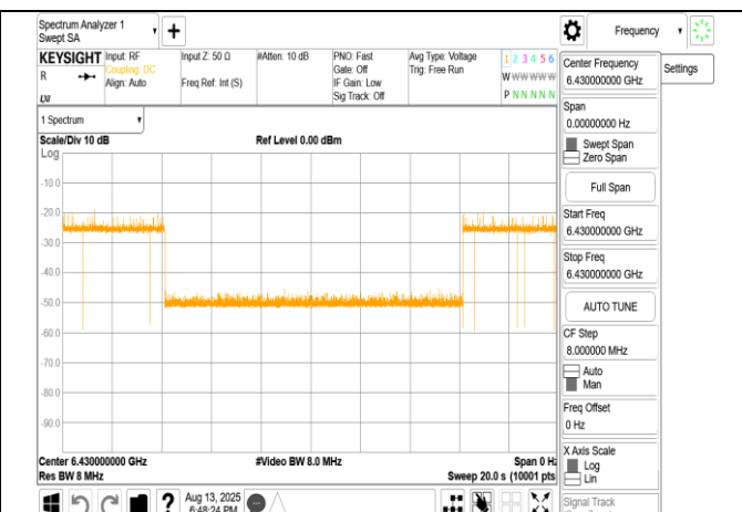
802.11ax_160MHz_CF 6505MHz_Interference_6430MHz_- 68.08dBm_OFF
