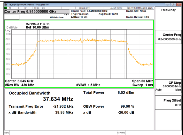
802.11ax 40MHz Chain0 6845MHz
