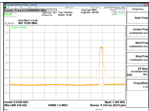
802.11n 40MHz Chain0_6925MHz
