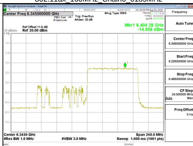
802.11ax 160MHz Chain0 6345MHz RU996 S67
