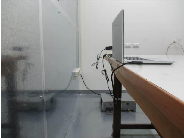
FCC_15_247_BLE_Conduction_Setup
