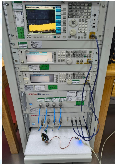
Photo of Setup for Conducted Measurement
