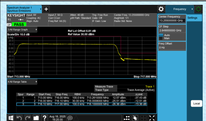
Band12-3MHz-QPSK-23165-15RB#0-PASS
