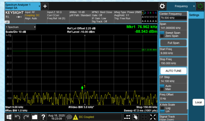
Band12-3MHz-QPSK-23165-1RB#0-0.009~0.15-PASS
