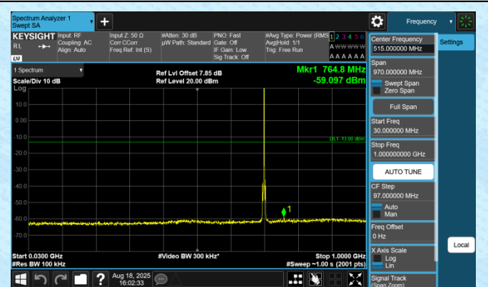
Band12-1.4MHz-QPSK-23095-1RB#0-30~1000-PASS
