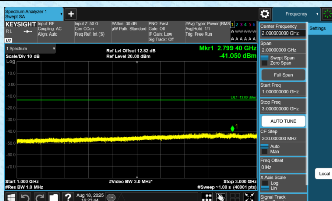
Band12-3MHz-QPSK-23165-1RB#0-1000~3000-PASS
