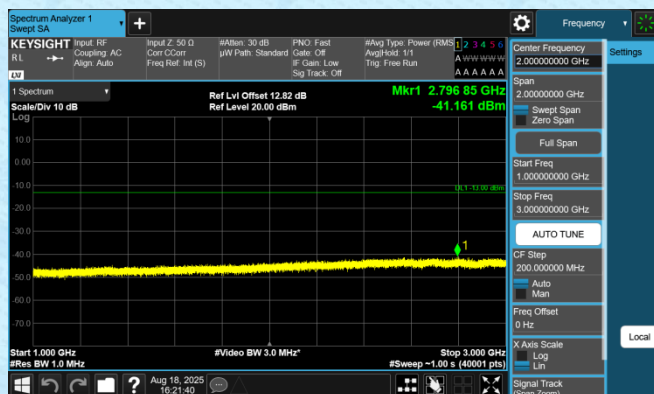
Band12-3MHz-QPSK-23025-1RB#0-1000~3000-PASS
