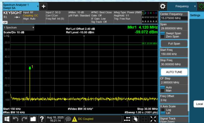
Band12-3MHz-QPSK-23025-1RB#0-0.15~30-PASS
