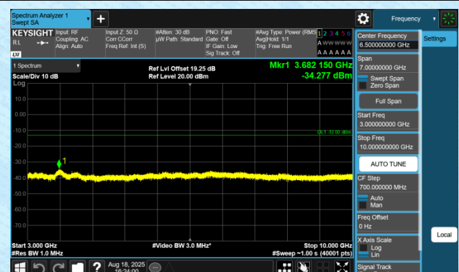
Band12-3MHz-QPSK-23165-1RB#0-3000~10000-PASS
