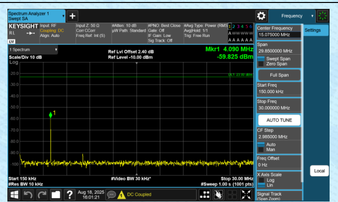
Band12-1.4MHz-QPSK-23017-1RB#0-0.15~30-PASS
