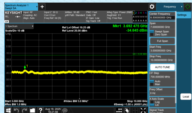
Band12-3MHz-QPSK-23025-1RB#0-3000~10000-PASS
