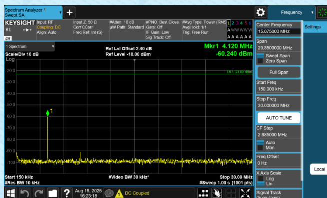
Band12-3MHz-QPSK-23165-1RB#0-0.15~30-PASS
