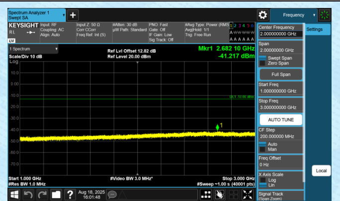
Band12-1.4MHz-QPSK-23017-1RB#0-1000~3000-PASS
