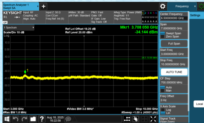
Band12-3MHz-QPSK-23095-1RB#0-3000~10000-PASS
