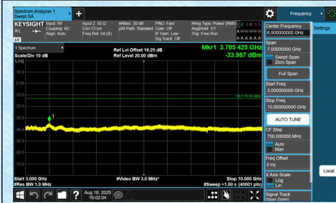
Band12-1.4MHz-QPSK-23017-1RB#0-3000~10000-PASS
