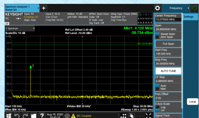
Band12-5MHz-QPSK-23035-1RB#0-0.15~30-PASS
