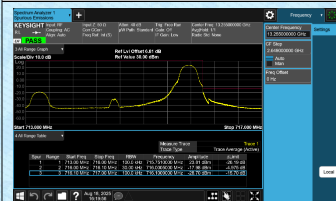
Band12-3MHz-QPSK-23165-1RB#14-PASS
