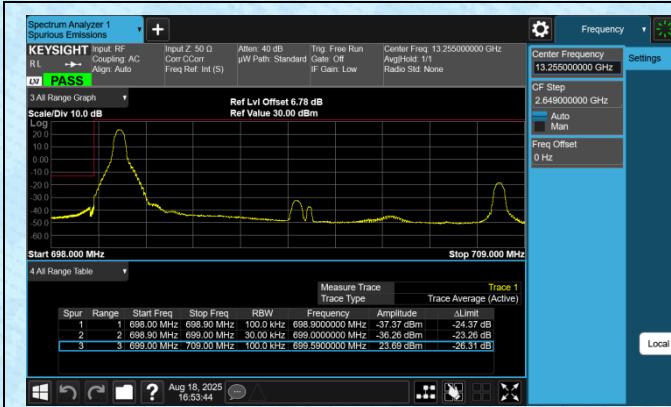
Band12-10MHz-QPSK-23060-1RB#0-PASS
