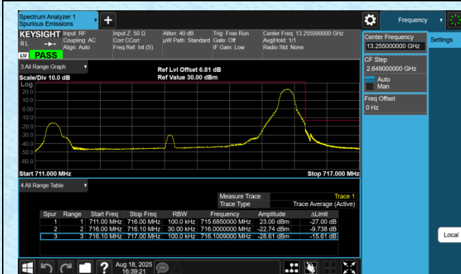
Band12-5MHz-16QAM-23155-1RB#24-PASS
