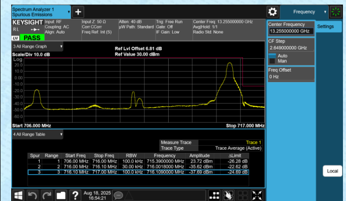
Band12-10MHz-QPSK-23130-1RB#49-PASS
