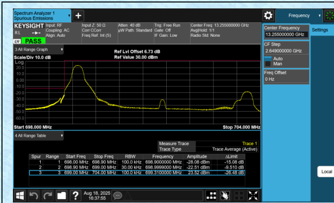
Band12-5MHz-QPSK-23035-1RB#0-PASS
