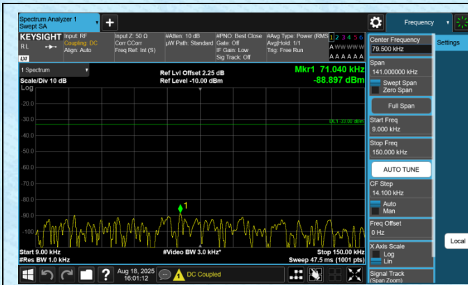
Band12-1.4MHz-QPSK-23017-1RB#0-0.009~0.15-PASS
