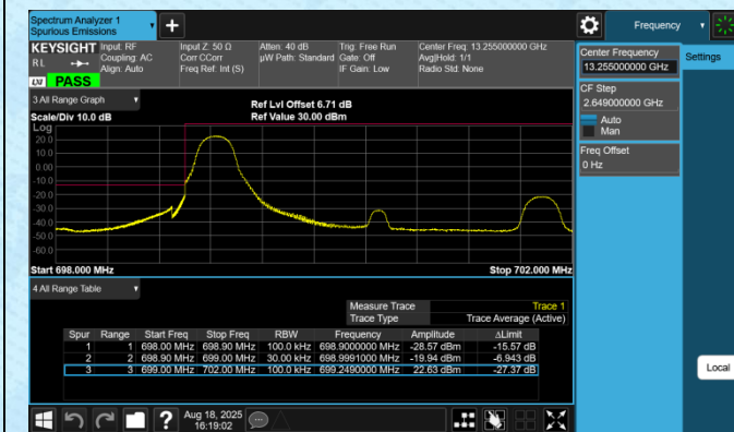
Band12-3MHz-16QAM-23025-1RB#0-PASS
