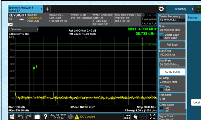
Band12-1.4MHz-QPSK-23095-1RB#0-0.15~30-PASS
