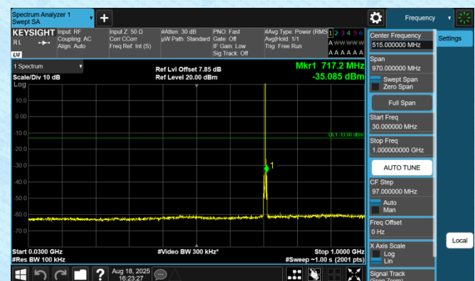
Band12-3MHz-QPSK-23165-1RB#0-30~1000-PASS
