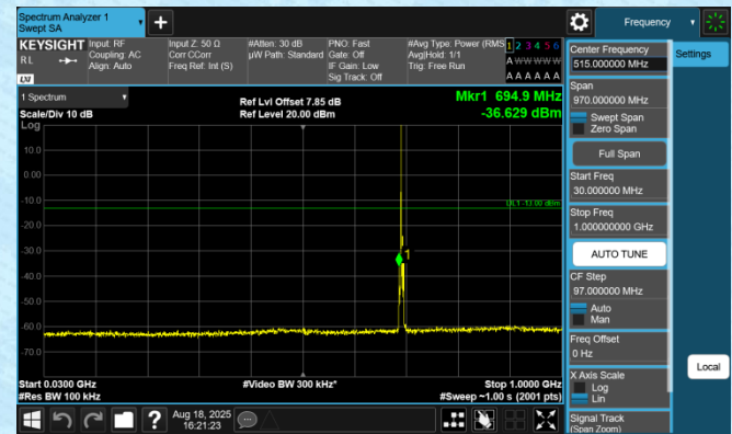
Band12-3MHz-QPSK-23025-1RB#0-30~1000-PASS
