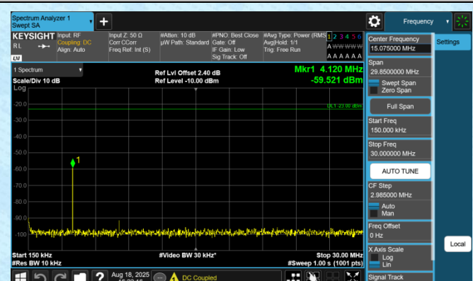
Band12-3MHz-QPSK-23095-1RB#0-0.15~30-PASS
