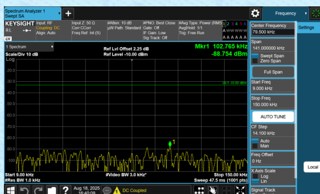
Band12-5MHz-QPSK-23035-1RB#0-0.009~0.15-PASS
