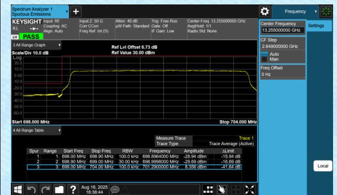
Band12-5MHz-16QAM-23035-25RB#0-PASS
