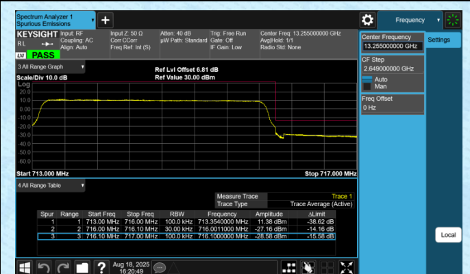
Band12-3MHz-16QAM-23165-15RB#0-PASS
