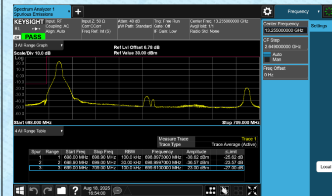
Band12-10MHz-16QAM-23060-1RB#0-PASS
