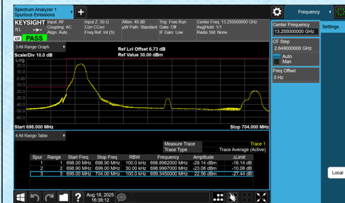
Band12-5MHz-16QAM-23035-1RB#0-PASS
