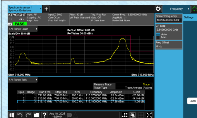
Band12-5MHz-QPSK-23155-1RB#24-PASS
