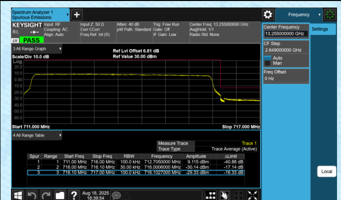
Band12-5MHz-16QAM-23155-25RB#0-PASS
