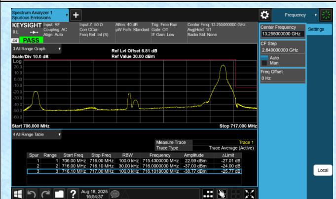
Band12-10MHz-16QAM-23130-1RB#49-PASS
