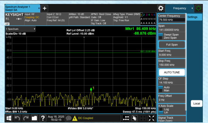
Band12-1.4MHz-QPSK-23095-1RB#0-0.009~0.15-PASS
