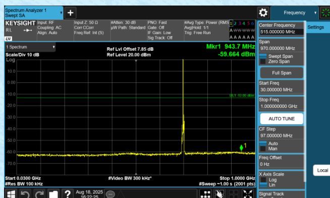
Band12-3MHz-QPSK-23095-1RB#0-30~1000-PASS
