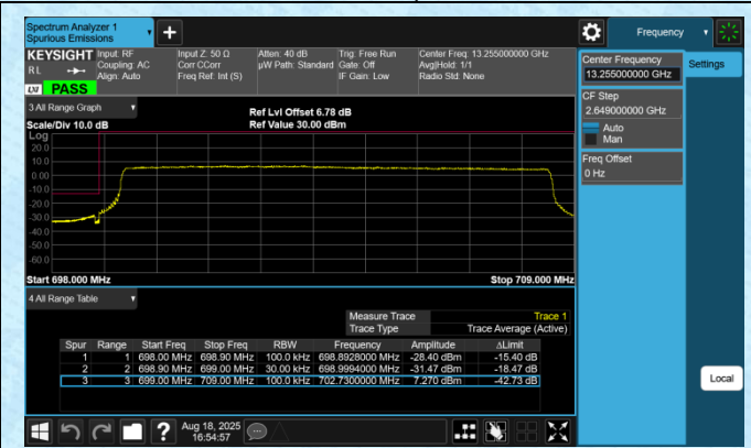
Band12-10MHz-QPSK-23060-50RB#0-PASS
