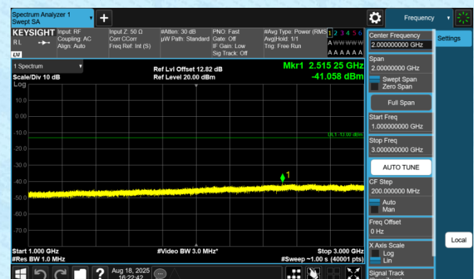
Band12-3MHz-QPSK-23095-1RB#0-1000~3000-PASS
