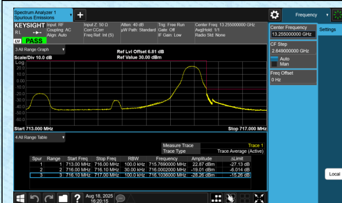
Band12-3MHz-16QAM-23165-1RB#14-PASS
