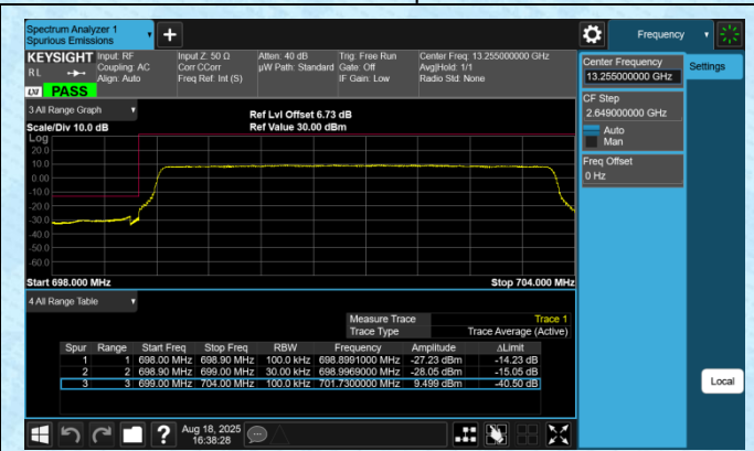
Band12-5MHz-QPSK-23035-25RB#0-PASS
