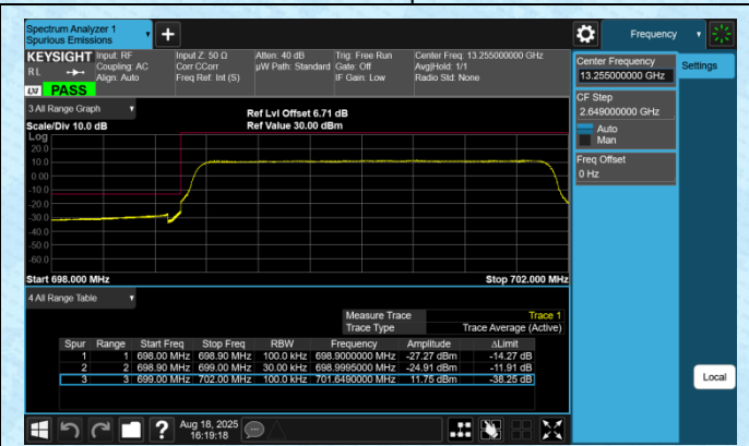
Band12-3MHz-QPSK-23025-15RB#0-PASS
