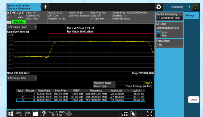
Band12-3MHz-16QAM-23025-15RB#0-PASS
