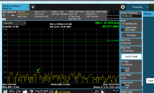
Band12-3MHz-QPSK-23095-1RB#0-0.009~0.15-PASS
