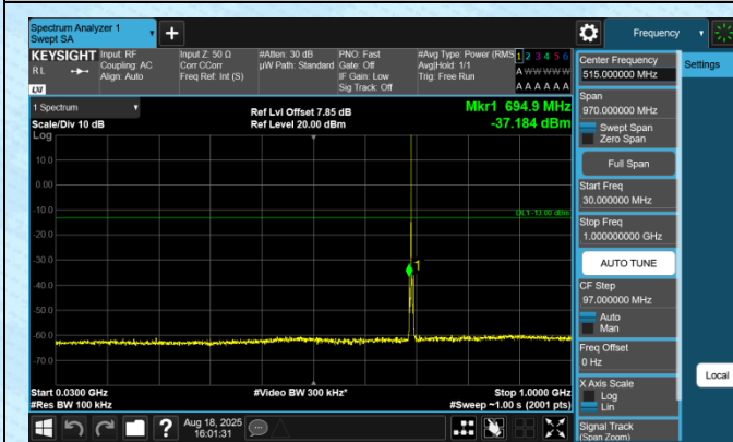
Band12-1.4MHz-QPSK-23017-1RB#0-30~1000-PASS
