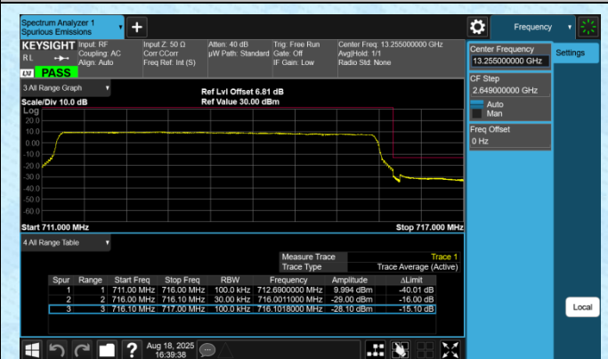
Band12-5MHz-QPSK-23155-25RB#0-PASS
