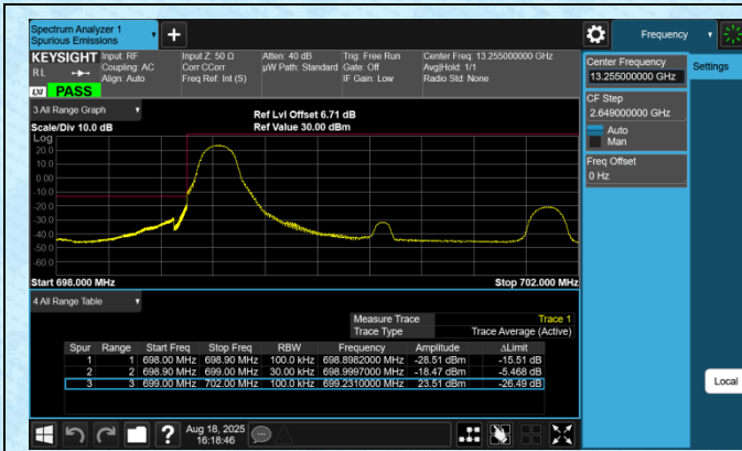
Band12-3MHz-QPSK-23025-1RB#0-PASS
