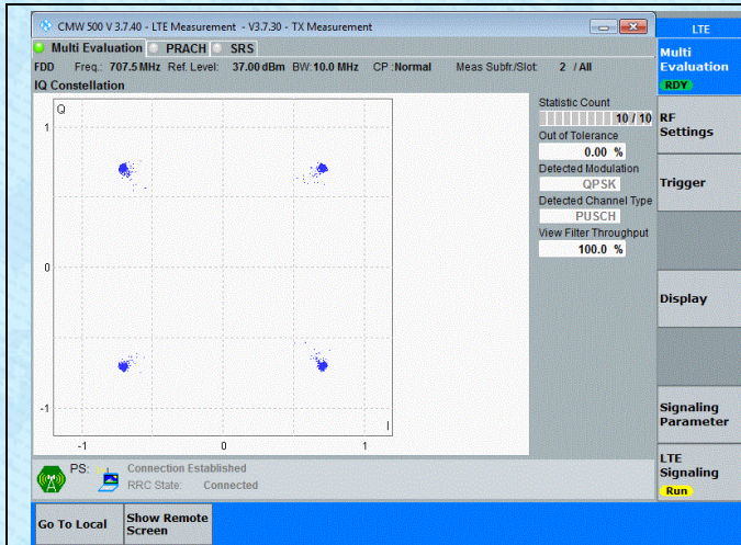
Band12-10MHz-QPSK-23095-50RB#0-PASS
