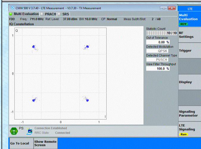
Band12-10MHz-QPSK-23130-50RB#0-PASS
