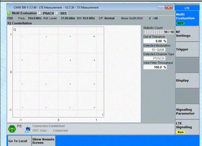
Band12-10MHz-16QAM-23060-1RB#0-PASS
