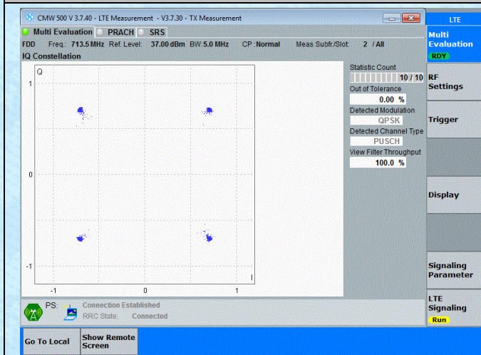
Band12-5MHz-QPSK-23155-25RB#0-PASS
