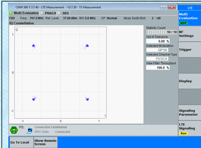
Band12-5MHz-QPSK-23095-25RB#0-PASS
