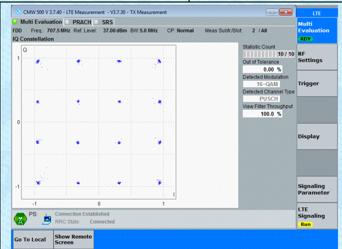
Band12-5MHz-16QAM-23095-25RB#0-PASS
