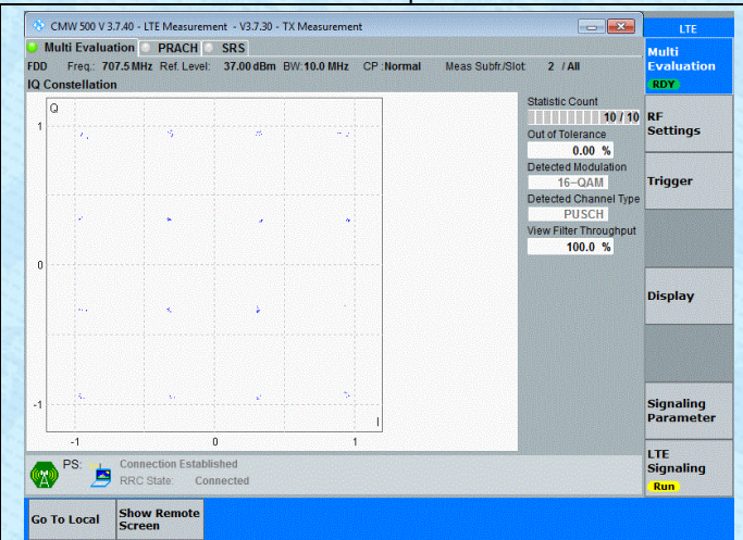
Band12-10MHz-16QAM-23095-1RB#0-PASS
