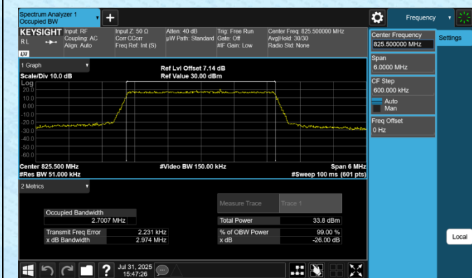
Band5-3MHz-QPSK-20415-15RB#0-PASS
