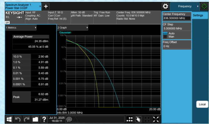
Band5-3MHz-16QAM-20525-15RB#0-PASS
