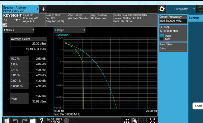
Band5-3MHz-QPSK-20525-1RB#0-PASS
