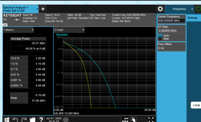
Band5-10MHz-16QAM-20525-1RB#0-PASS
