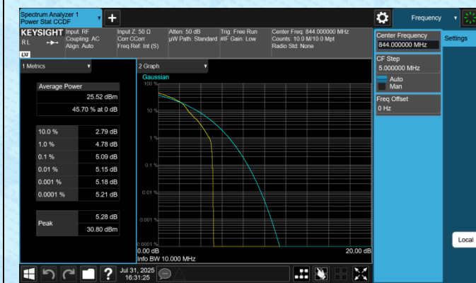
Band5-10MHz-16QAM-20600-1RB#0-PASS
