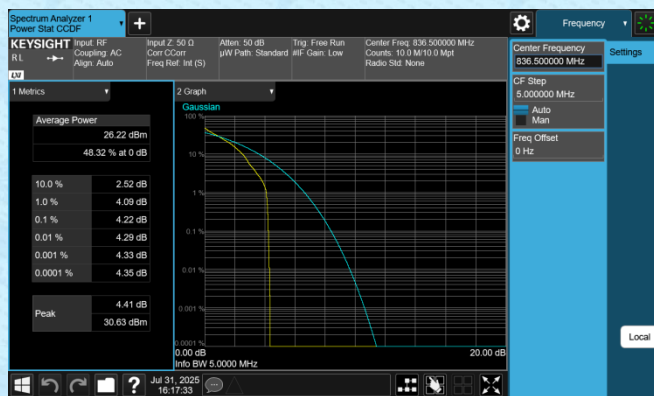
Band5-5MHz-QPSK-20525-1RB#0-PASS
