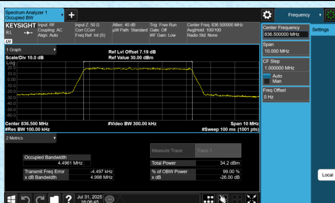
Band5-5MHz-QPSK-20525-25RB#0-PASS
