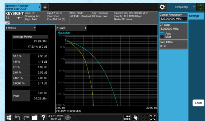
Band5-10MHz-QPSK-20450-50RB#0-PASS
