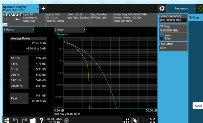
Band5-1.4MHz-16QAM-20525-1RB#0-PASS
