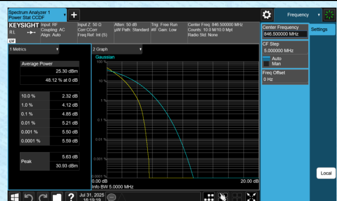
Band5-5MHz-QPSK-20625-25RB#0-PASS
