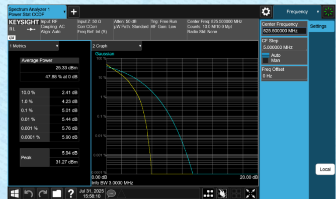
Band5-3MHz-QPSK-20415-15RB#0-PASS
