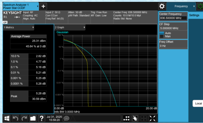
Band5-3MHz-16QAM-20525-1RB#0-PASS
