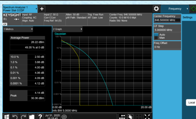
Band5-5MHz-QPSK-20625-1RB#0-PASS
