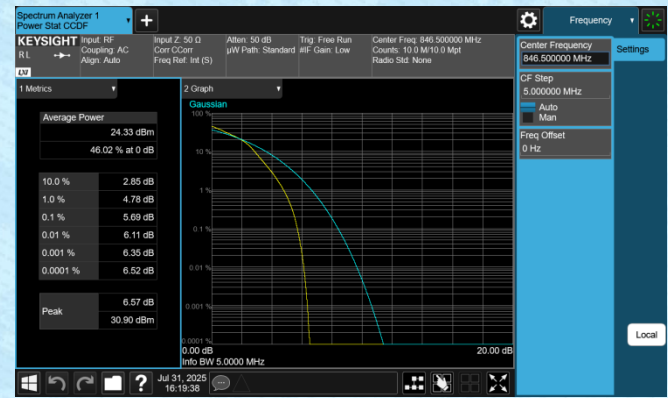
Band5-5MHz-16QAM-20625-25RB#0-PASS
