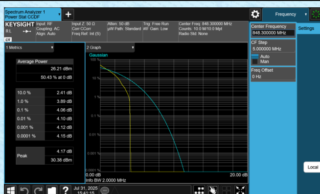
Band5-1.4MHz-QPSK-20643-1RB#0-PASS
