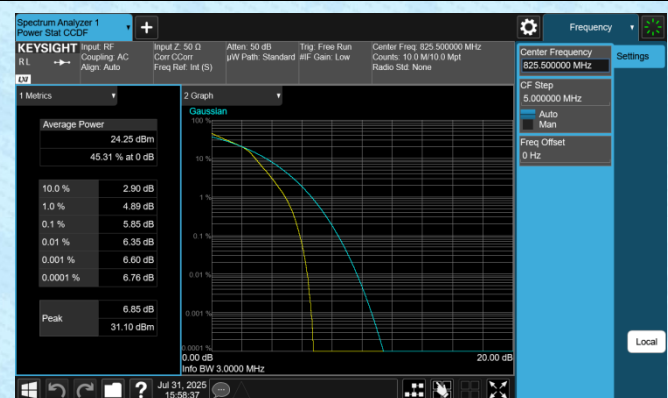
Band5-3MHz-16QAM-20415-15RB#0-PASS
