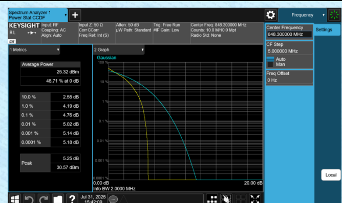
Band5-1.4MHz-QPSK-20643-6RB#0-PASS
