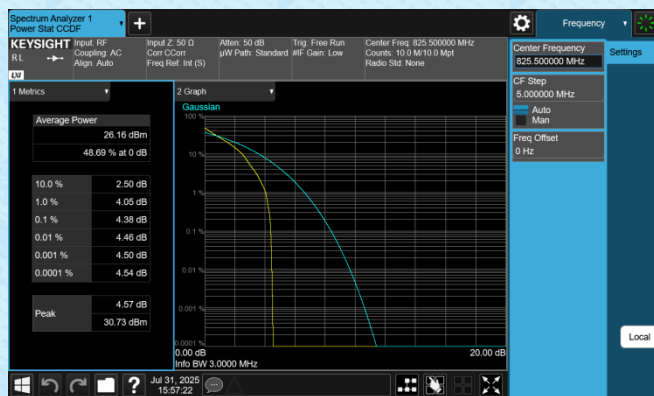
Band5-3MHz-QPSK-20415-1RB#0-PASS
