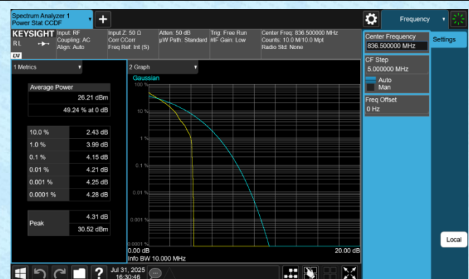
Band5-10MHz-QPSK-20525-1RB#0-PASS
