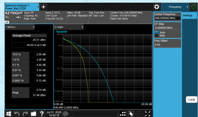
Band5-1.4MHz-QPSK-20525-6RB#0-PASS
