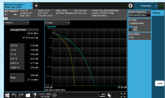
Band5-5MHz-QPSK-20525-25RB#0-PASS
