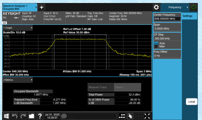
Band5-1.4MHz-16QAM-20643-6RB#0-PASS
