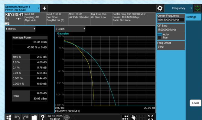
Band5-1.4MHz-16QAM-20525-6RB#0-PASS
