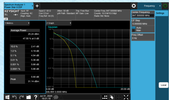
Band5-3MHz-QPSK-20635-15RB#0-PASS
