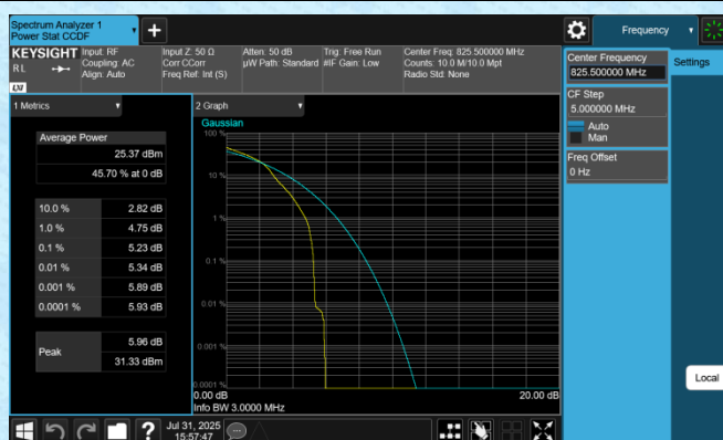
Band5-3MHz-16QAM-20415-1RB#0-PASS
