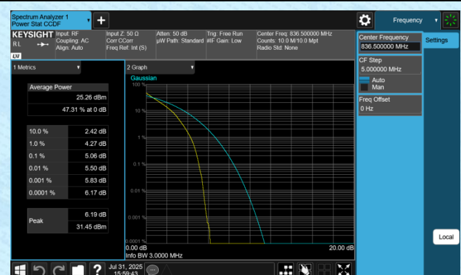
Band5-3MHz-QPSK-20525-15RB#0-PASS
