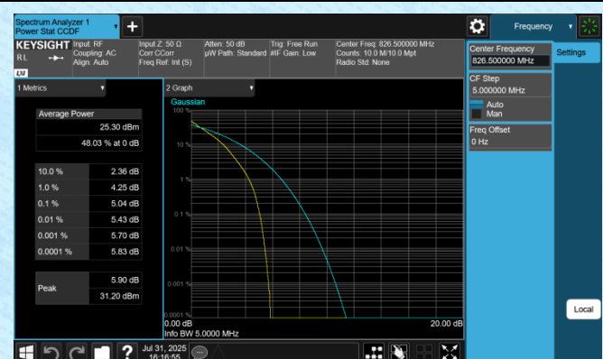
Band5-5MHz-QPSK-20425-25RB#0-PASS
