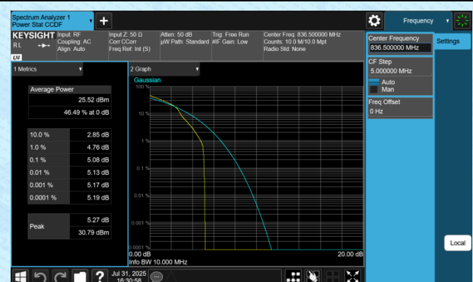
Band5-10MHz-QPSK-20525-50RB#0-PASS
