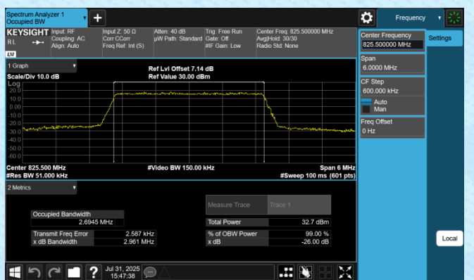
Band5-3MHz-16QAM-20415-15RB#0-PASS
