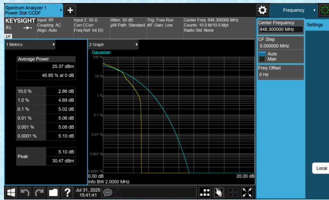
Band5-1.4MHz-16QAM-20643-1RB#0-PASS
