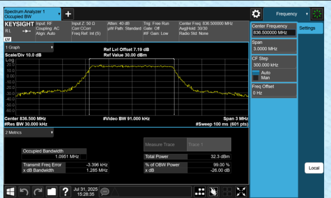
Band5-1.4MHz-16QAM-20525-6RB#0-PASS
