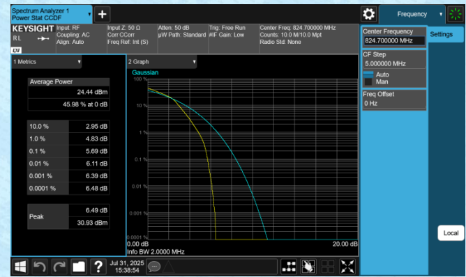
Band5-1.4MHz-16QAM-20407-6RB#0-PASS
