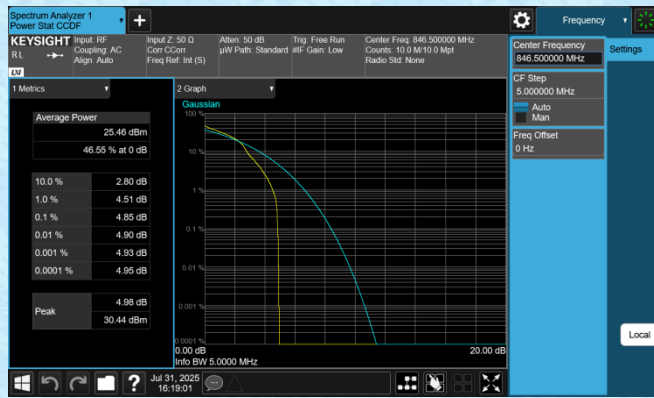
Band5-5MHz-16QAM-20625-1RB#0-PASS
