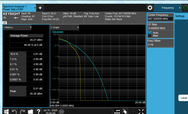
Band5-3MHz-16QAM-20635-1RB#0-PASS
