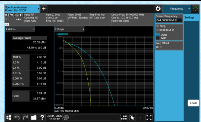
Band5-10MHz-QPSK-20600-50RB#0-PASS
