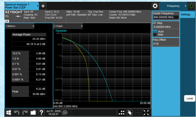
Band5-1.4MHz-16QAM-20643-6RB#0-PASS
