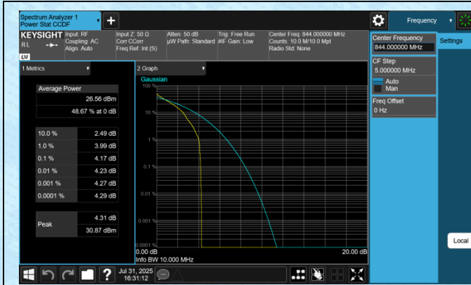
Band5-10MHz-QPSK-20600-1RB#0-PASS
