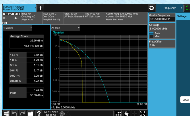
Band5-5MHz-16QAM-20525-1RB#0-PASS
