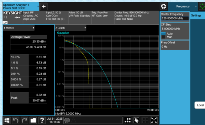
Band5-5MHz-16QAM-20425-1RB#0-PASS
