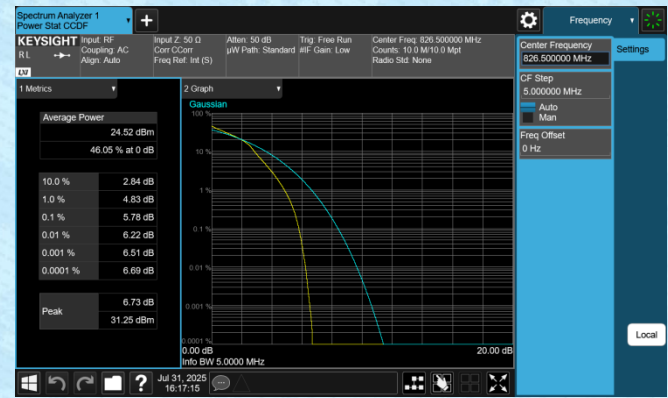
Band5-5MHz-16QAM-20425-25RB#0-PASS
