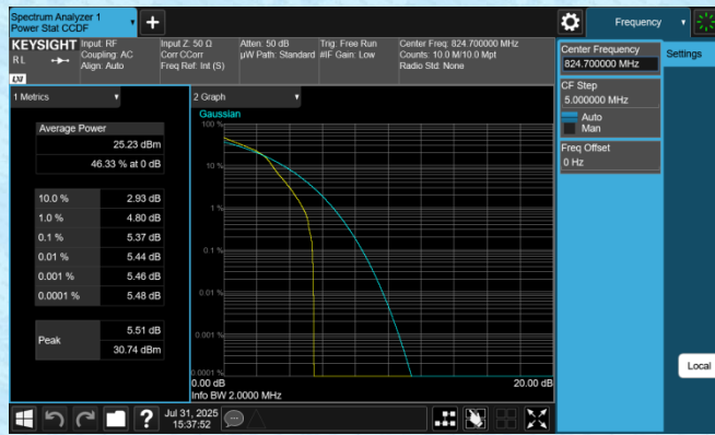
Band5-1.4MHz-16QAM-20407-1RB#0-PASS
