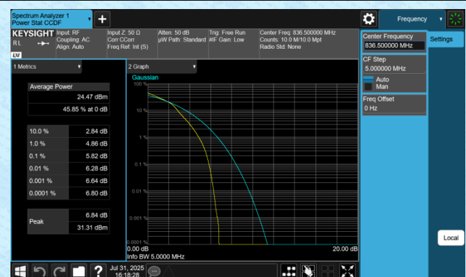
Band5-5MHz-16QAM-20525-25RB#0-PASS
