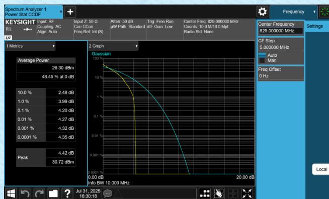
Band5-10MHz-QPSK-20450-1RB#0-PASS
