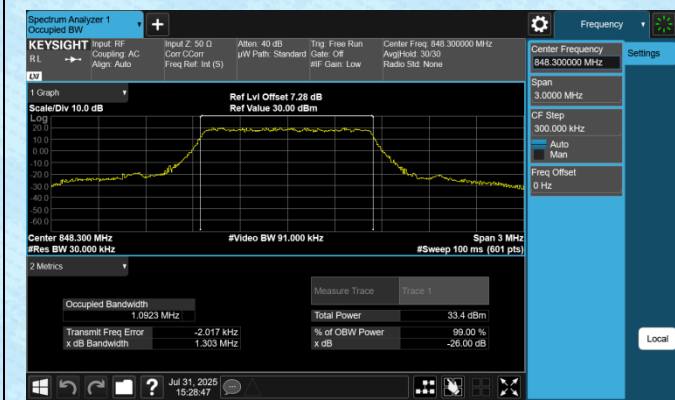
Band5-1.4MHz-QPSK-20643-6RB#0-PASS
