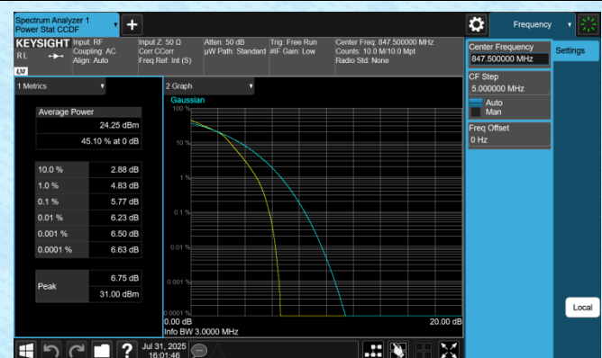
Band5-3MHz-16QAM-20635-15RB#0-PASS
