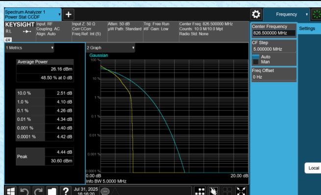
Band5-5MHz-QPSK-20425-1RB#0-PASS
