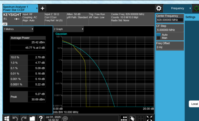
Band5-10MHz-16QAM-20450-1RB#0-PASS
