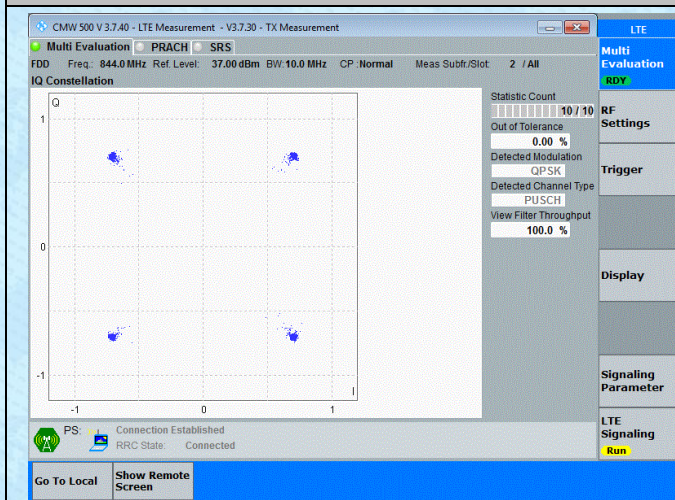
Band5-10MHz-QPSK-20600-50RB#0-PASS
