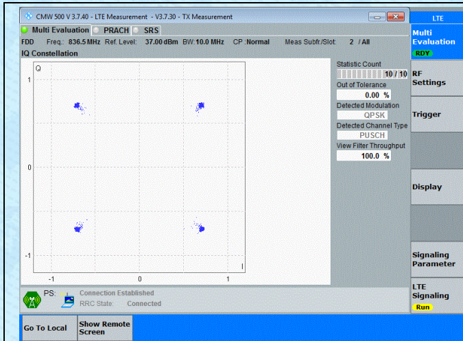
Band5-10MHz-QPSK-20525-50RB#0-PASS
