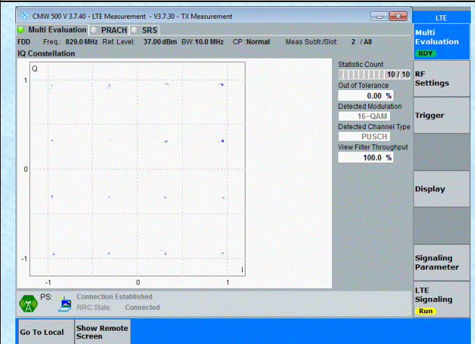
Band5-10MHz-16QAM-20450-1RB#0-PASS
