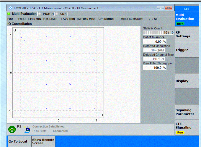
Band5-10MHz-16QAM-20600-1RB#0-PASS
