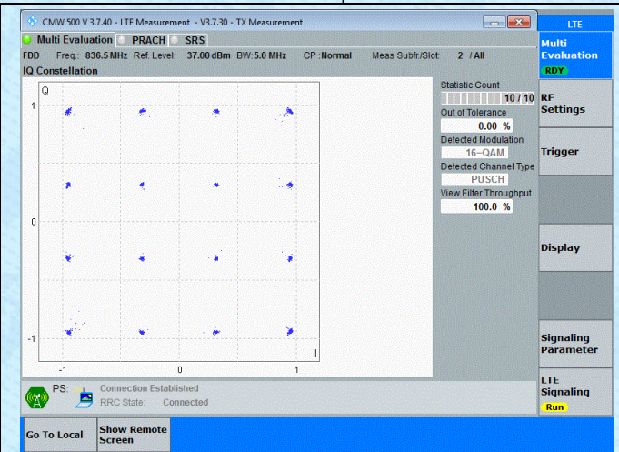
Band5-5MHz-16QAM-20525-25RB#0-PASS
