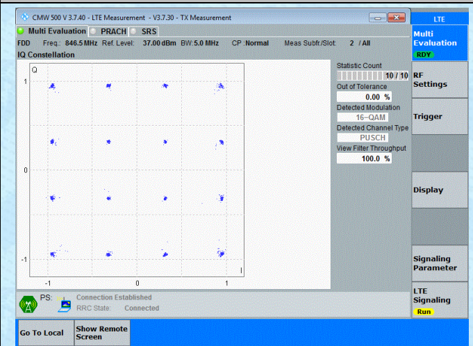
Band5-5MHz-16QAM-20625-25RB#0-PASS
