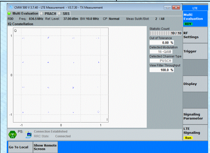
Band5-10MHz-16QAM-20525-1RB#0-PASS
