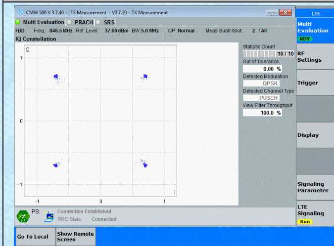
Band5-5MHz-QPSK-20625-25RB#0-PASS
