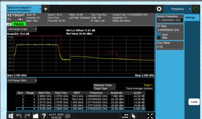
Band7-5MHz-16QAM-21425-25RB#0-PASS
