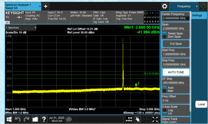
Band7-5MHz-QPSK-20775-1RB#0-1000~3000-PASS
