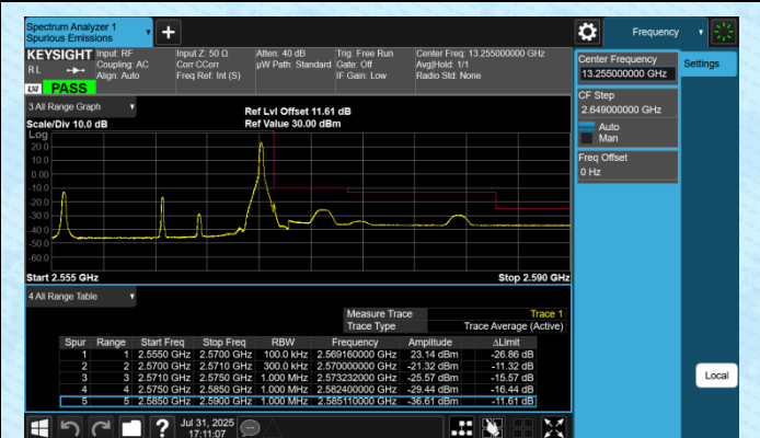
Band7-15MHz-QPSK-21375-1RB#74-PASS
