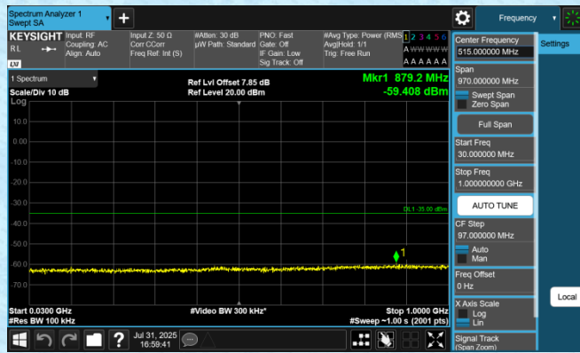
Band7-10MHz-QPSK-21100-1RB#0-30~1000-PASS
