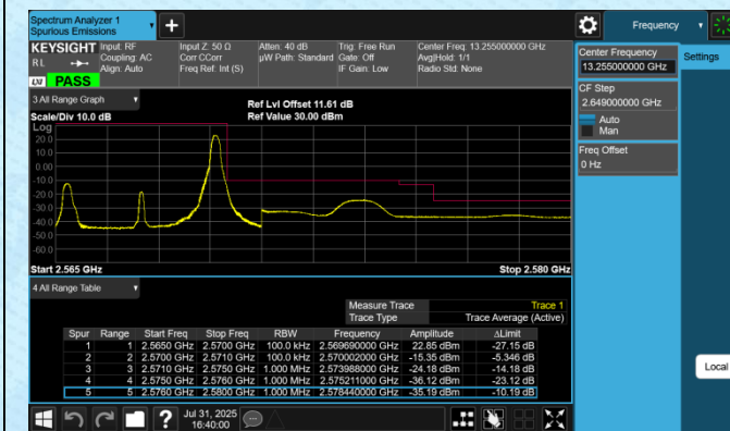
Band7-5MHz-QPSK-21425-1RB#24-PASS
