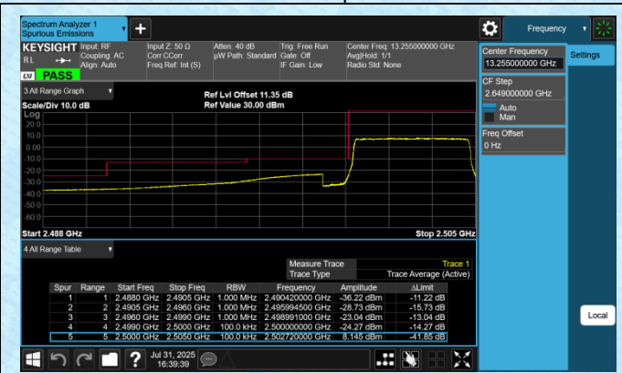
Band7-5MHz-16QAM-20775-25RB#0-PASS
