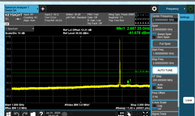
Band7-5MHz-QPSK-21425-1RB#0-1000~3000-PASS
