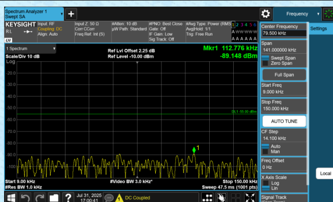
Band7-10MHz-QPSK-21400-1RB#0-0.009~0.15-PASS
