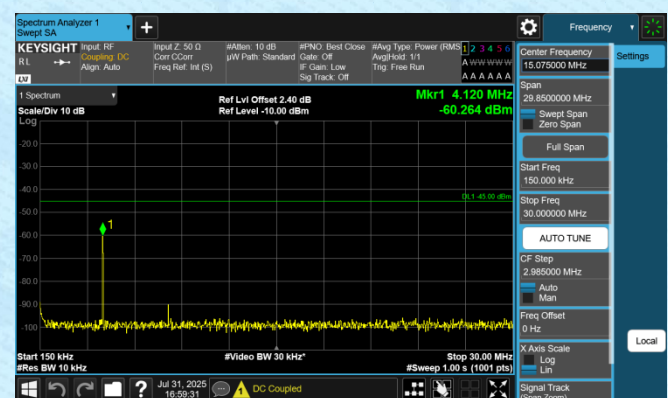
Band7-10MHz-QPSK-21100-1RB#0-0.15~30-PASS
