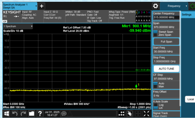
Band7-5MHz-QPSK-20775-1RB#0-30~1000-PASS
