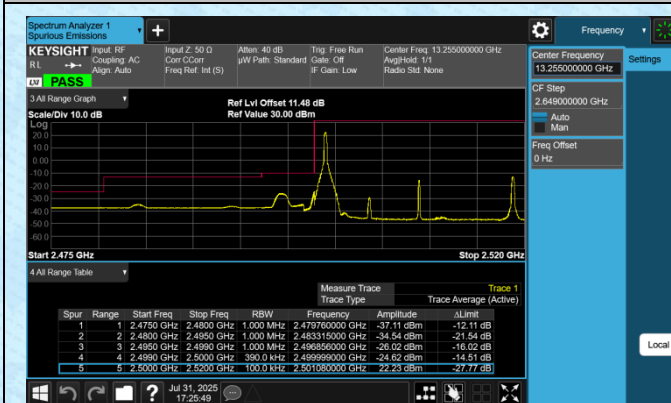
Band7-20MHz-16QAM-20850-1RB#0-PASS
