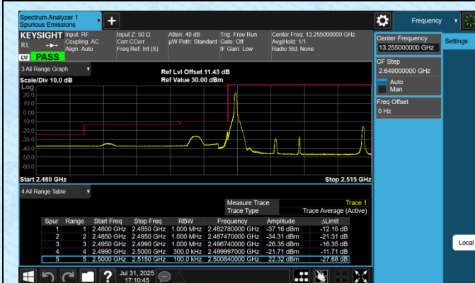
Band7-15MHz-16QAM-20825-1RB#0-PASS
