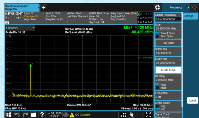
Band7-5MHz-QPSK-21425-1RB#0-0.15~30-PASS
