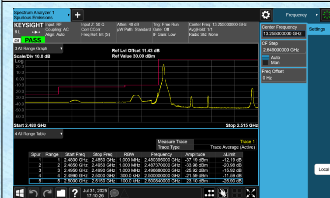
Band7-15MHz-QPSK-20825-1RB#0-PASS
