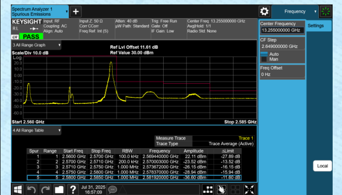
Band7-10MHz-16QAM-21400-1RB#49-PASS
