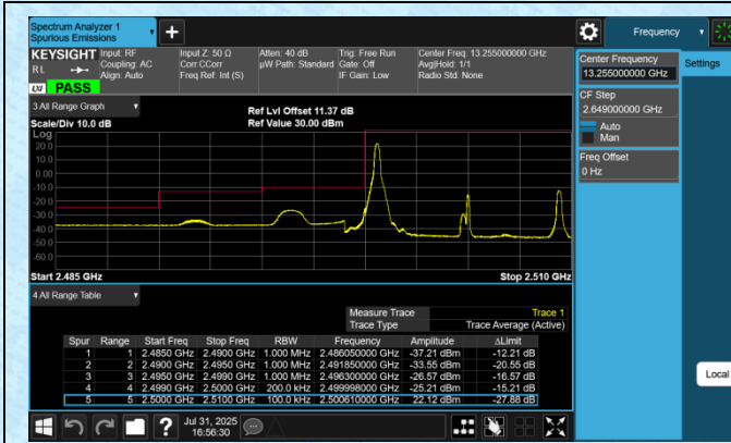
Band7-10MHz-16QAM-20800-1RB#0-PASS
