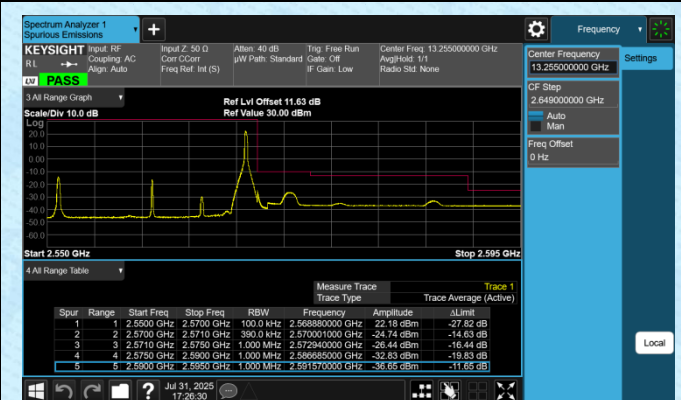
Band7-20MHz-16QAM-21350-1RB#99-PASS
