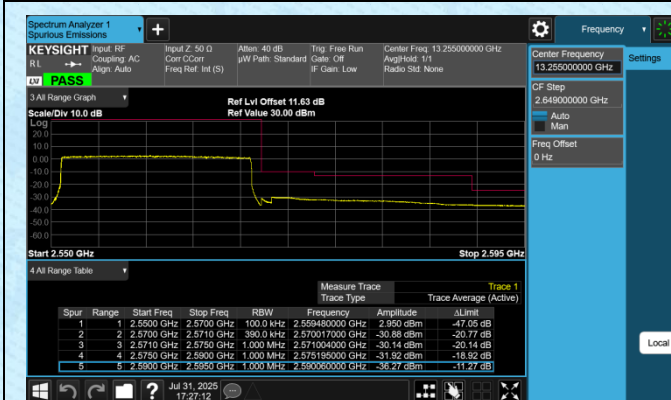
Band7-20MHz-QPSK-21350-100RB#0-PASS
