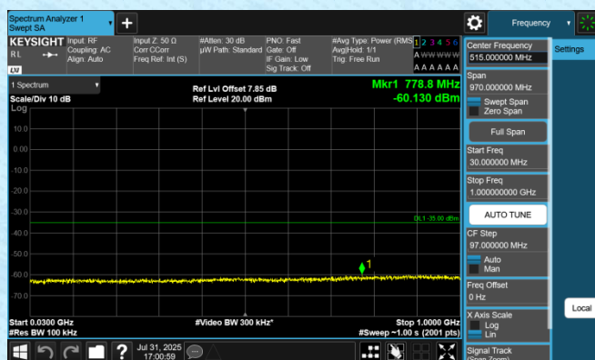
Band7-10MHz-QPSK-21400-1RB#0-30~1000-PASS
