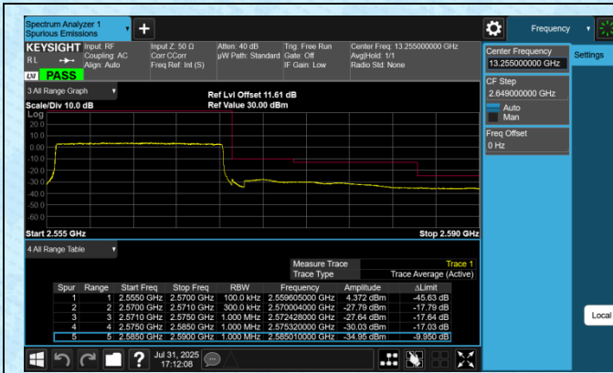
Band7-15MHz-QPSK-21375-75RB#0-PASS
