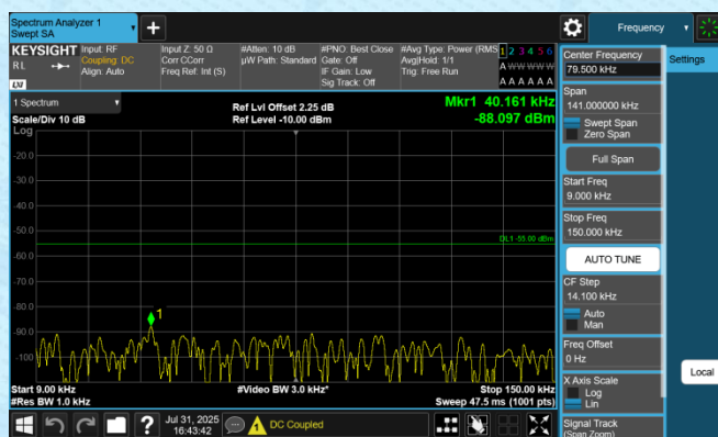
Band7-5MHz-QPSK-21425-1RB#0-0.009~0.15-PASS
