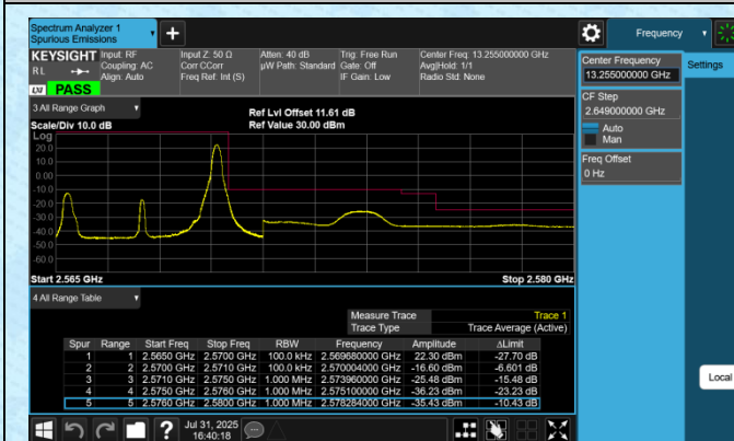
Band7-5MHz-16QAM-21425-1RB#24-PASS
