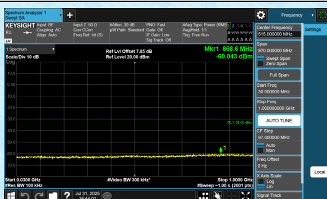
Band7-5MHz-QPSK-21425-1RB#0-30~1000-PASS
