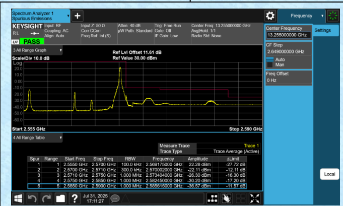
Band7-15MHz-16QAM-21375-1RB#74-PASS
