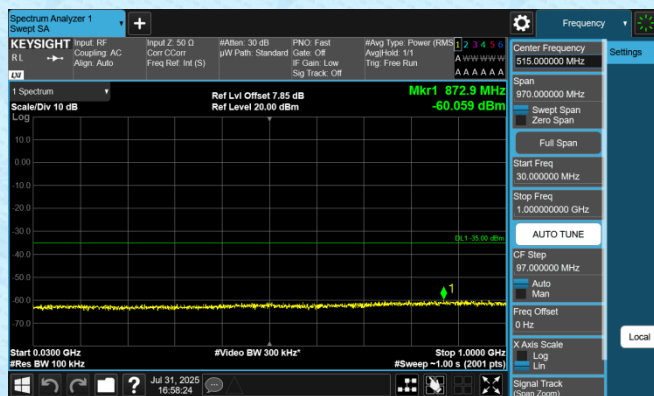
Band7-10MHz-QPSK-20800-1RB#0-30~1000-PASS
