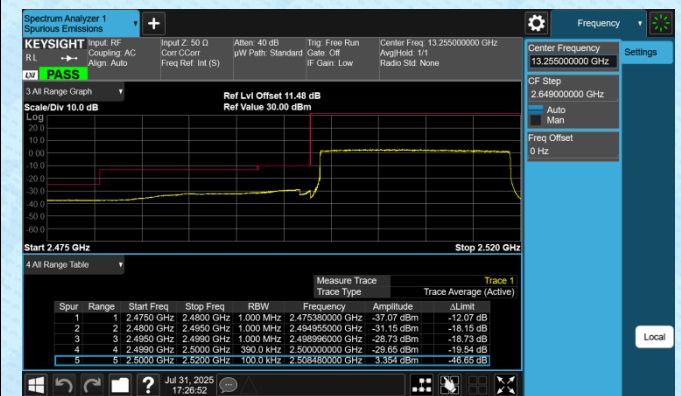
Band7-20MHz-QPSK-20850-100RB#0-PASS
