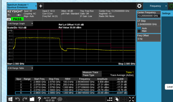
Band7-10MHz-QPSK-21400-50RB#0-PASS
