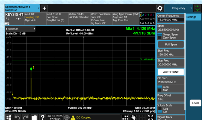
Band7-10MHz-QPSK-21400-1RB#0-0.15~30-PASS
