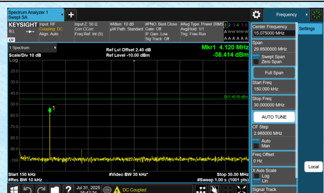
Band7-5MHz-QPSK-21100-1RB#0-0.15~30-PASS
