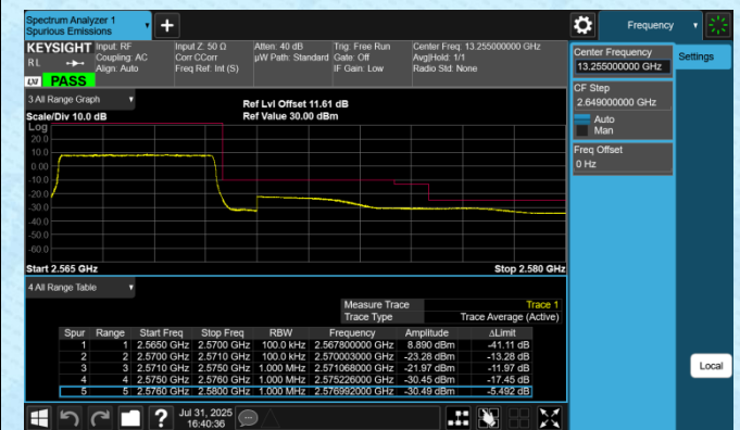
Band7-5MHz-QPSK-21425-25RB#0-PASS
