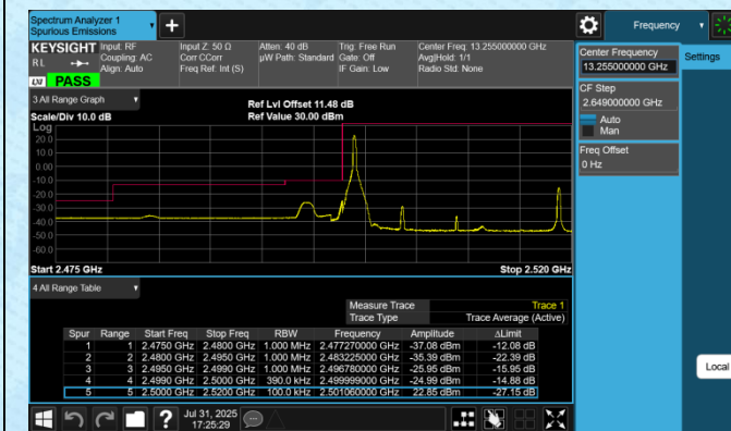
Band7-20MHz-QPSK-20850-1RB#0-PASS
