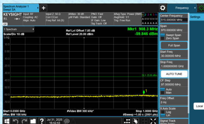
Band7-5MHz-QPSK-21100-1RB#0-30~1000-PASS
