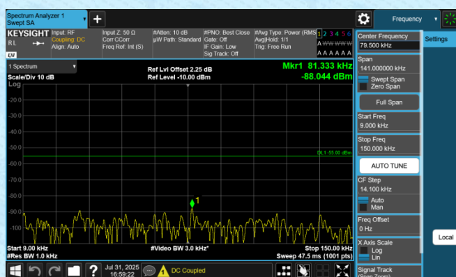
Band7-10MHz-QPSK-21100-1RB#0-0.009~0.15-PASS
