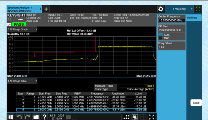
Band7-15MHz-QPSK-20825-75RB#0-PASS
