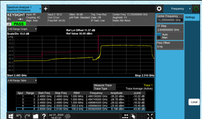
Band7-10MHz-QPSK-20800-50RB#0-PASS
