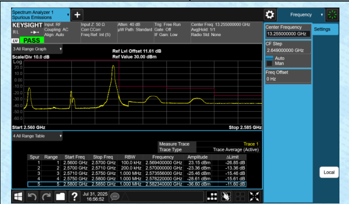
Band7-10MHz-QPSK-21400-1RB#49-PASS
