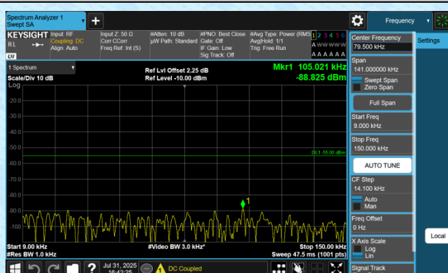
Band7-5MHz-QPSK-21100-1RB#0-0.009~0.15-PASS
