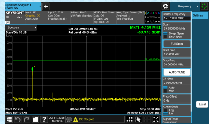
Band7-10MHz-QPSK-20800-1RB#0-0.15~30-PASS
