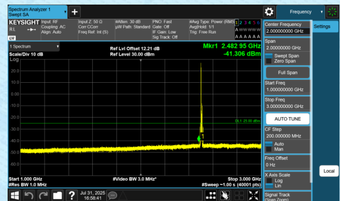
Band7-10MHz-QPSK-20800-1RB#0-1000~3000-PASS
