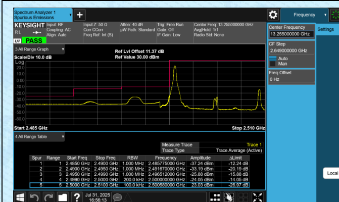
Band7-10MHz-QPSK-20800-1RB#0-PASS
