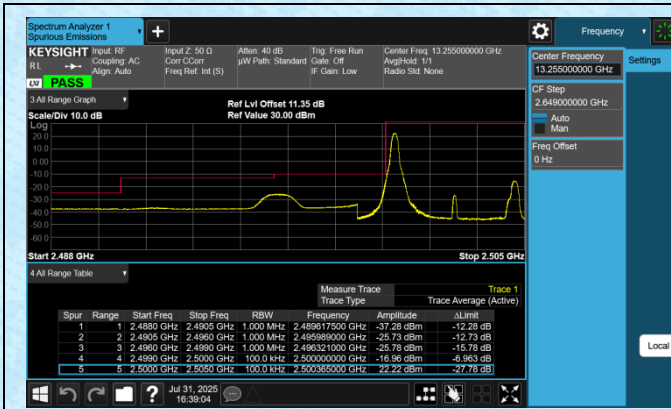
Band7-5MHz-16QAM-20775-1RB#0-PASS
