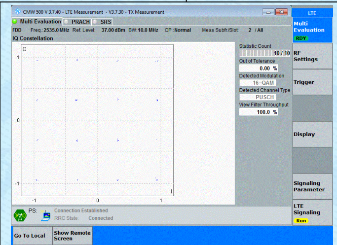
Band7-10MHz-16QAM-21100-1RB#0-PASS
