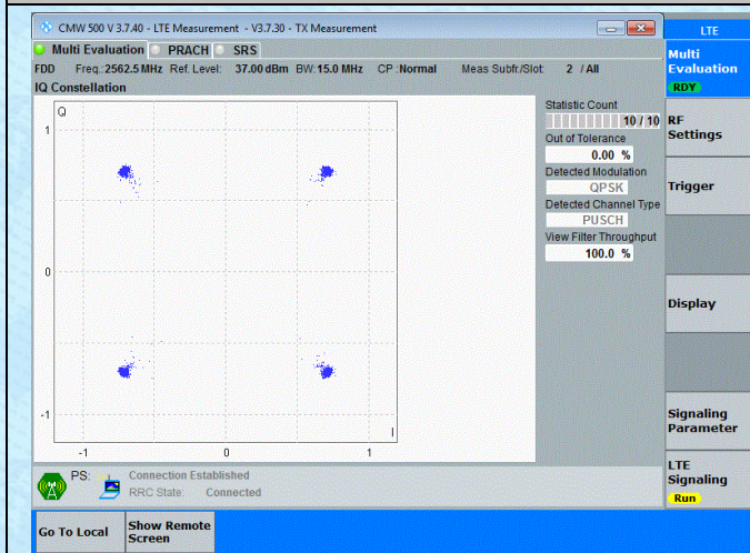
Band7-15MHz-QPSK-21375-75RB#0-PASS
