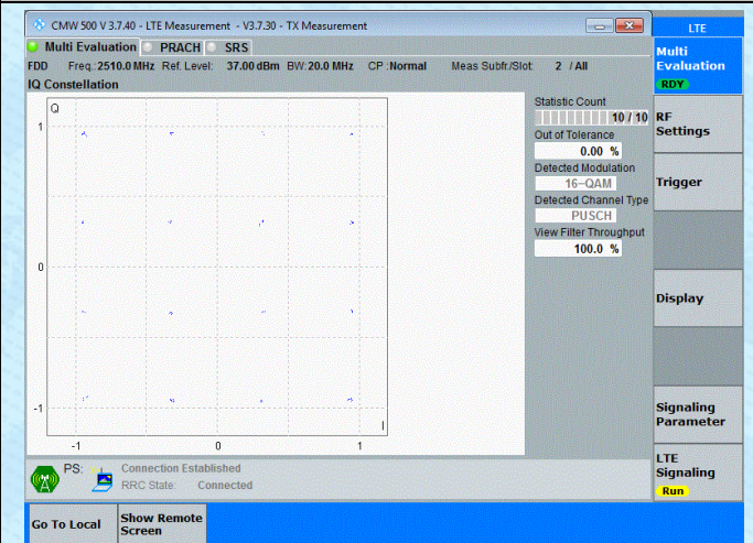
Band7-20MHz-16QAM-20850-1RB#0-PASS
