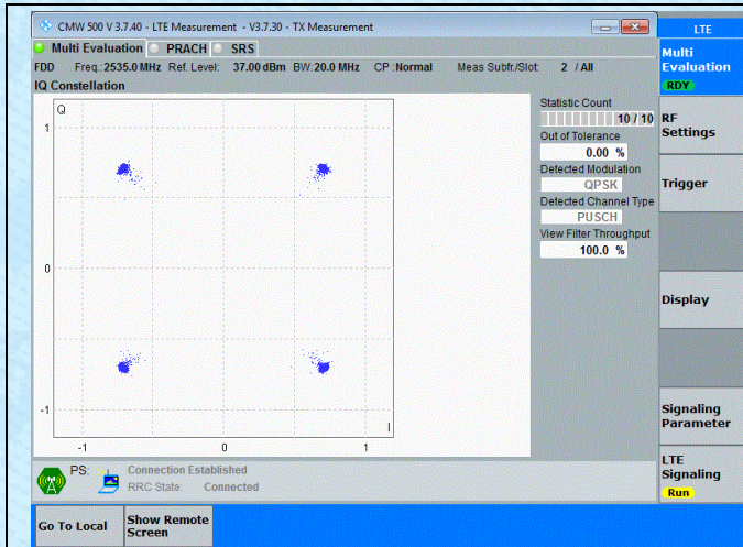
Band7-20MHz-QPSK-21100-100RB#0-PASS
