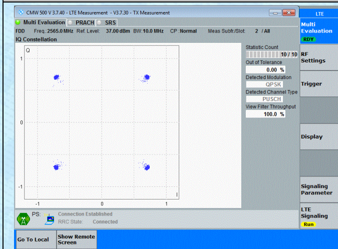
Band7-10MHz-QPSK-21400-50RB#0-PASS
