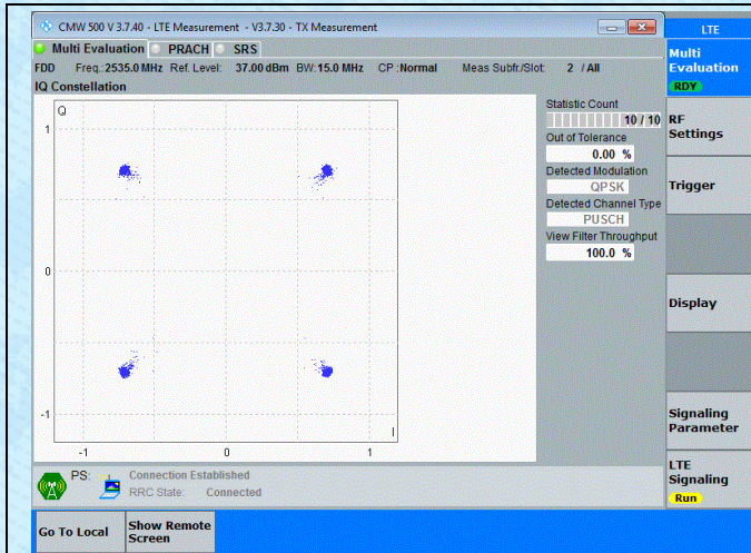
Band7-15MHz-QPSK-21100-75RB#0-PASS
