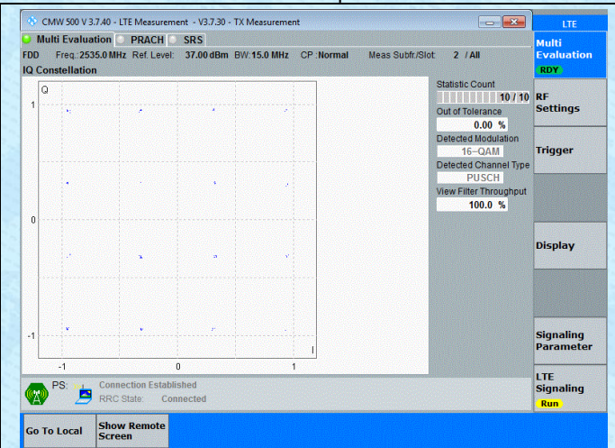
Band7-15MHz-16QAM-21100-1RB#0-PASS
