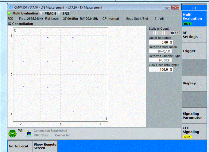
Band7-20MHz-16QAM-21100-1RB#0-PASS
