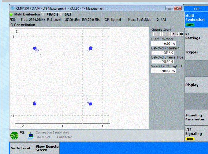
Band7-20MHz-QPSK-21350-100RB#0-PASS
