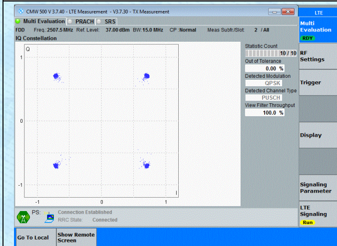
Band7-15MHz-QPSK-20825-75RB#0-PASS
