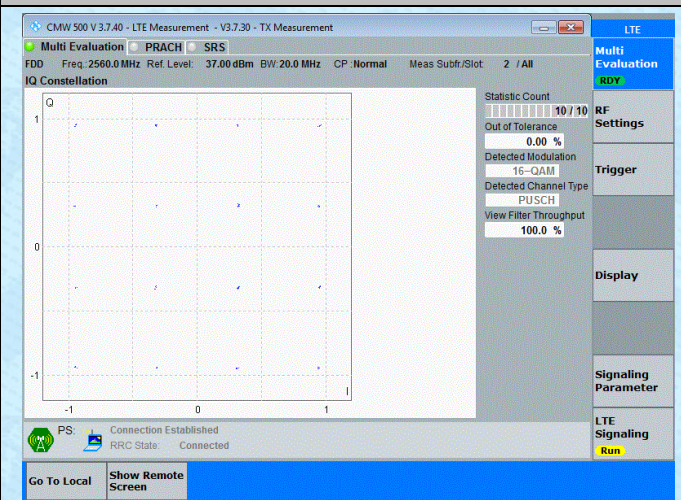
Band7-20MHz-16QAM-21350-1RB#0-PASS
