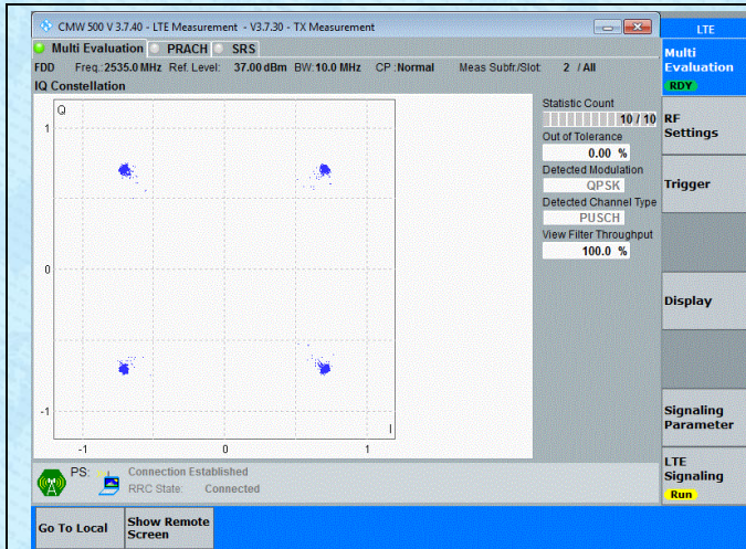
Band7-10MHz-QPSK-21100-50RB#0-PASS
