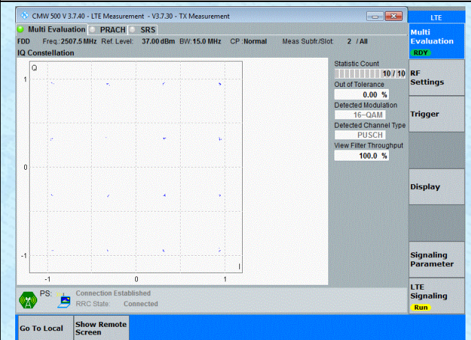
Band7-15MHz-16QAM-20825-1RB#0-PASS
