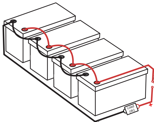
Figure 5-2 Parallel Application: 1S4P, 38.4V 400Ah
