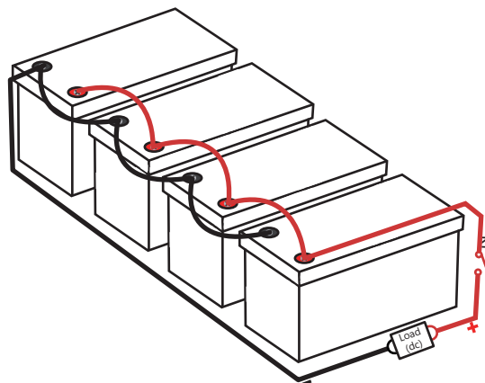
Figure 5-2 Parallel Application: 1S4P, 51.2V 400Ah
