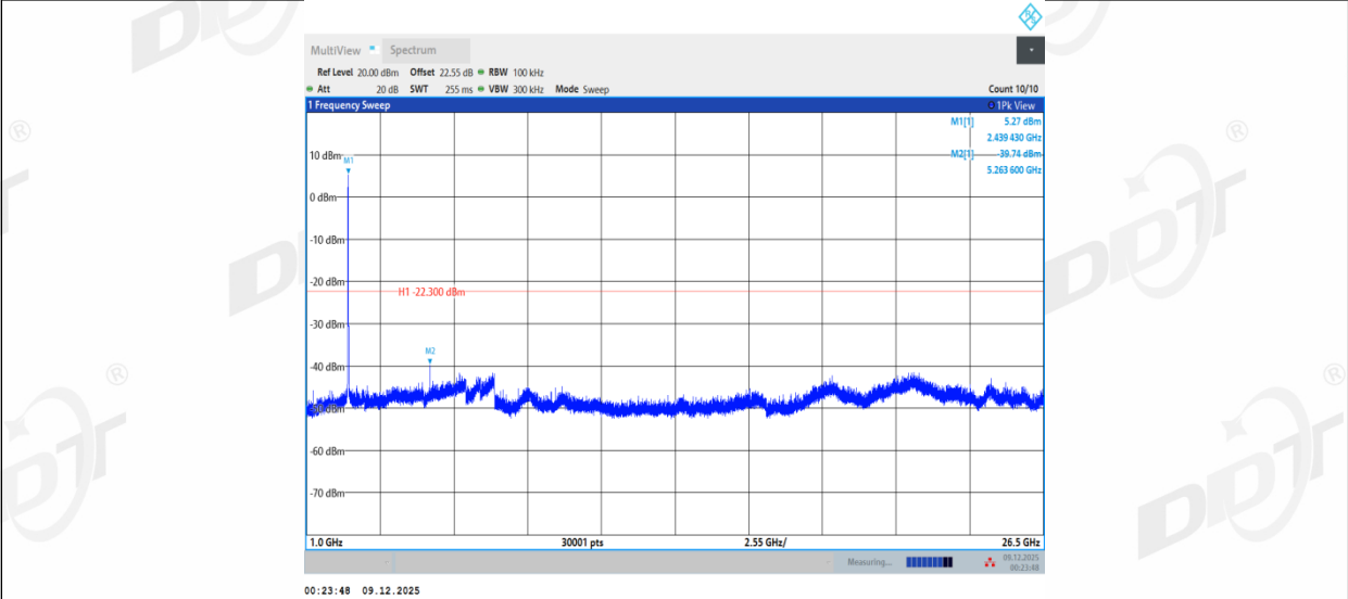
11N20SISO_Ant1_2462_0~Reference
