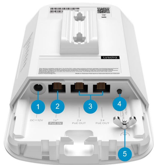
Figure 1-3 Components on the Back Panel
