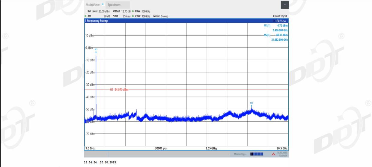
11N40SISO_Ant1_2437_0~Reference
