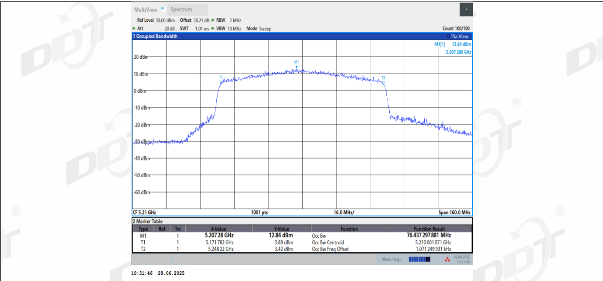
11AX80_Ant2_5210
