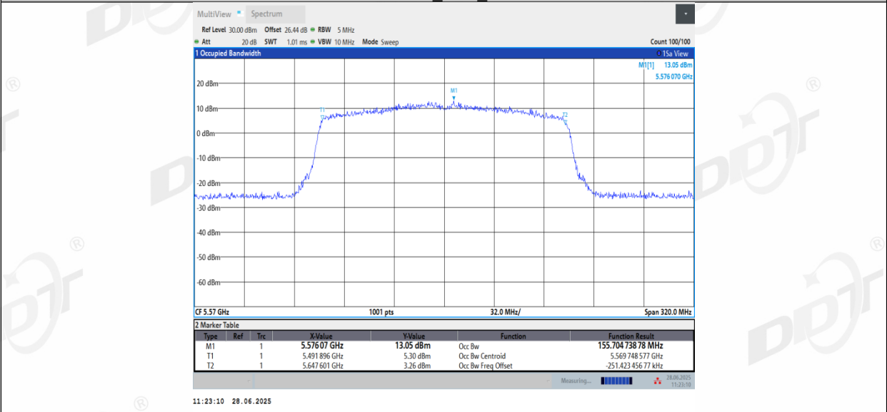
11AX160_Ant3_5570
