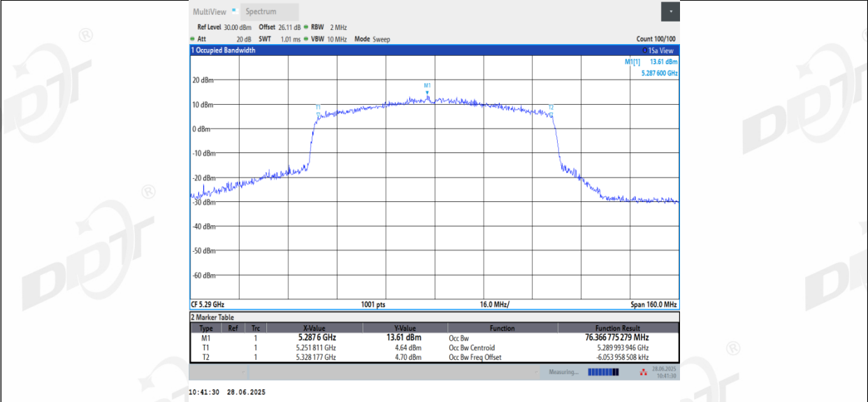
11AX80_Ant3_5290
