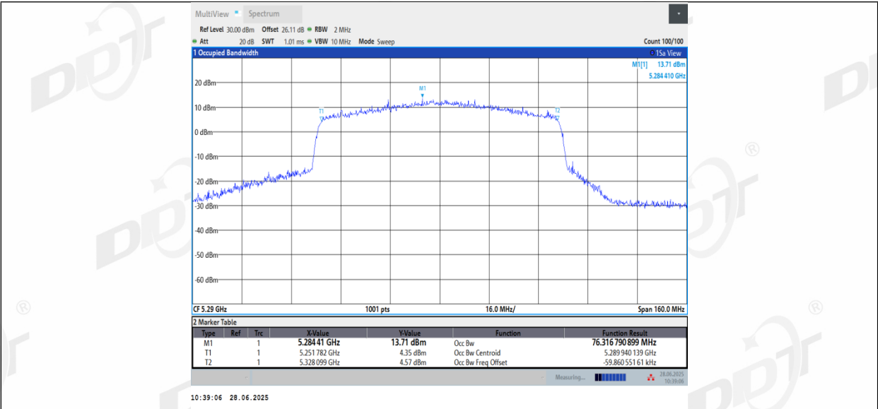
11AX80_Ant2_5290
