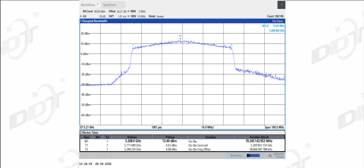
11AX80_Ant3_5210
