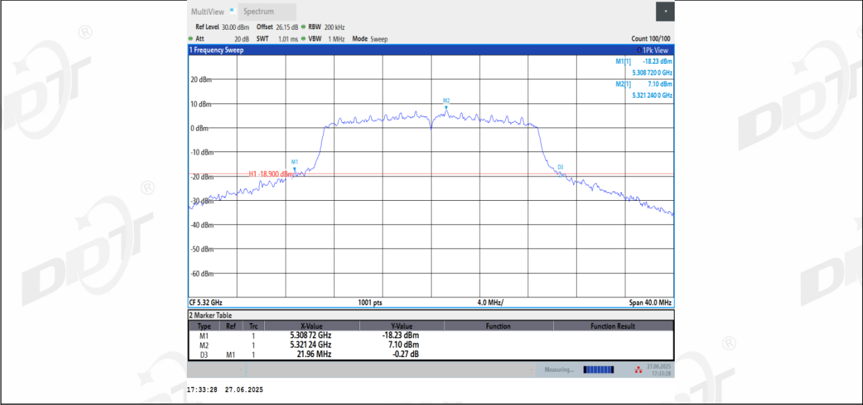
11AC20_Ant3_5320
