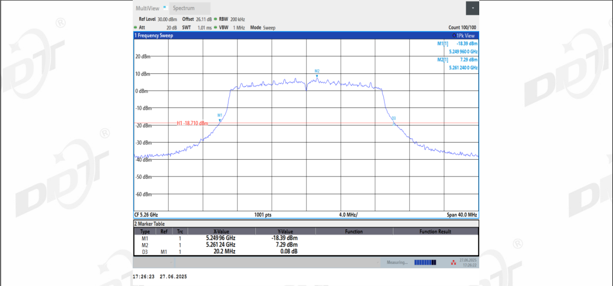
11AC20_Ant3_5260
