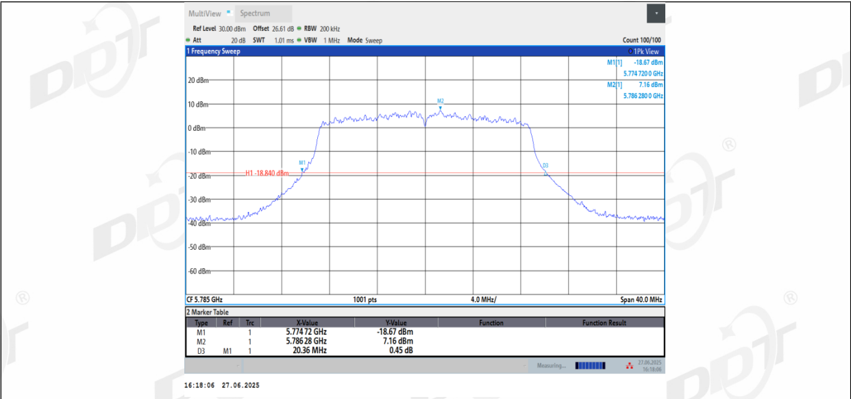
11N20_Ant2_5785
