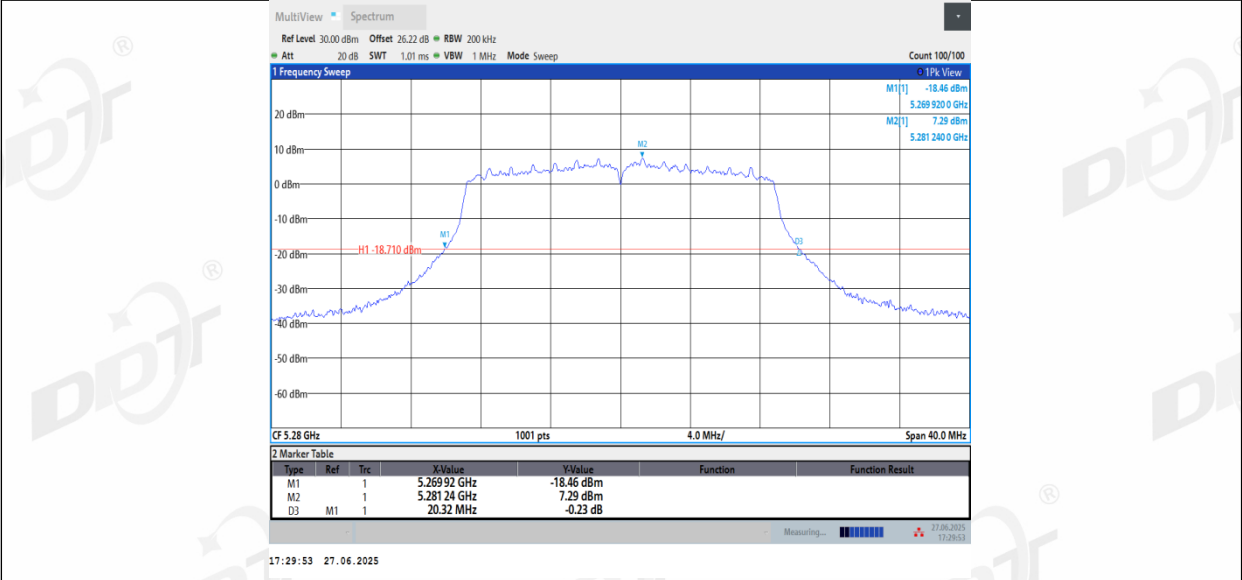
11AC20_Ant3_5280
