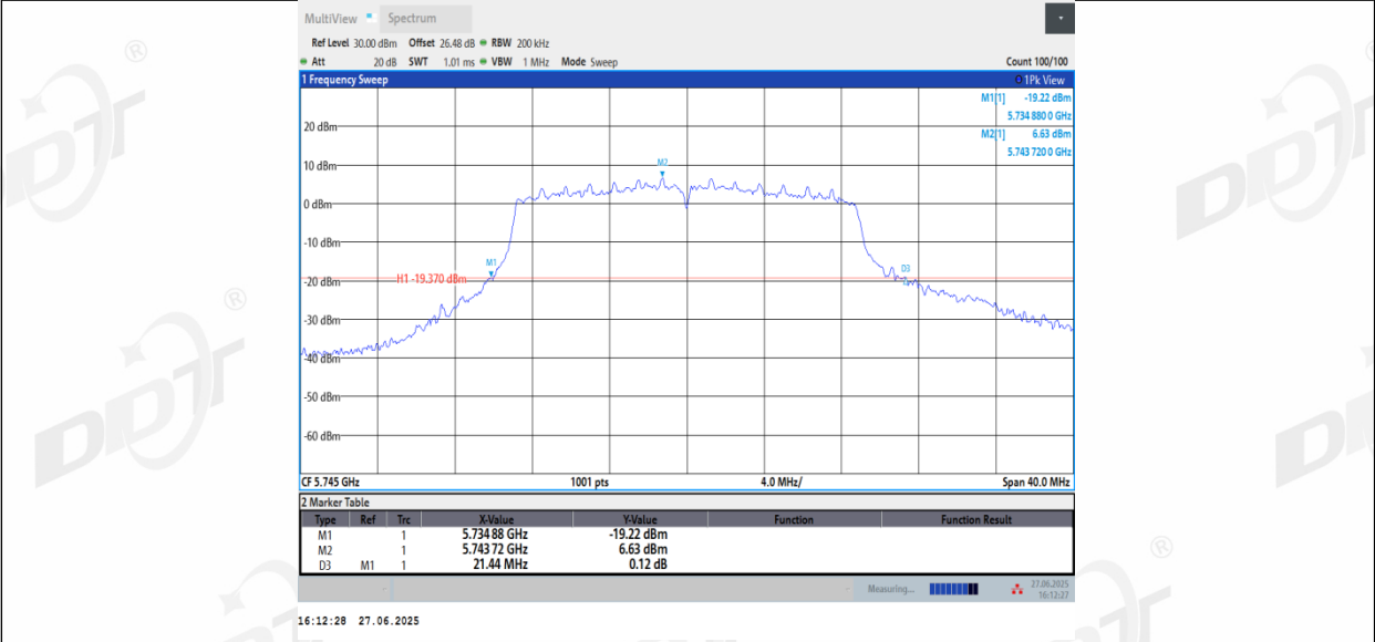
11N20_Ant3_5745
