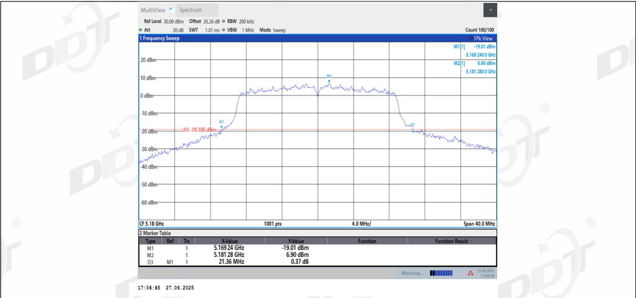
11AC20_Ant2_5180
