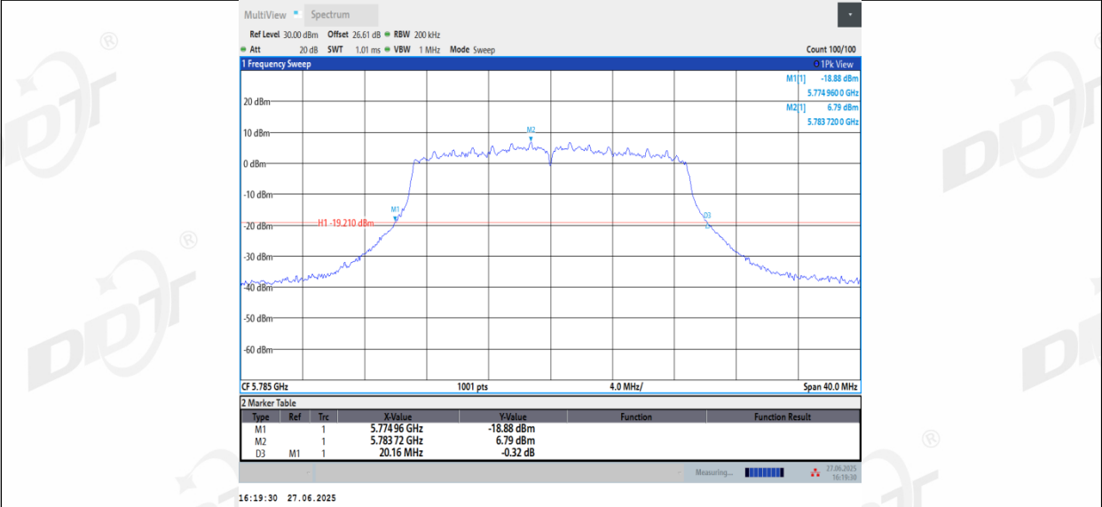
11N20_Ant3_5785
