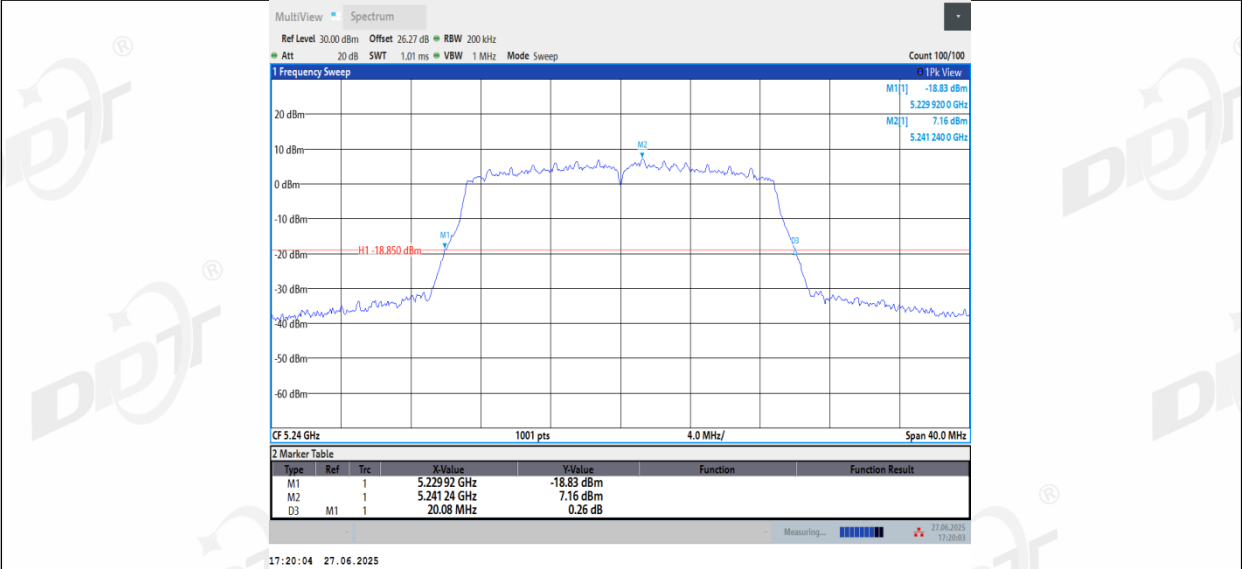
11AC20_Ant3_5240
