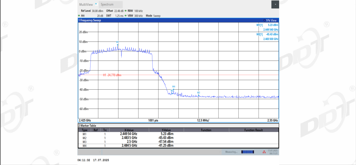
11AX40_Ant2_High_2452
