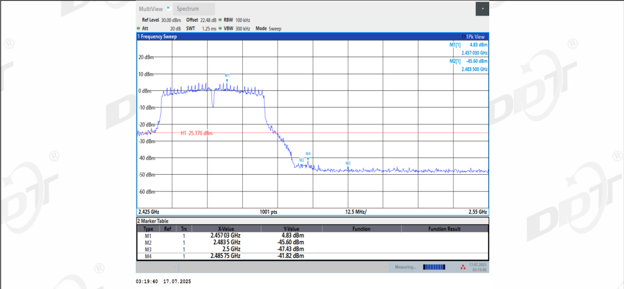
11N40_Ant2_High_2452
