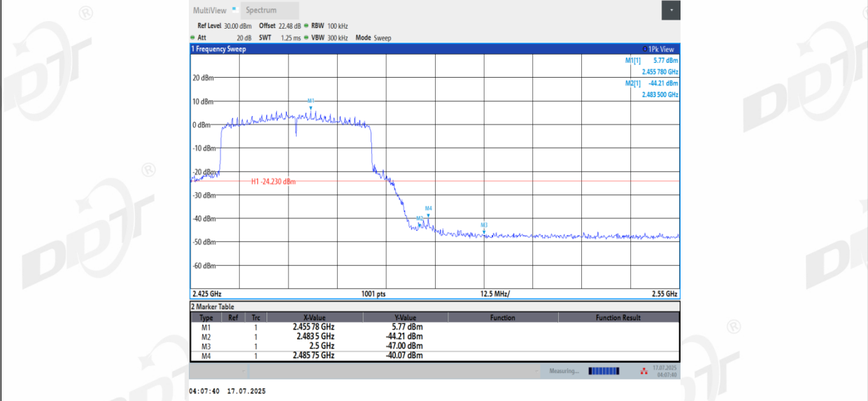
11AX40_Ant2_High_2452
