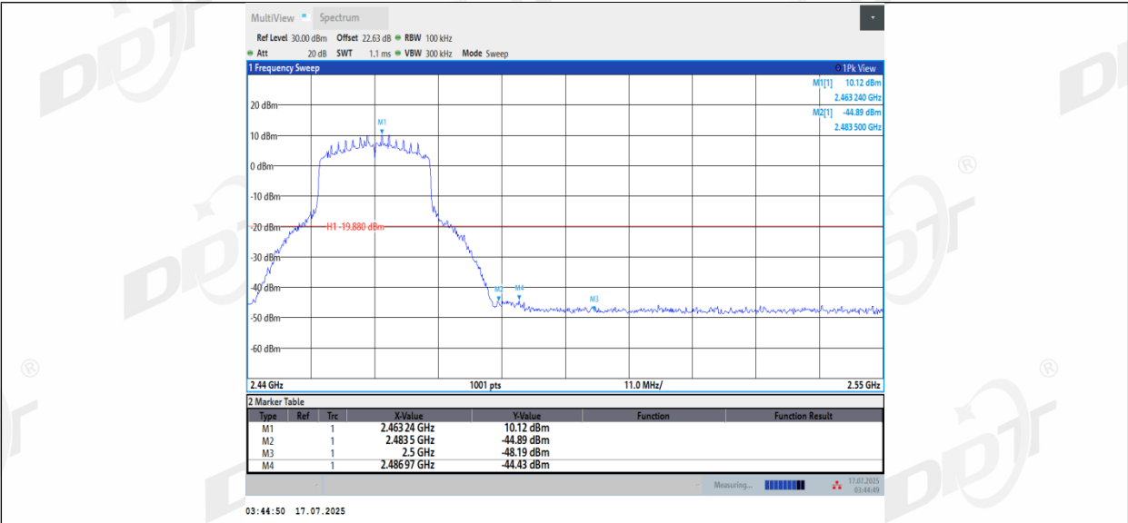
11AX20_Ant2_High_2462
