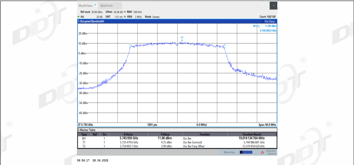
11AX20_Ant2_5745
