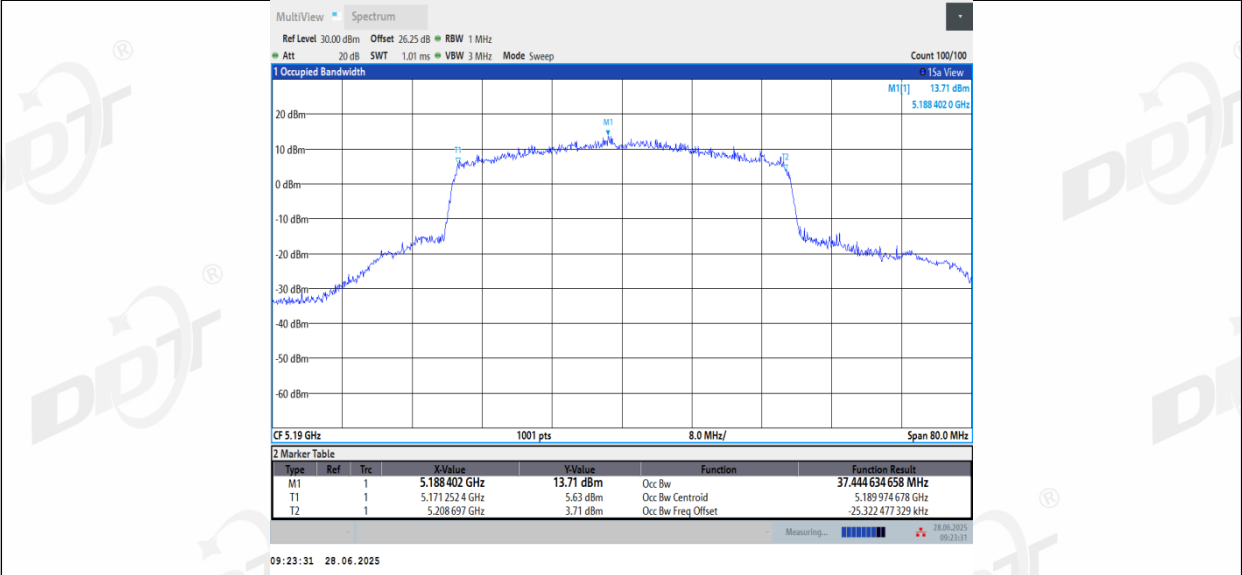
11AX40_Ant3_5190
