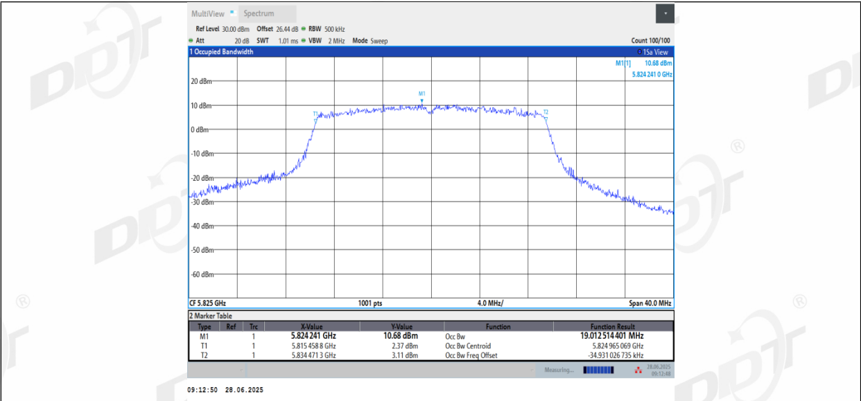
11AX20_Ant2_5825
