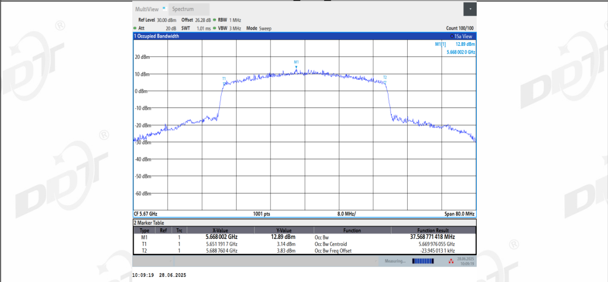
11AX40_Ant3_5670
