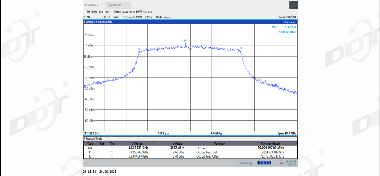
11AX20_Ant3_5825
