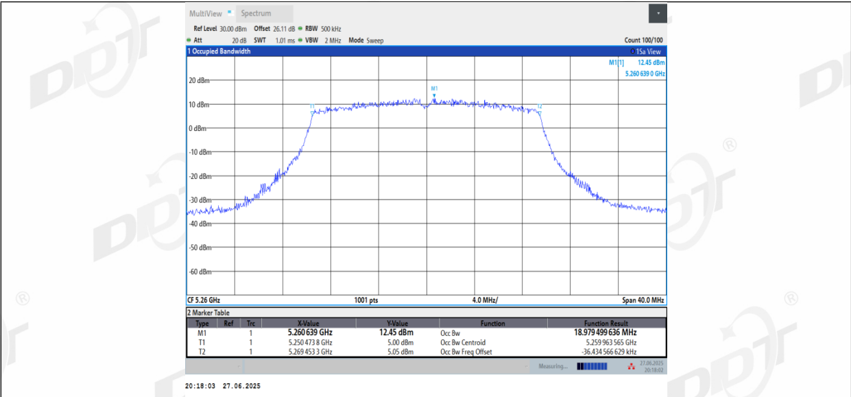
11AX20_Ant2_5260
