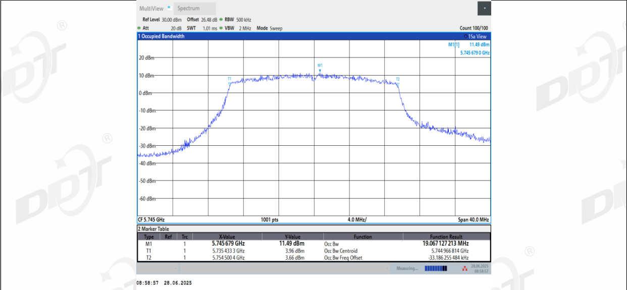
11AX20_Ant3_5745
