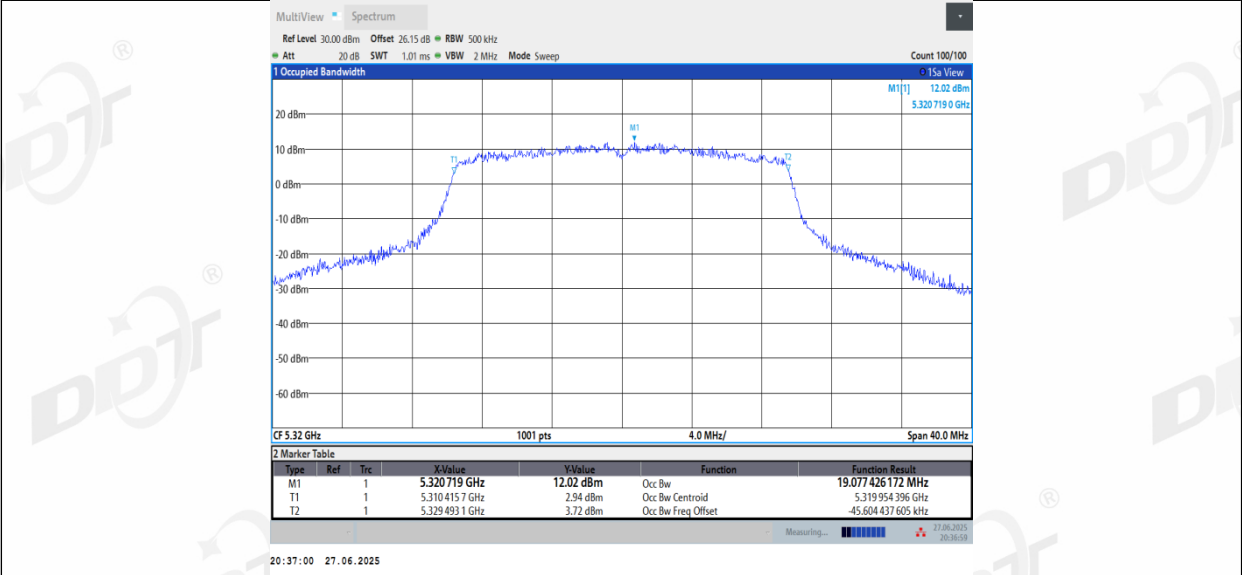
11AX20_Ant3_5320
