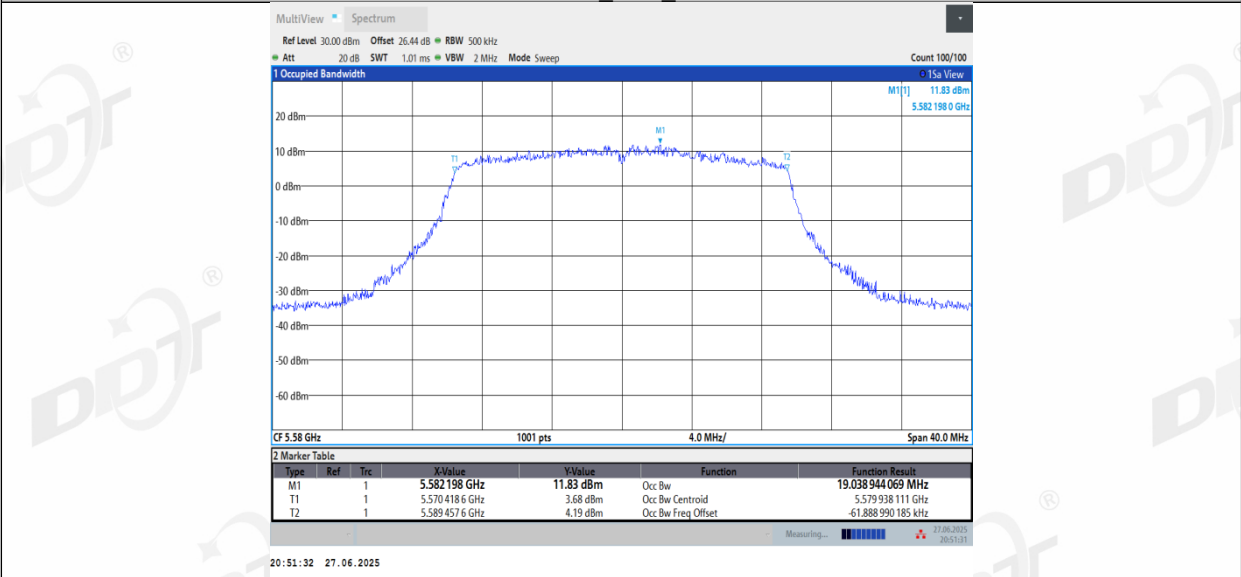
11AX20_Ant3_5580
