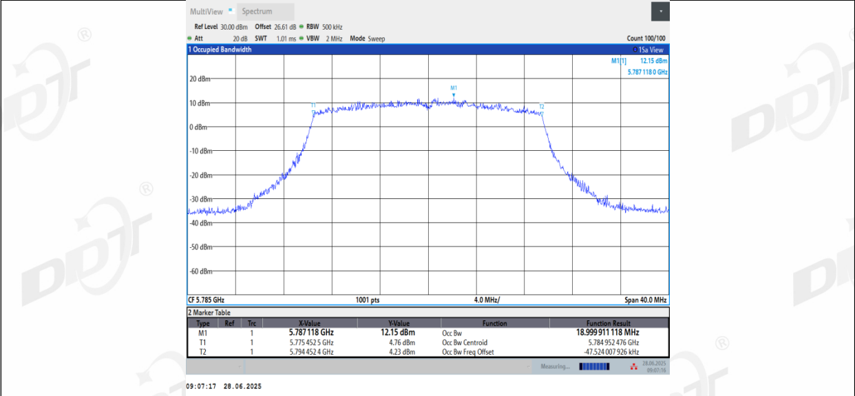
11AX20_Ant3_5785
