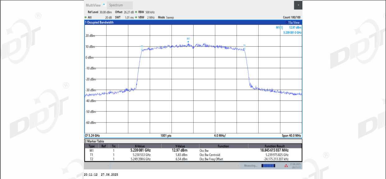
11AX20_Ant3_5240
