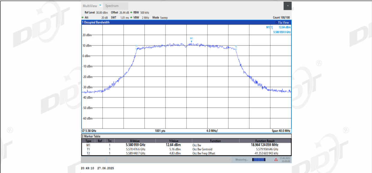
11AX20_Ant2_5580
