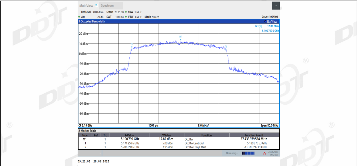
11AX40_Ant2_5190
