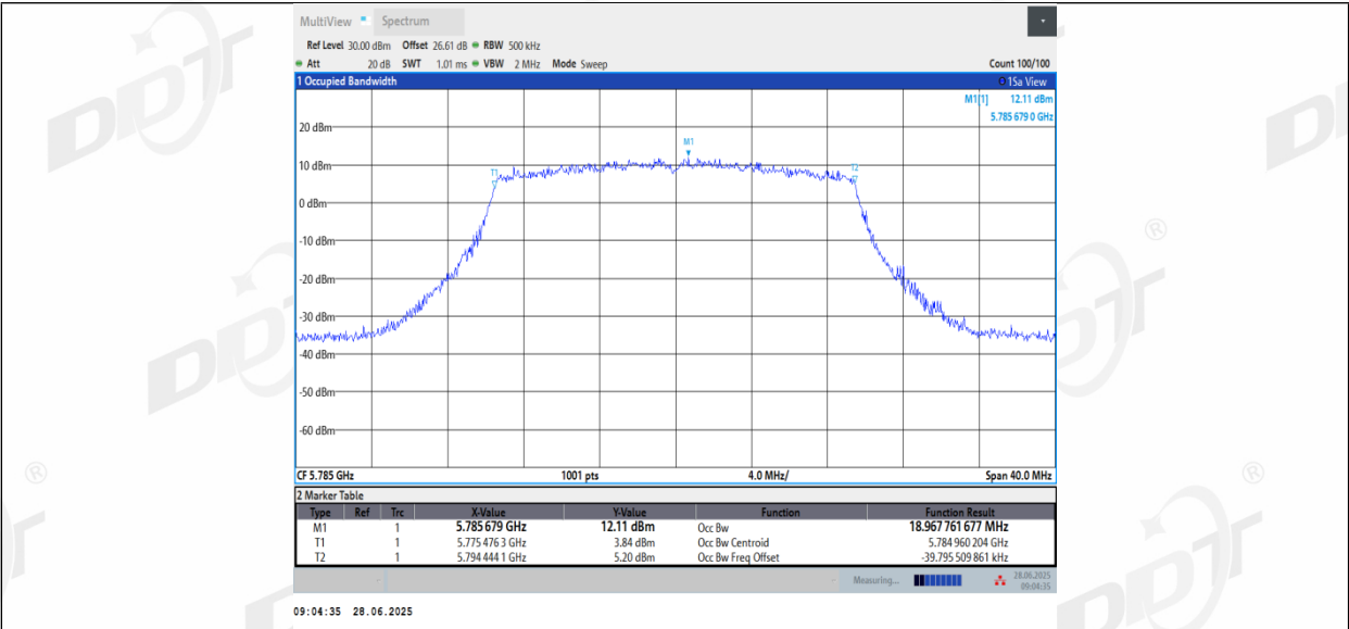
11AX20_Ant2_5785
