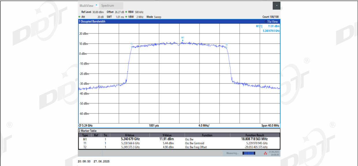
11AX20_Ant2_5240
