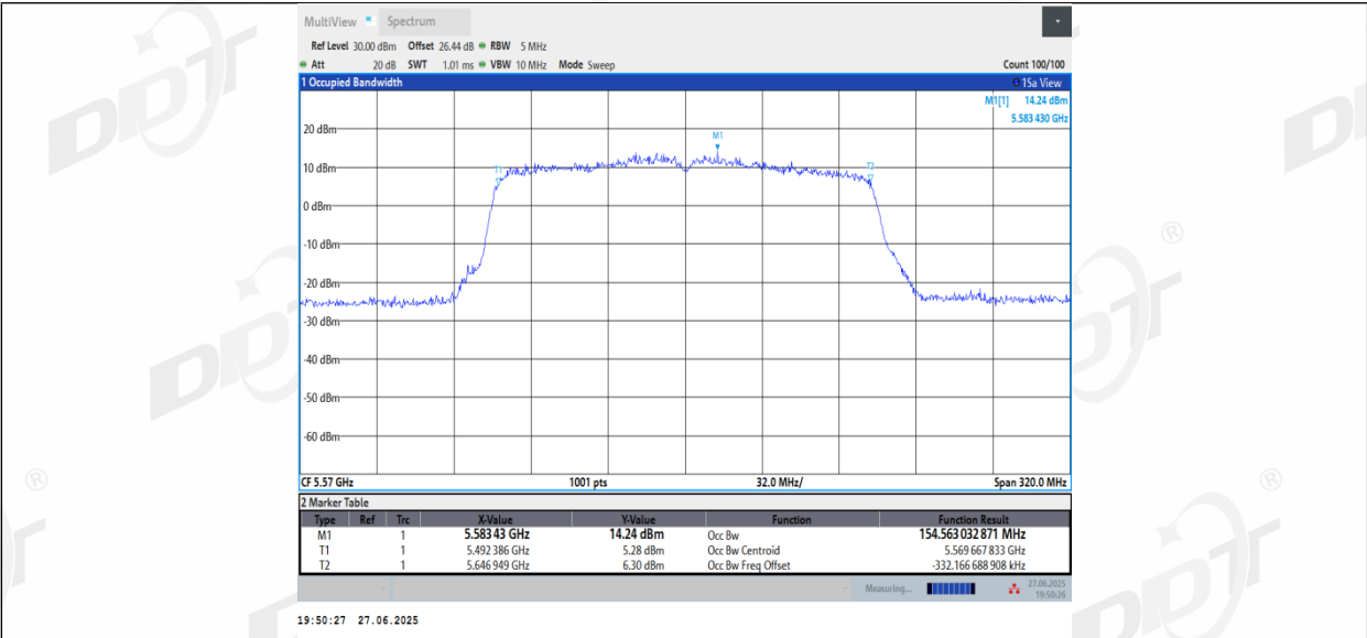
11AC160_Ant2_5570
