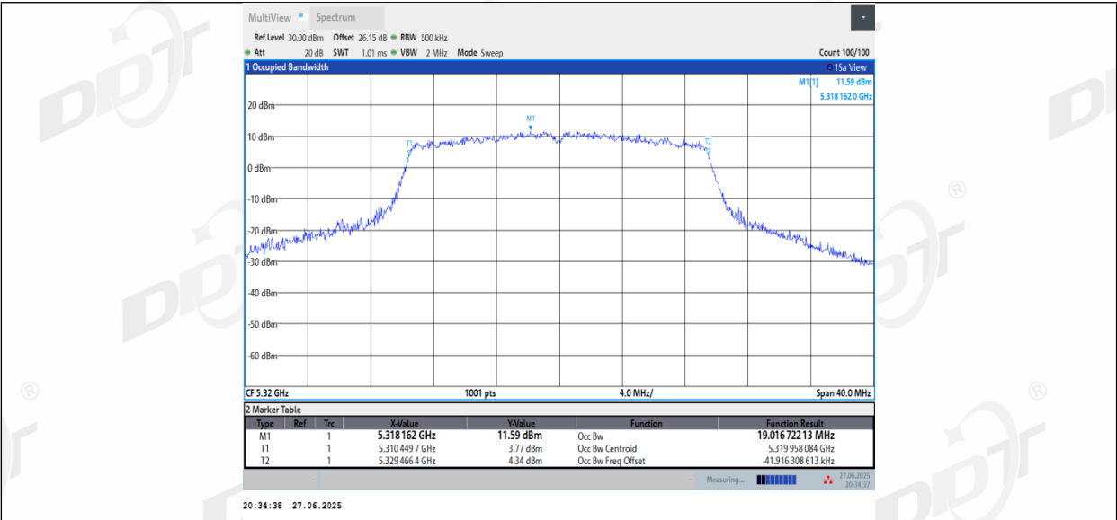
11AX20_Ant2_5320
