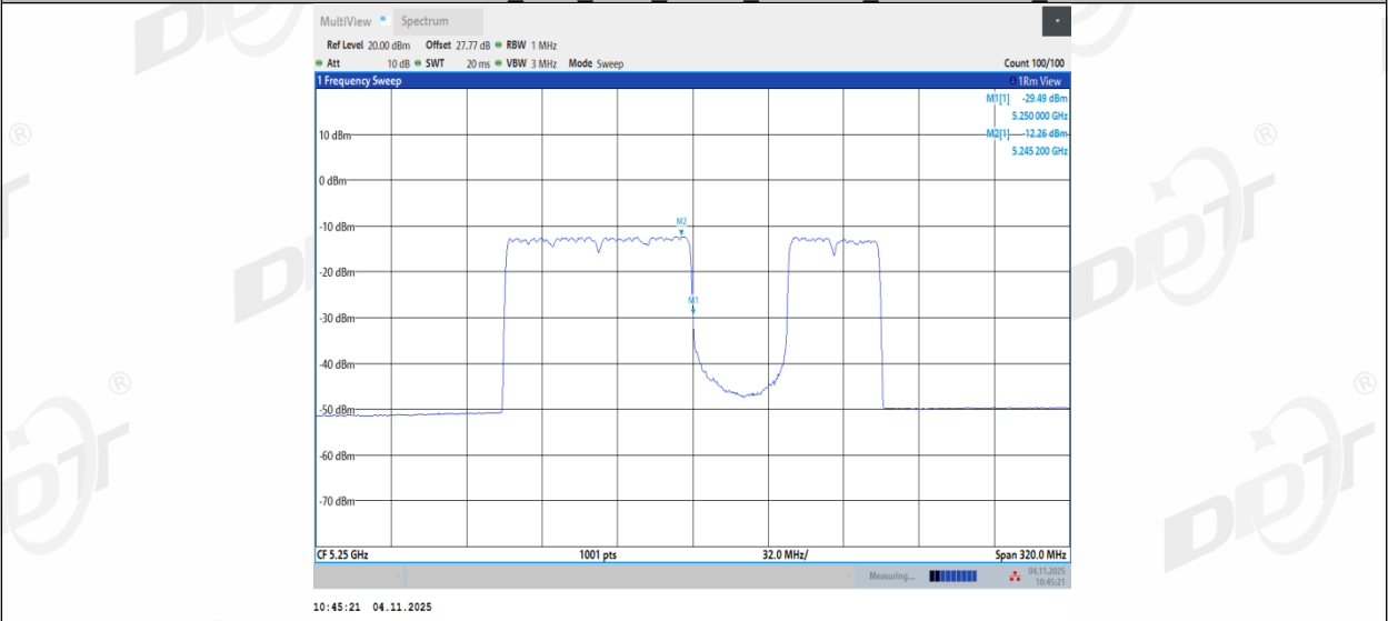
11BE160MIMO_Ant1_5250_UNII-1_996+484_Non-OFDMA_4
