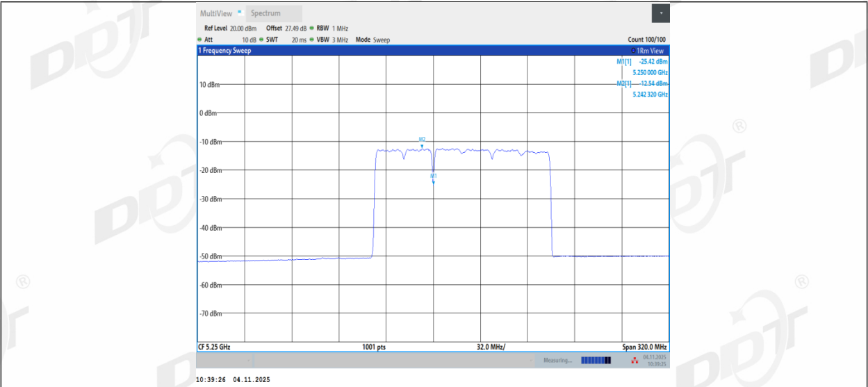
11BE160MIMO_Ant1_5250_UNII-1_996+484_Non-OFDMA_2
