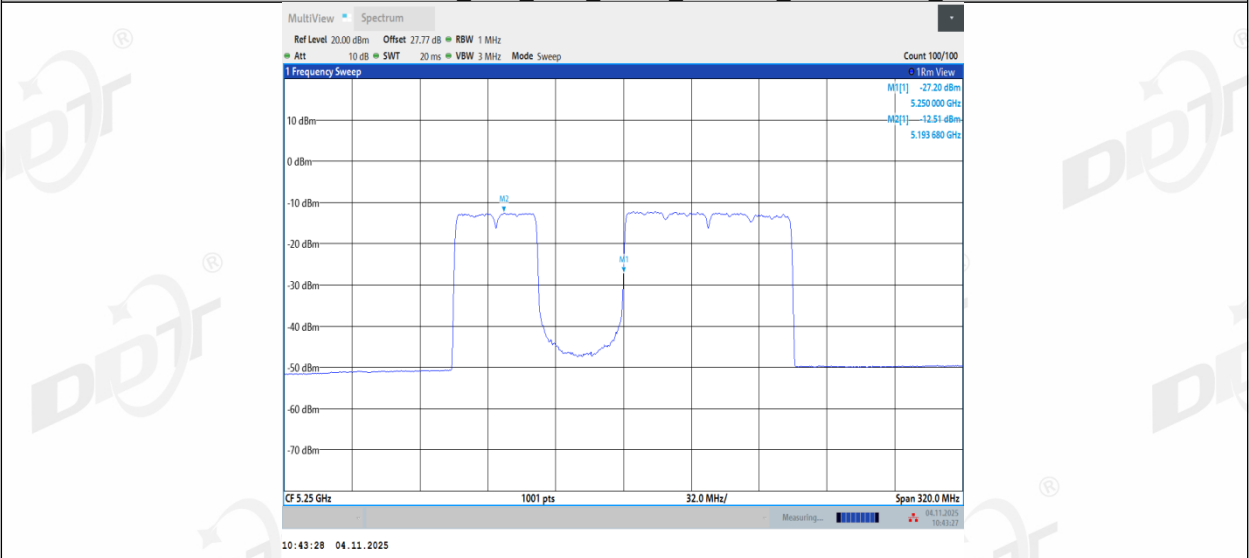
11BE160MIMO_Ant1_5250_UNII-1_996+484_Non-OFDMA_3
