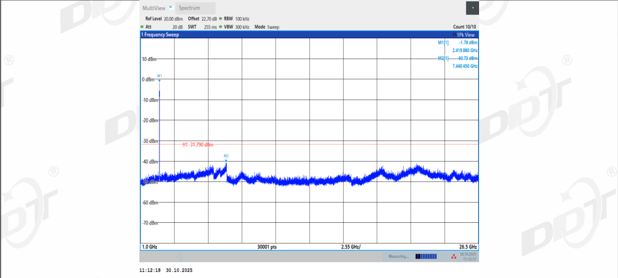
11BE40MIMO_Ant1_2437_0~Reference
