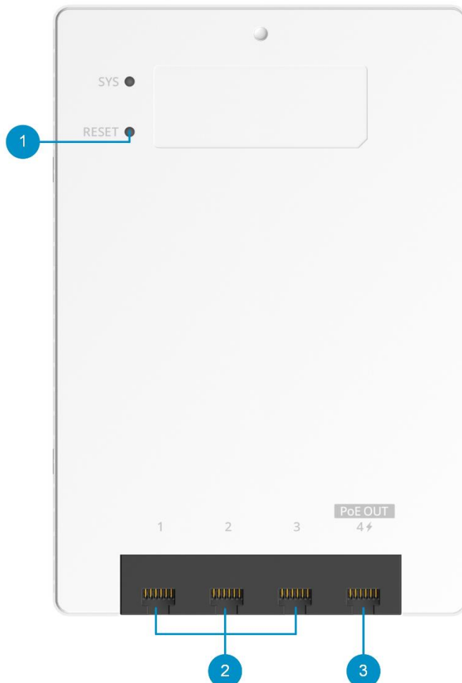
Figure 1-2 Front Panel
