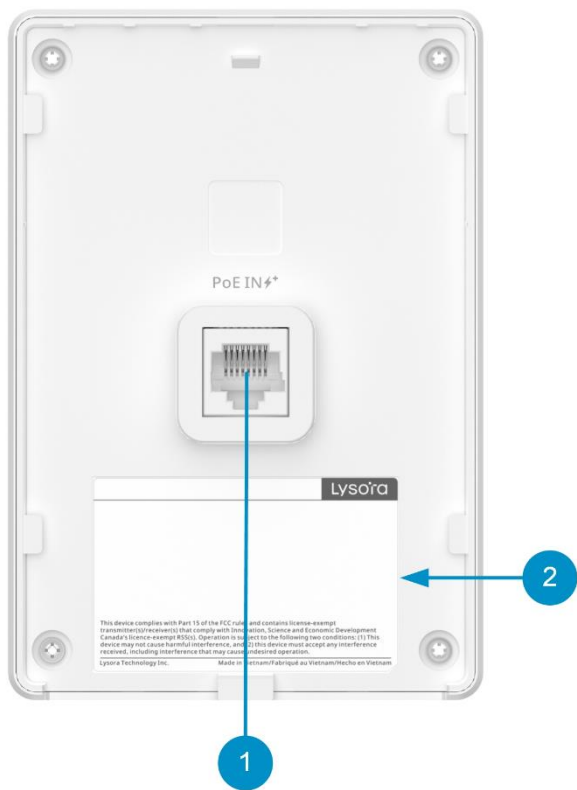
Figure 1-3Rear Panel
