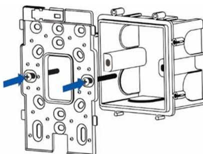
Figure 3-2 Installing the Mounting Bracket
