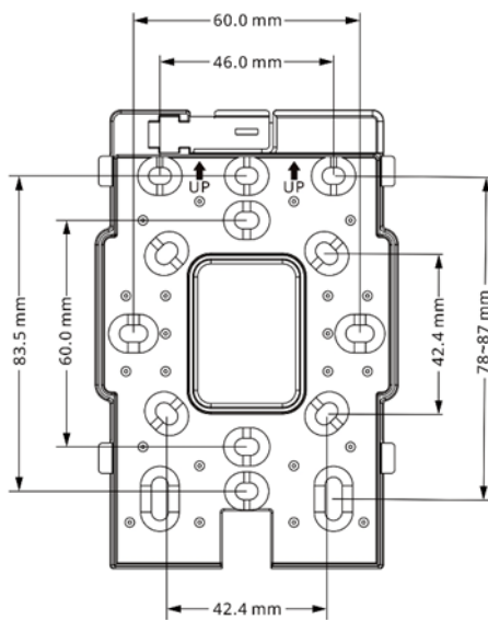
Figure 3-1 Dimensions of the Mounting Bracket
