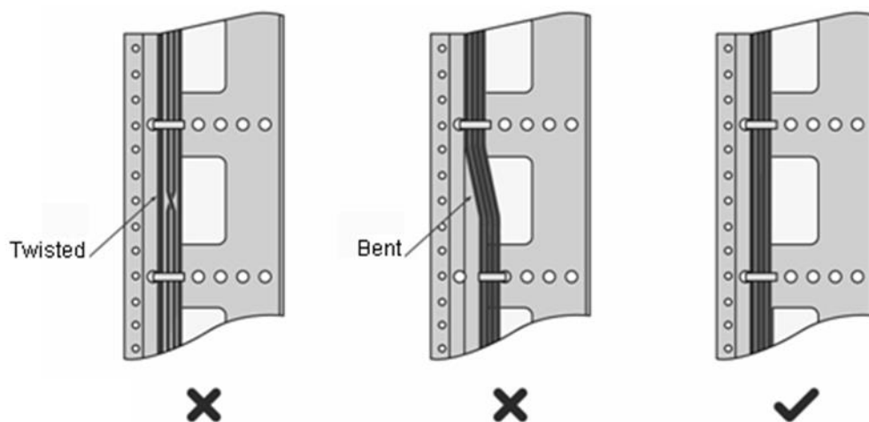
Figure 7-3 Bundling Cables (1)
