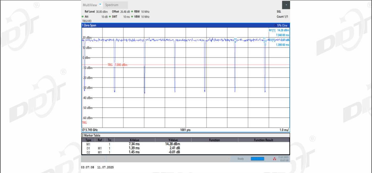
11A-CDD_Ant3_5745
