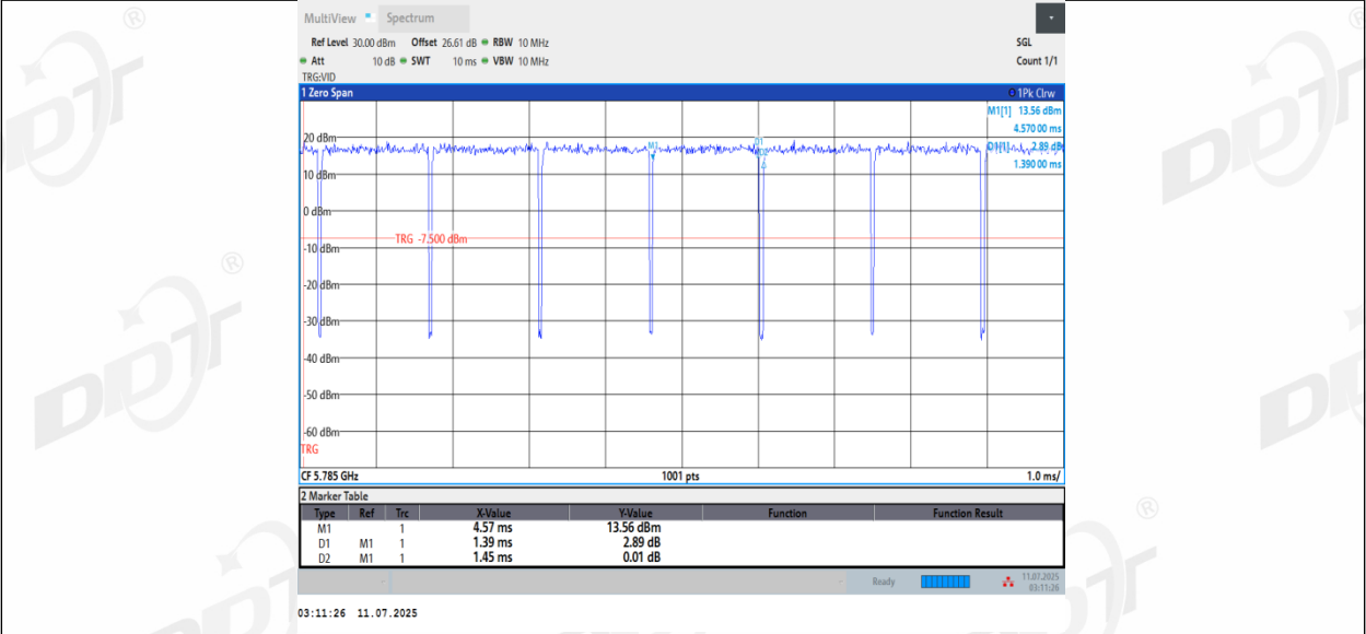
11A-CDD_Ant3_5785
