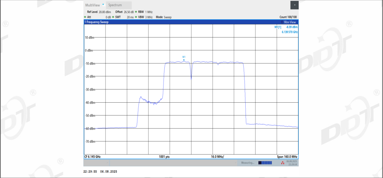
11BE80MIMO_Ant3_6145_484+242_Non-OFDMA_2
