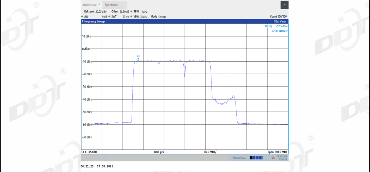
11BE80MIMO_Ant3_6145_484+242_Non-OFDMA_1
