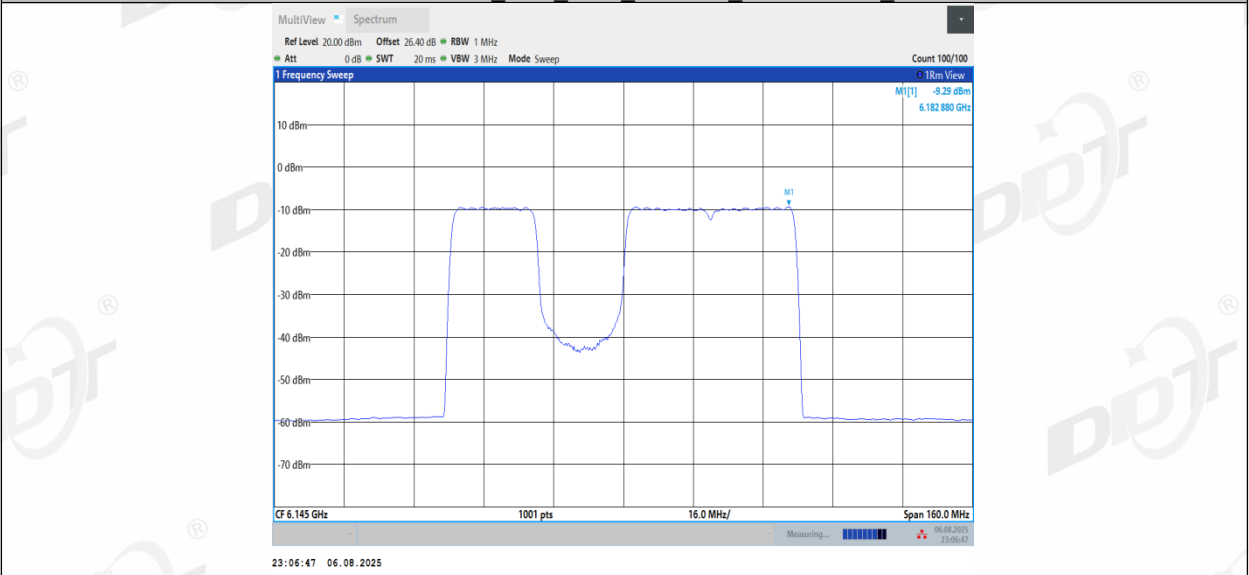
11BE80MIMO_Ant2_6145_484+242_Non-OFDMA_3
