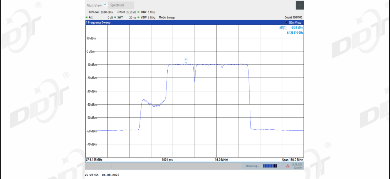
11BE80MIMO_Ant2_6145_484+242_Non-OFDMA_2
