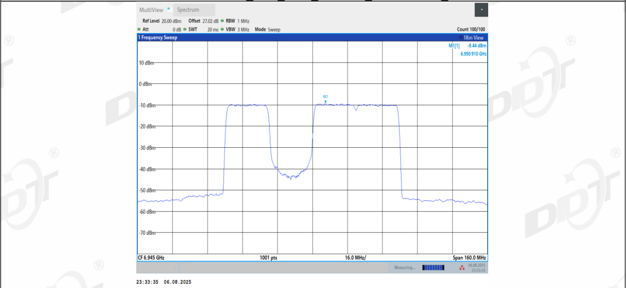
11BE80MIMO_Ant2_6945_484+242_Non-OFDMA_3
