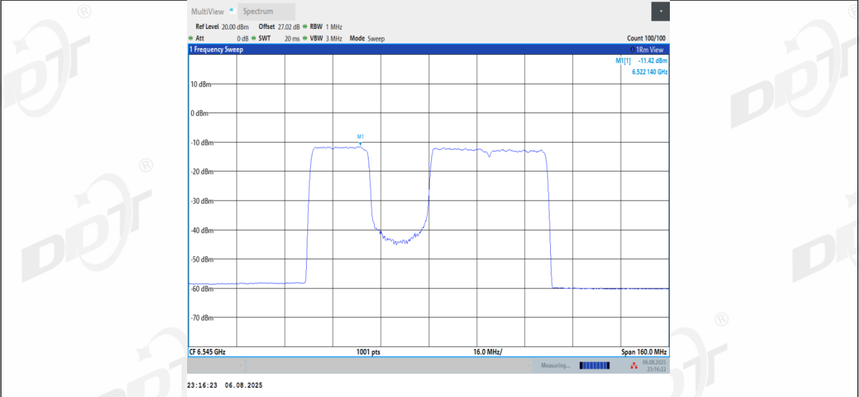
11BE80MIMO_Ant1_6545_484+242_Non-OFDMA_3
