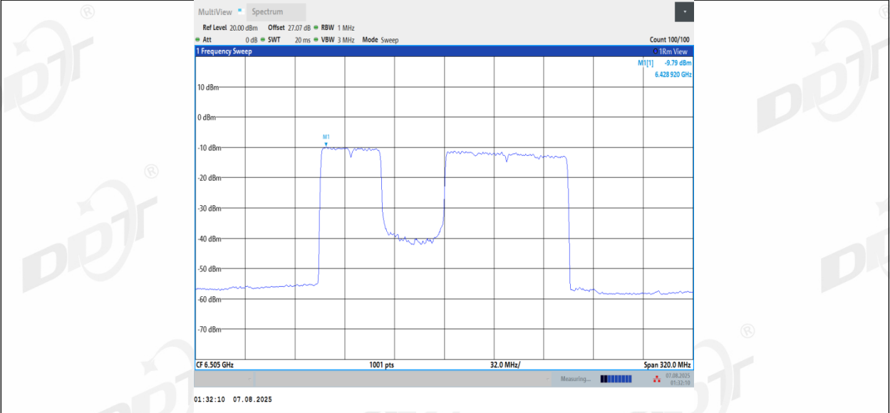
11BE160MIMO_Ant1_6505_996+484_Non-OFDMA_3
