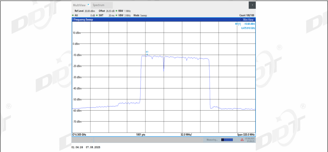
11BE160MIMO_Ant1_6505_996+484_Non-OFDMA_2
