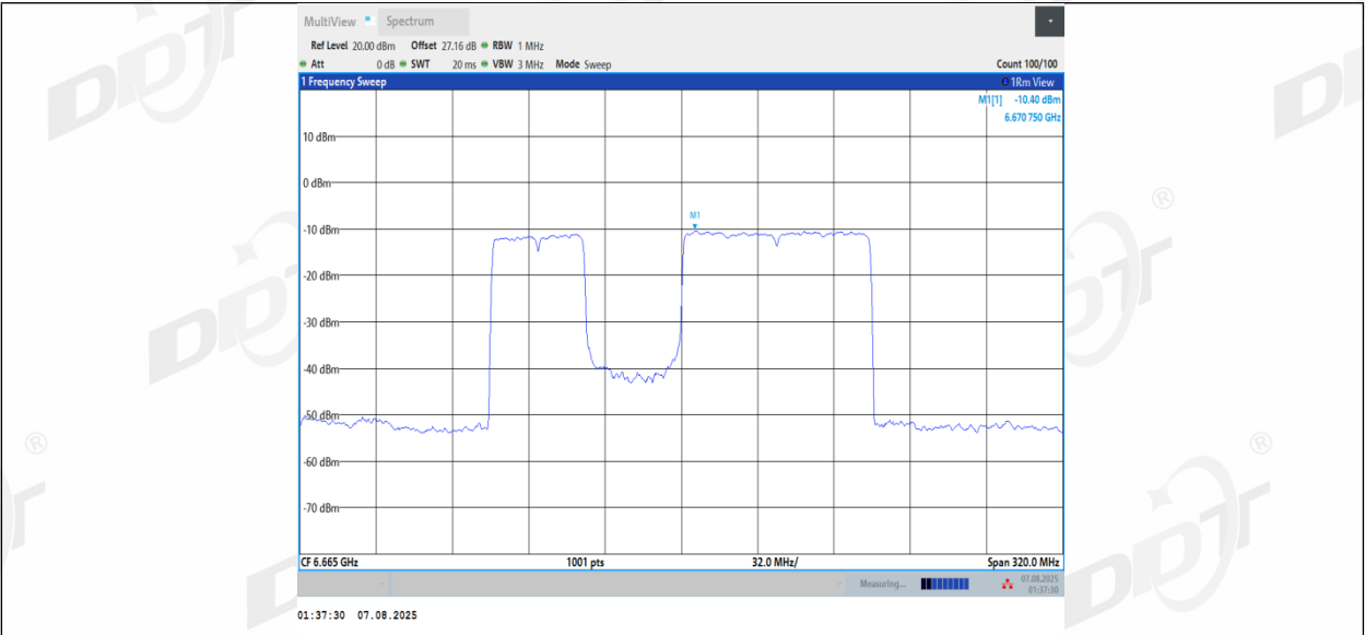
11BE160MIMO_Ant3_6665_996+484_Non-OFDMA_3
