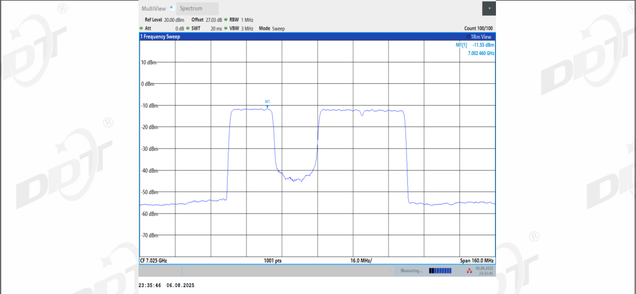
11BE80MIMO_Ant1_7025_484+242_Non-OFDMA_3
