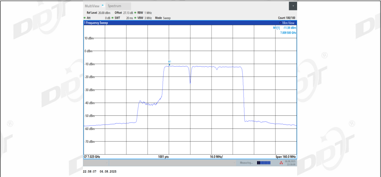
11BE80MIMO_Ant1_7025_484+242_Non-OFDMA_2
