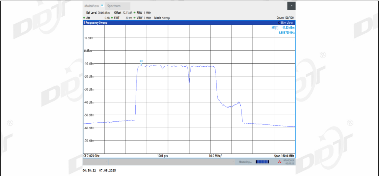
11BE80MIMO_Ant2_7025_484+242_Non-OFDMA_1
