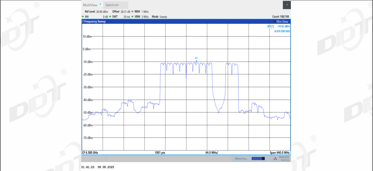
11BE320MIMO_Ant1_6585_2*996+484_Non-OFDMA_12
