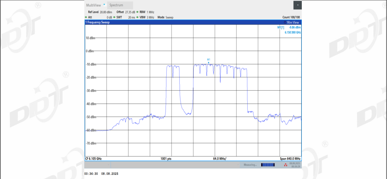
11BE320MIMO_Ant1_6105_2*996+484_Non-OFDMA_9
