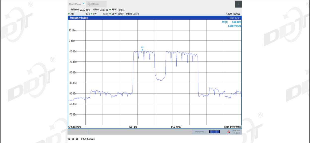
11BE320MIMO_Ant3_6585_2*996+484_Non-OFDMA_10
