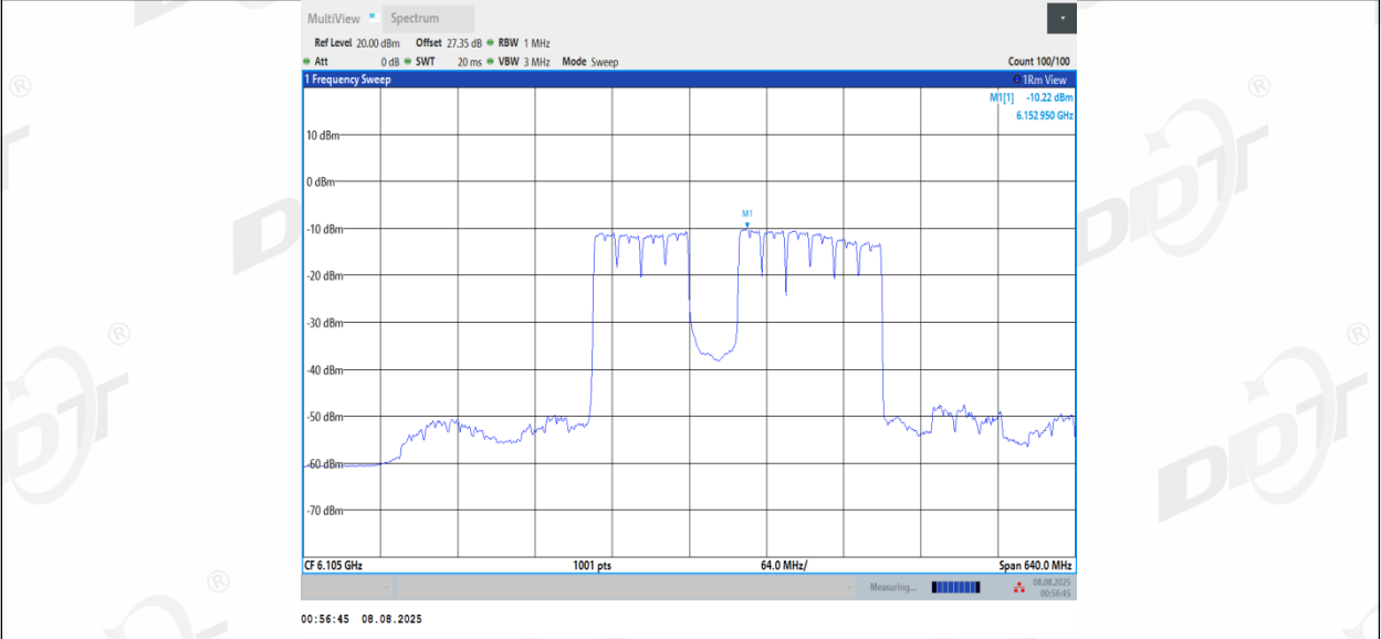
11BE320MIMO_Ant1_6105_2*996+484_Non-OFDMA_10
