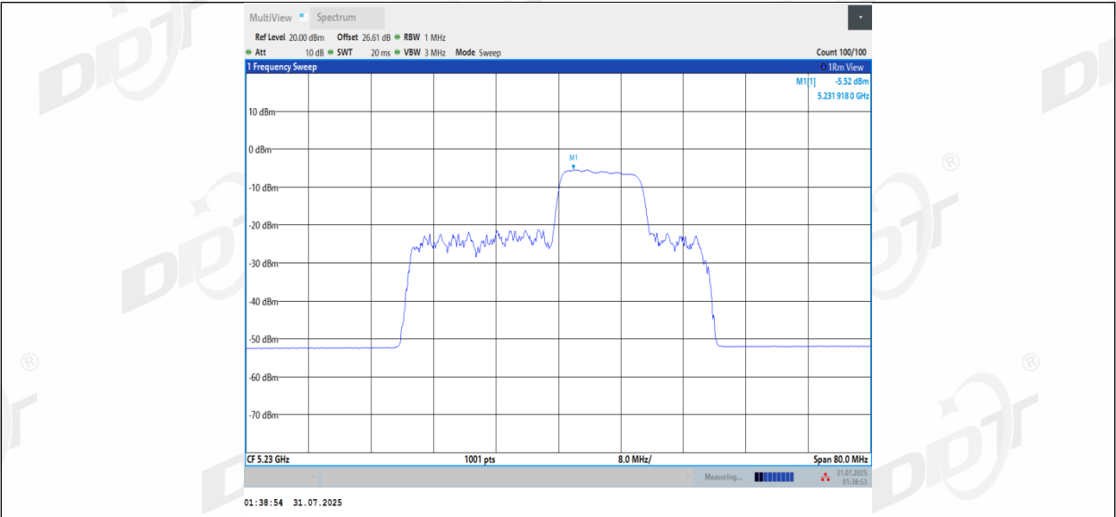
11BE40MIMO_Ant1_5230_106+26_OFDMA_4
