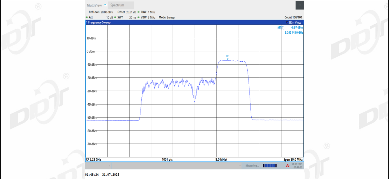
11BE40MIMO_Ant2_5230_106+26_OFDMA_3
