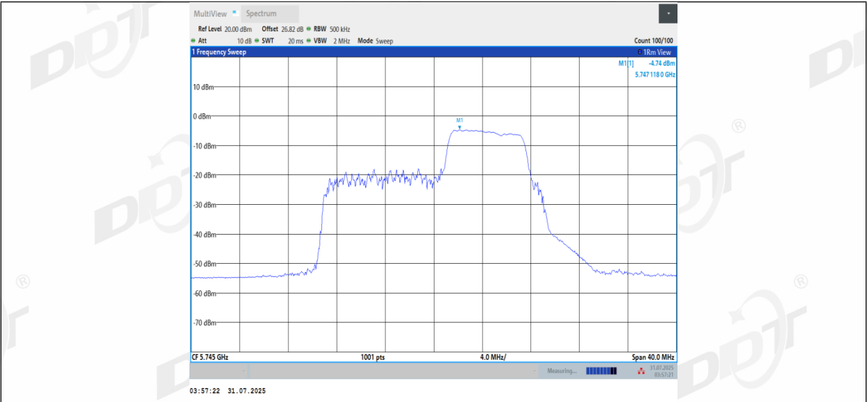
11BE20MIMO_Ant3_5745_106+26_OFDMA_1
