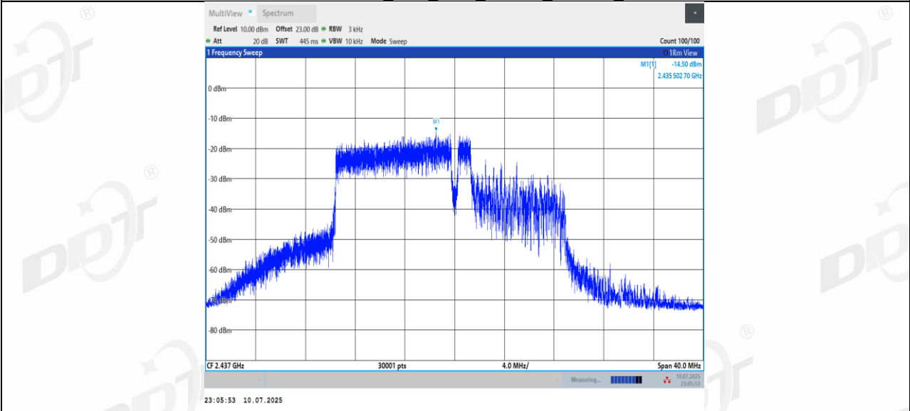
11BE20MIMO Ant1_2437_106+26_OFDMA_2
