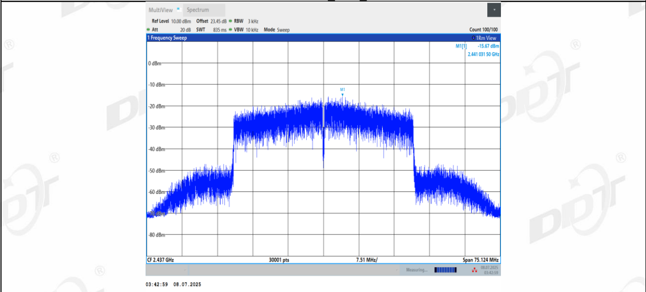
11BE40MIMO Ant2 2437
