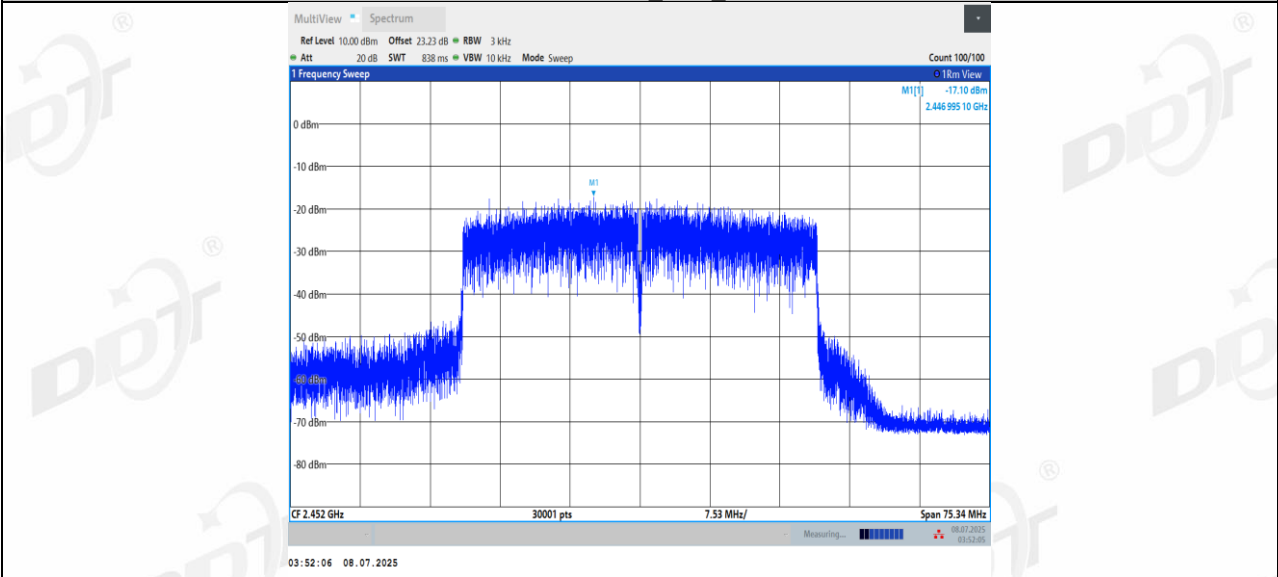
11BE40MIMO Ant2 2452
