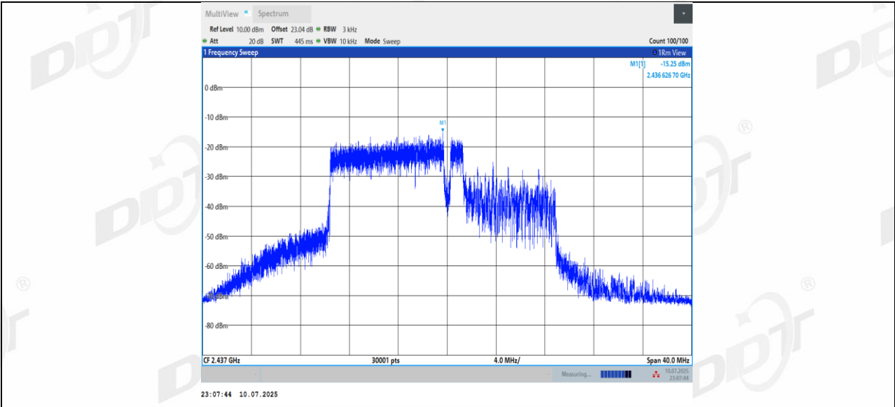
11BE20MIMO Ant2_2437_106+26_OFDMA_2
