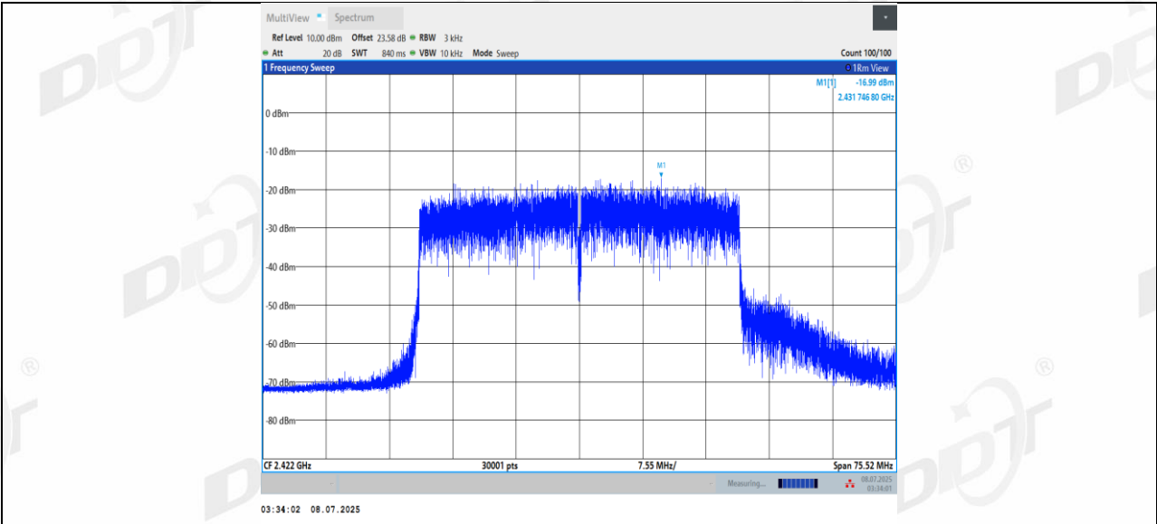
11BE40MIMO Ant2 2422
