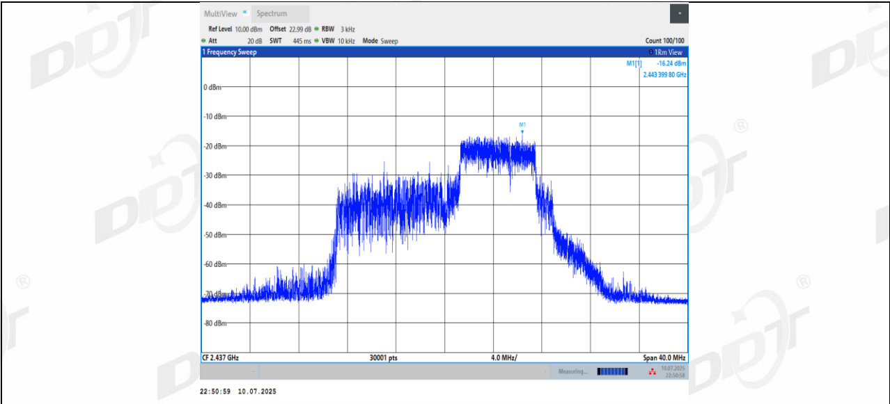
11BE20MIMO Ant1_2437_106+26_OFDMA_1
