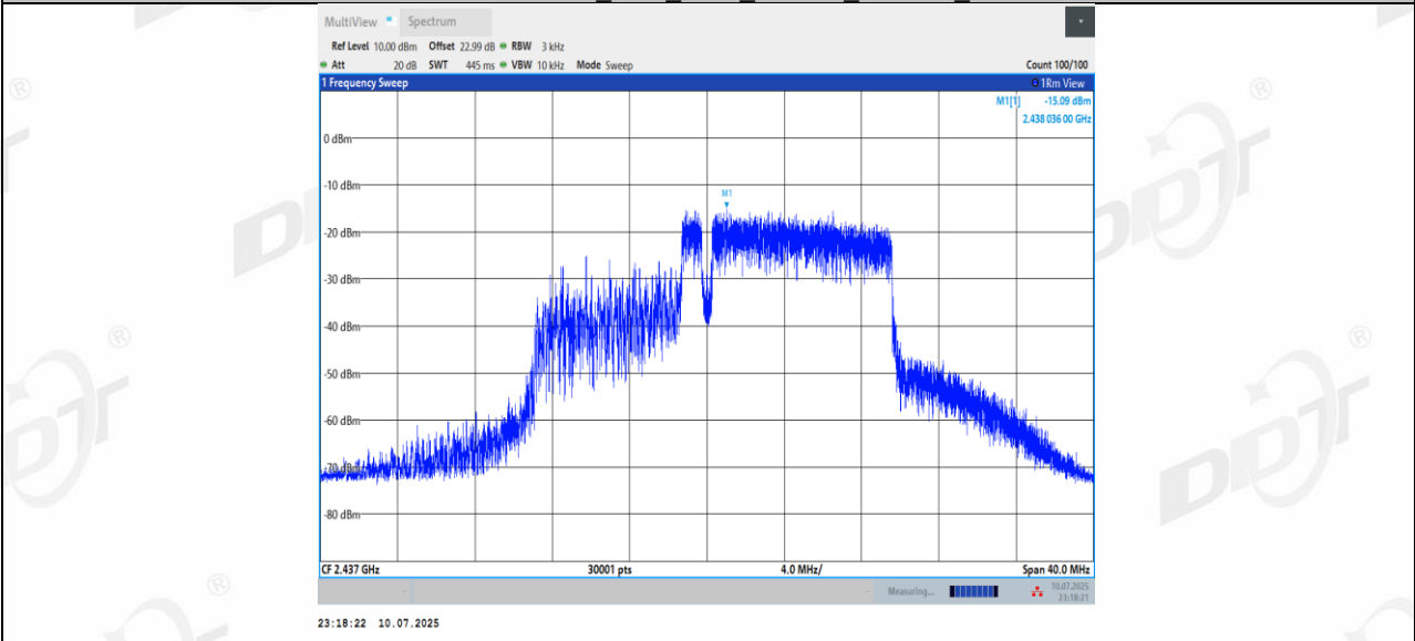
11BE20MIMO Ant2_2437_52+26_OFDMA_1
