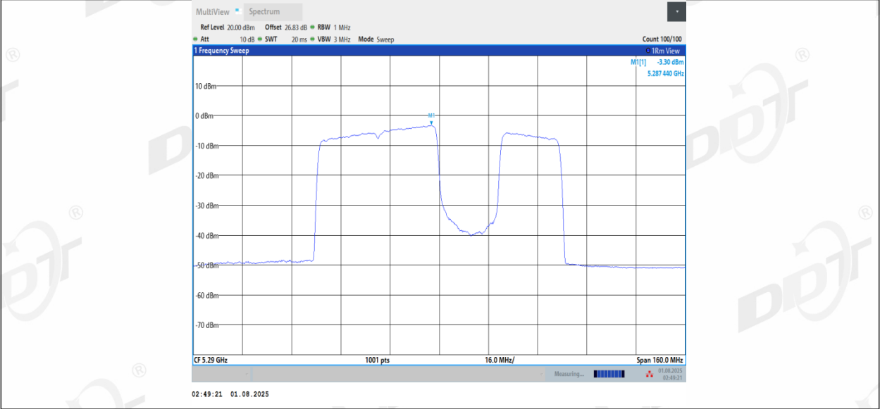
11BE80MIMO_Ant1_5290_484+242_Non-OFDMA_4
