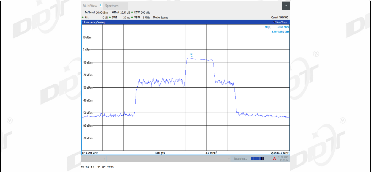
11BE40MIMO_Ant1_5795_106+26_OFDMA_4
