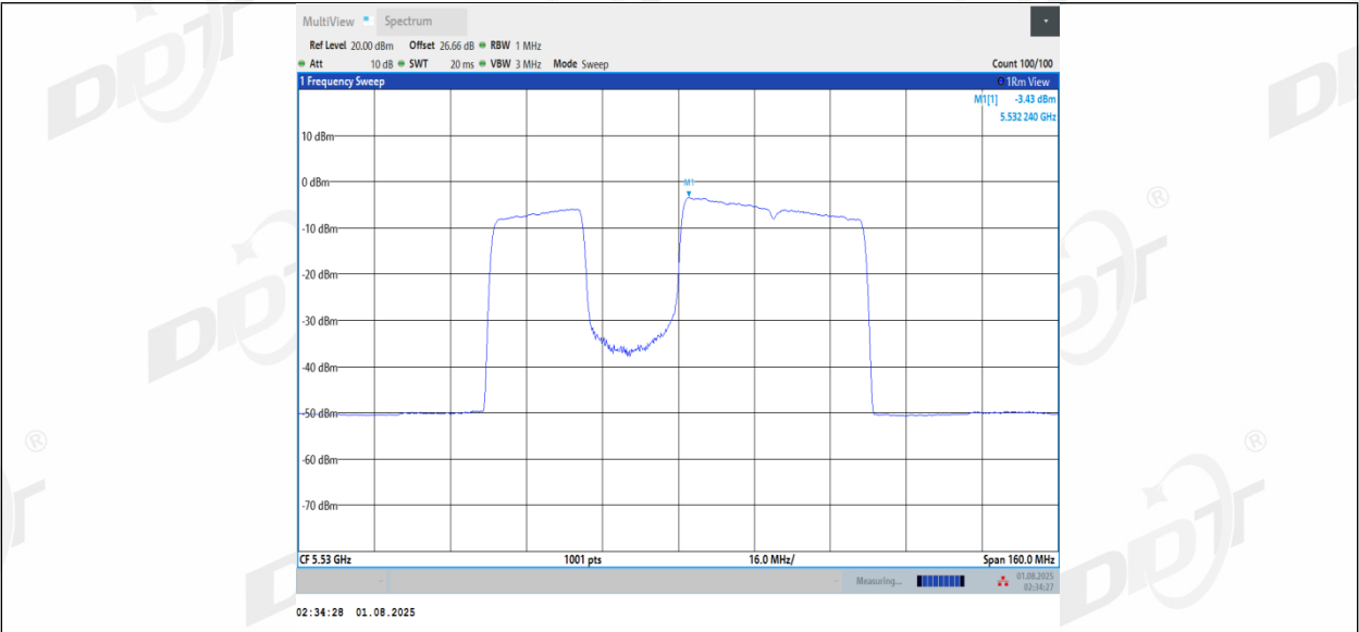
11BE80MIMO_Ant3 5530_484+242 Non-OFDMA_3
