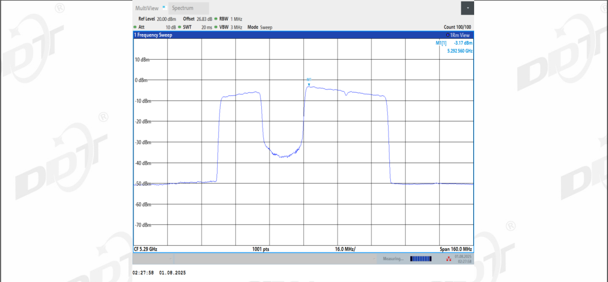
11BE80MIMO_Ant1_5290_484+242_Non-OFDMA_3
