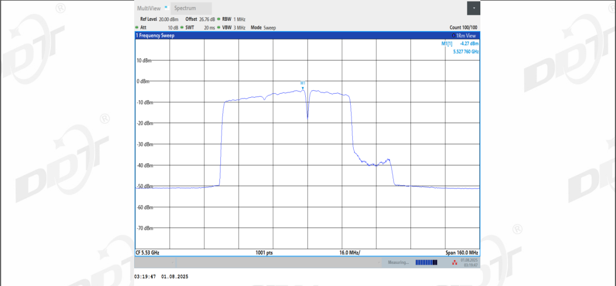
11BE80MIMO_Ant3_5530_484+242_Non-OFDMA_1
