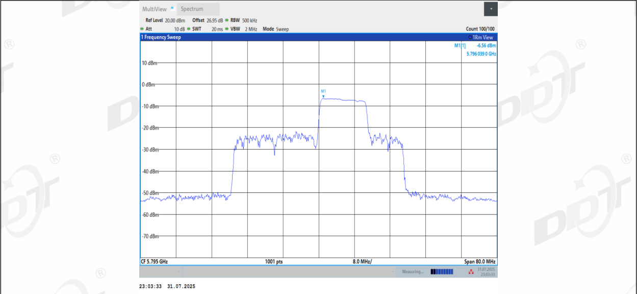
11BE40MIMO_Ant2_5795_106+26_OFDMA_4
