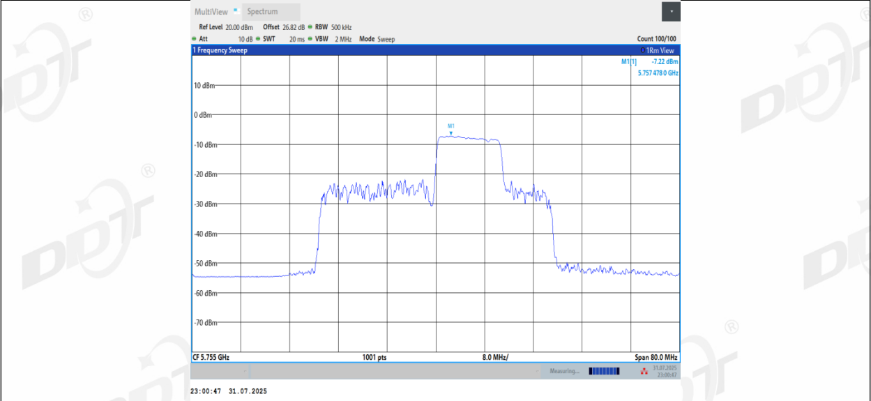
11BE40MIMO_Ant3_5755_106+26_OFDMA_4
