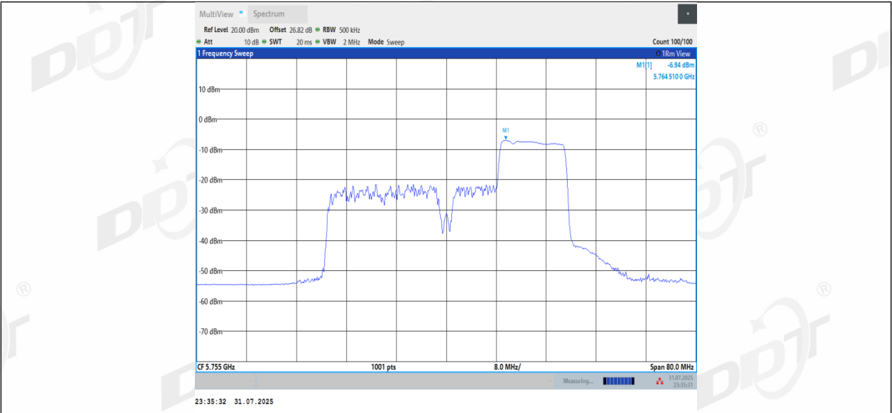
11BE40MIMO_Ant3_5755_106+26_OFDMA_3
