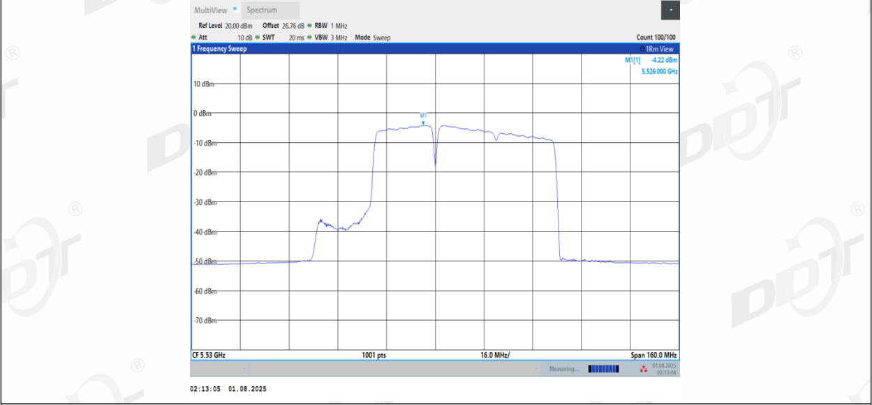
11BE80MIMO_Ant3_5530_484+242_Non-OFDMA_2
