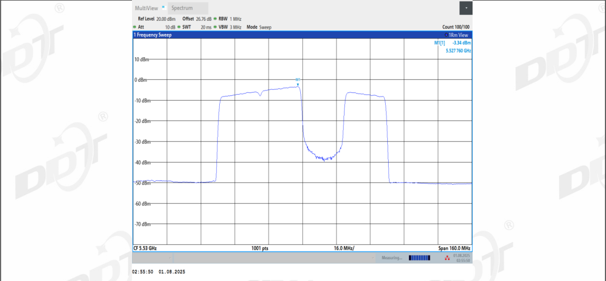
11BE80MIMO_Ant3 5530_484+242 Non-OFDMA_4
