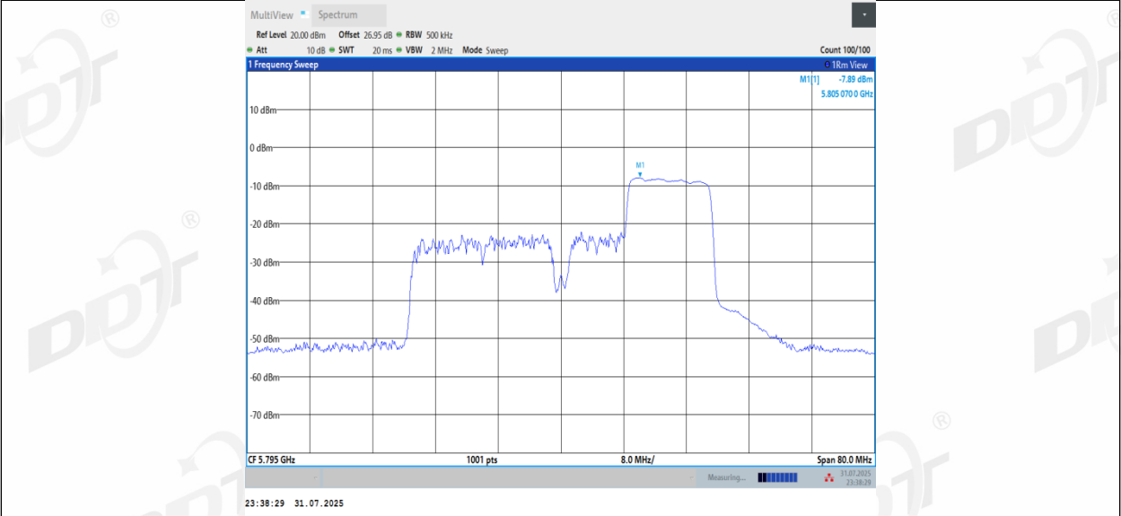
11BE40MIMO_Ant2_5795_106+26_OFDMA_3
