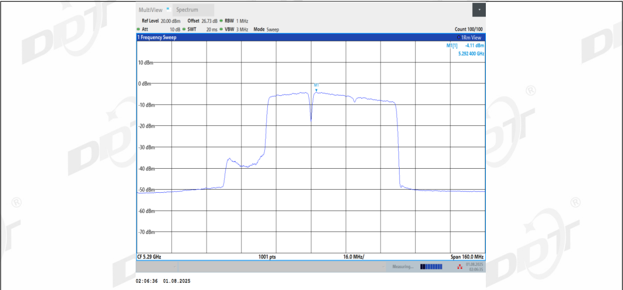
11BE80MIMO_Ant1_5290_484+242_Non-OFDMA_2
