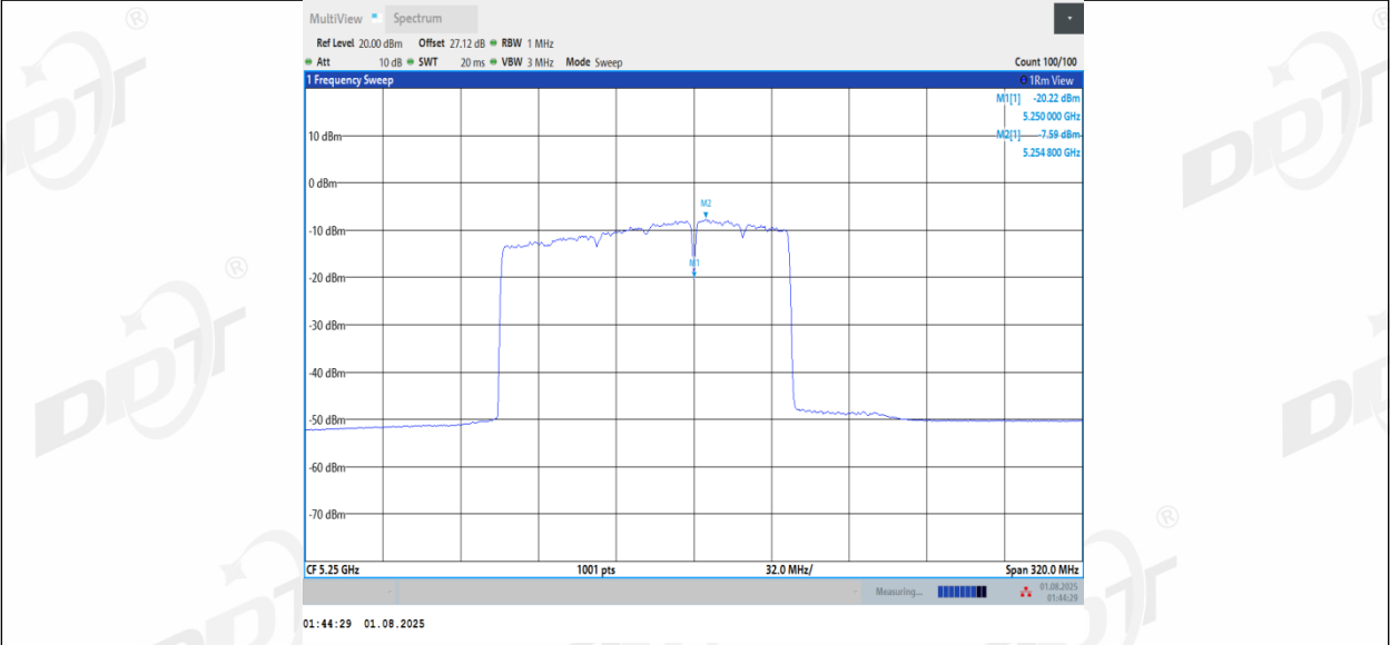
11BE160MIMO_Ant2_5250_UNII-2A_996+484_Non-OFDMA_1
