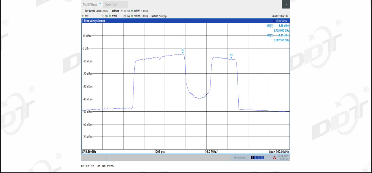
11BE80MIMO Ant1_5690_UNII-2C_484+242_Non-OFDMA 4
