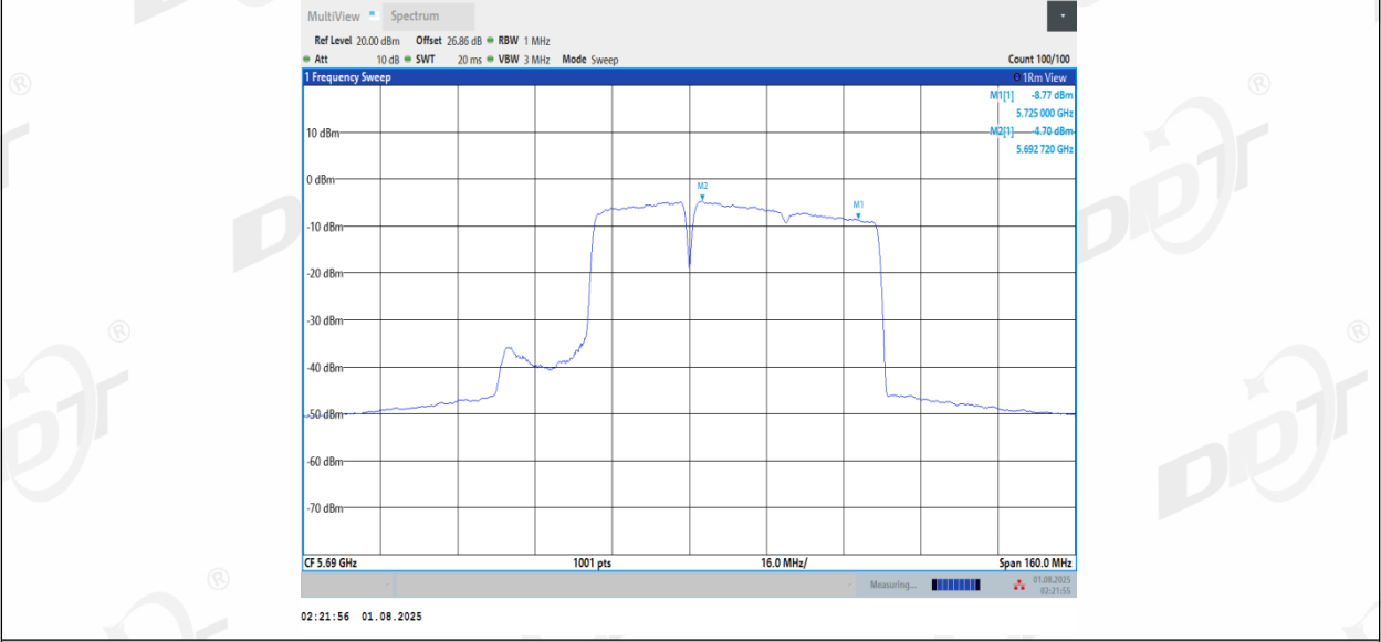
11BE80MIMO Ant3_5690_UNII-2C_484+242_Non-OFDMA_2
