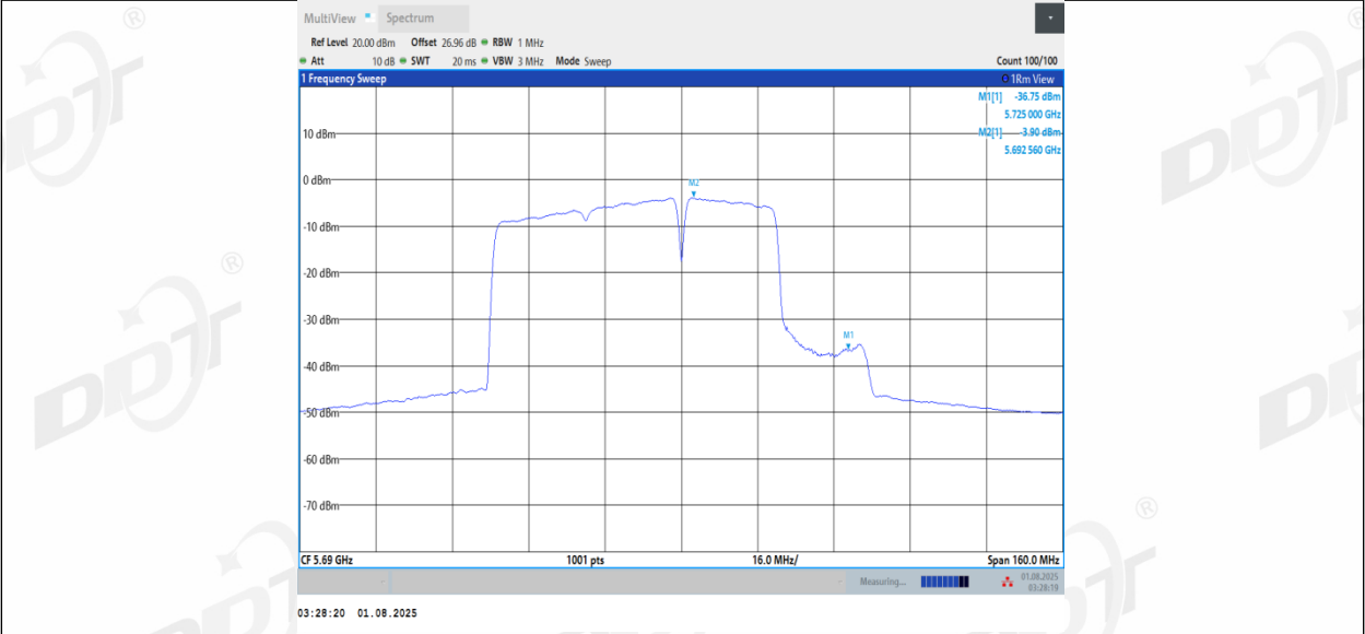
11BE80MIMO Ant3_5690_UNII-2C_484+242_Non-OFDMA_1
