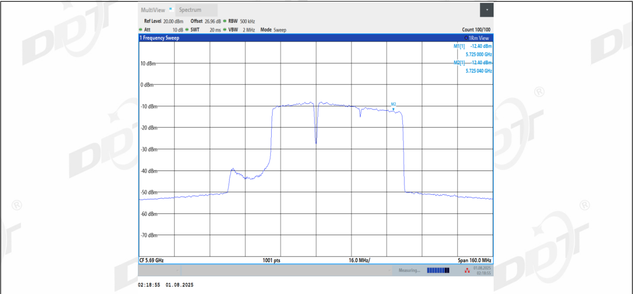
11BE80MIMO_Ant1_5690_UNII-3_484+242_Non-OFDMA_2
