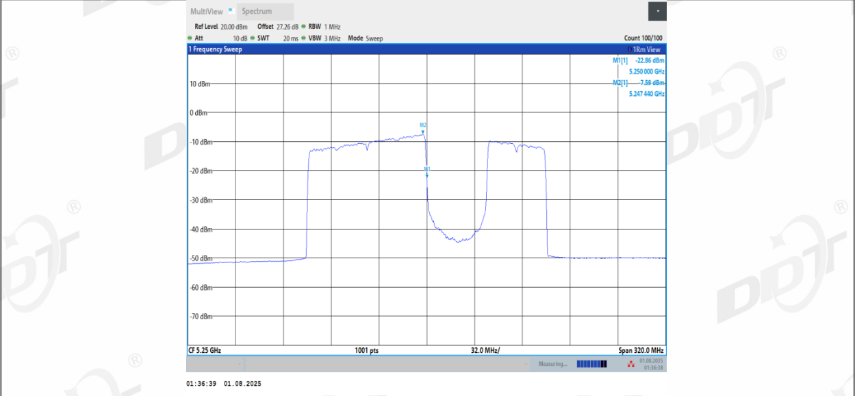
11BE160MIMO_Ant1_5250_UNII-1_996+484_Non-OFDMA_4
