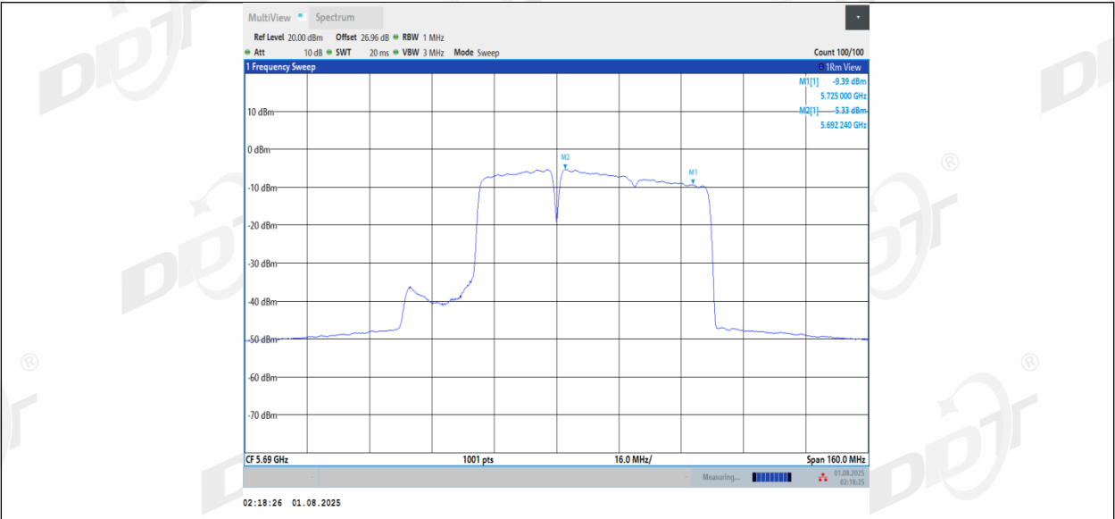
11BE80MIMO Ant1_5690_UNII-2C_484+242_Non-OFDMA 2
