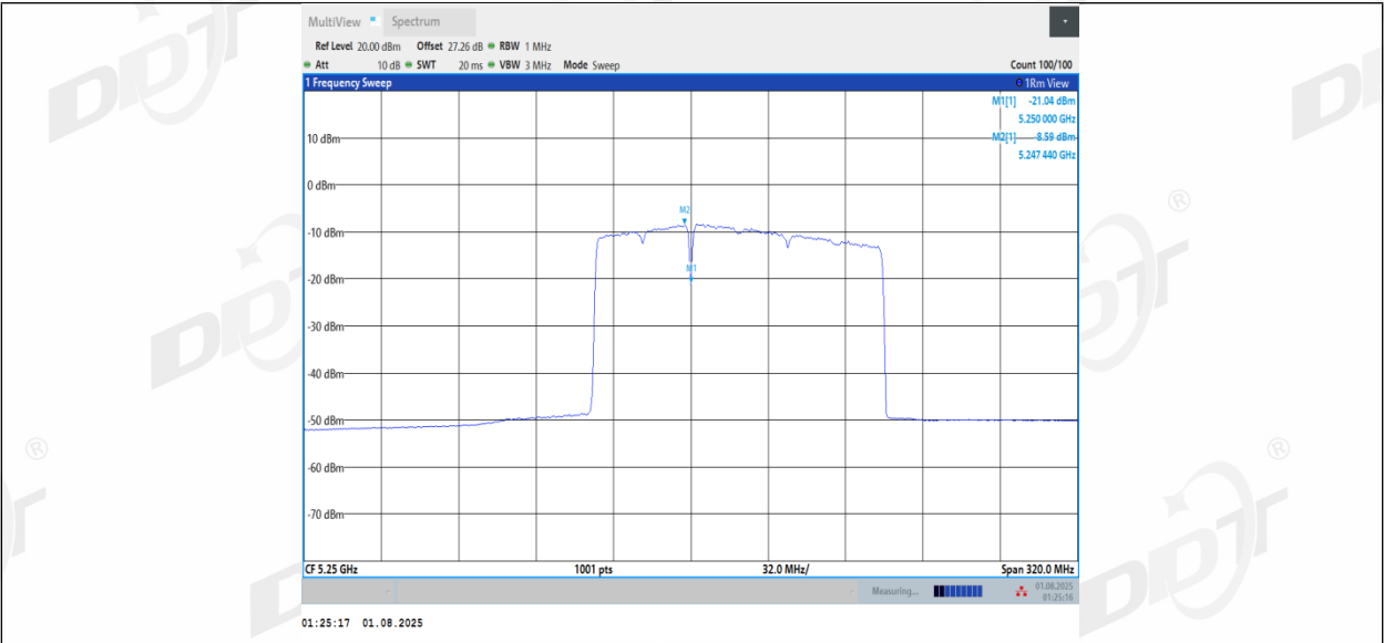
11BE160MIMO_Ant1_5250_UNII-1_996+484_Non-OFDMA_2
