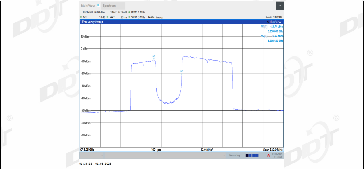
11BE160MIMO_Ant3_5250_UNII-1_996+484_Non-OFDMA_3
