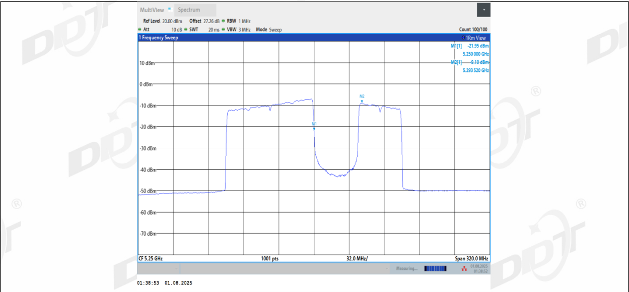
11BE160MIMO_Ant2_5250_UNII-2A_996+484_Non-OFDMA_4
