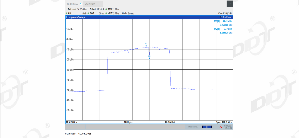
11BE160MIMO_Ant1_5250_UNII-2A_996+484_Non-OFDMA_1
