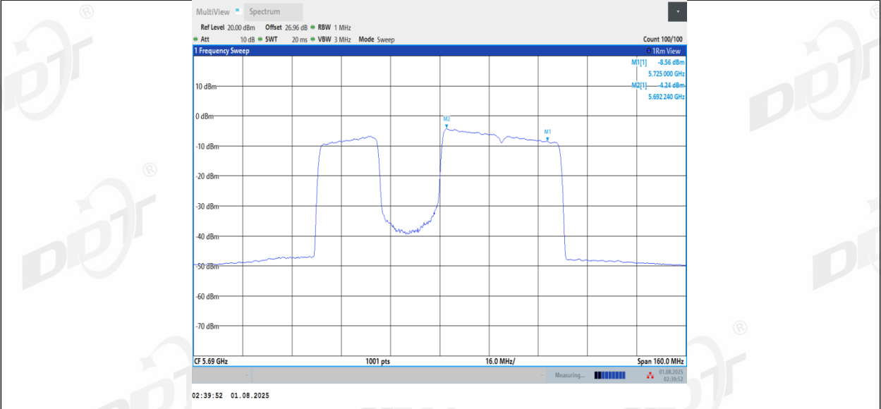
11BE80MIMO Ant1_5690_UNII-2C_484+242_Non-OFDMA 3
