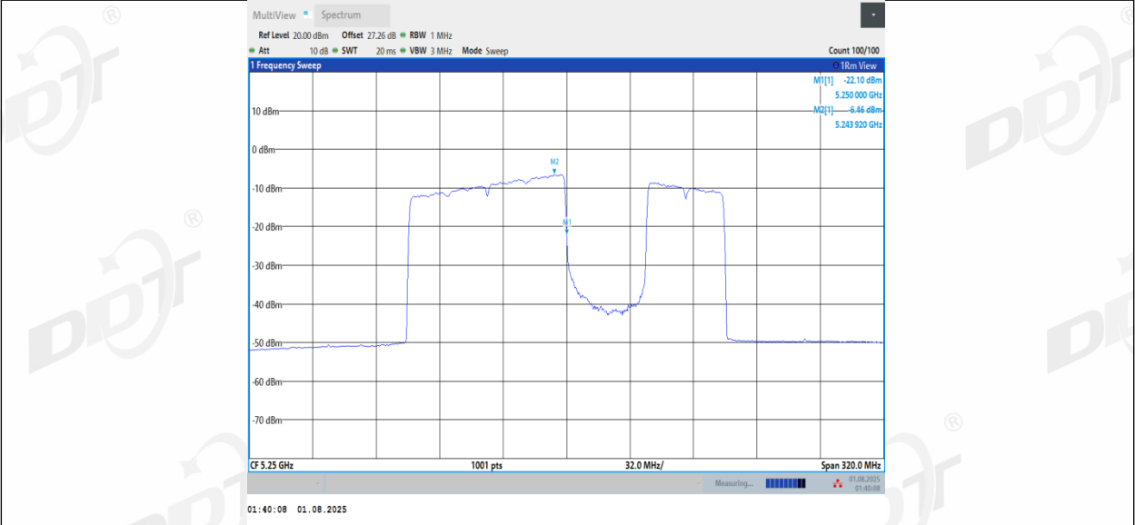
11BE160MIMO_Ant3_5250_UNII-1_996+484_Non-OFDMA_4
