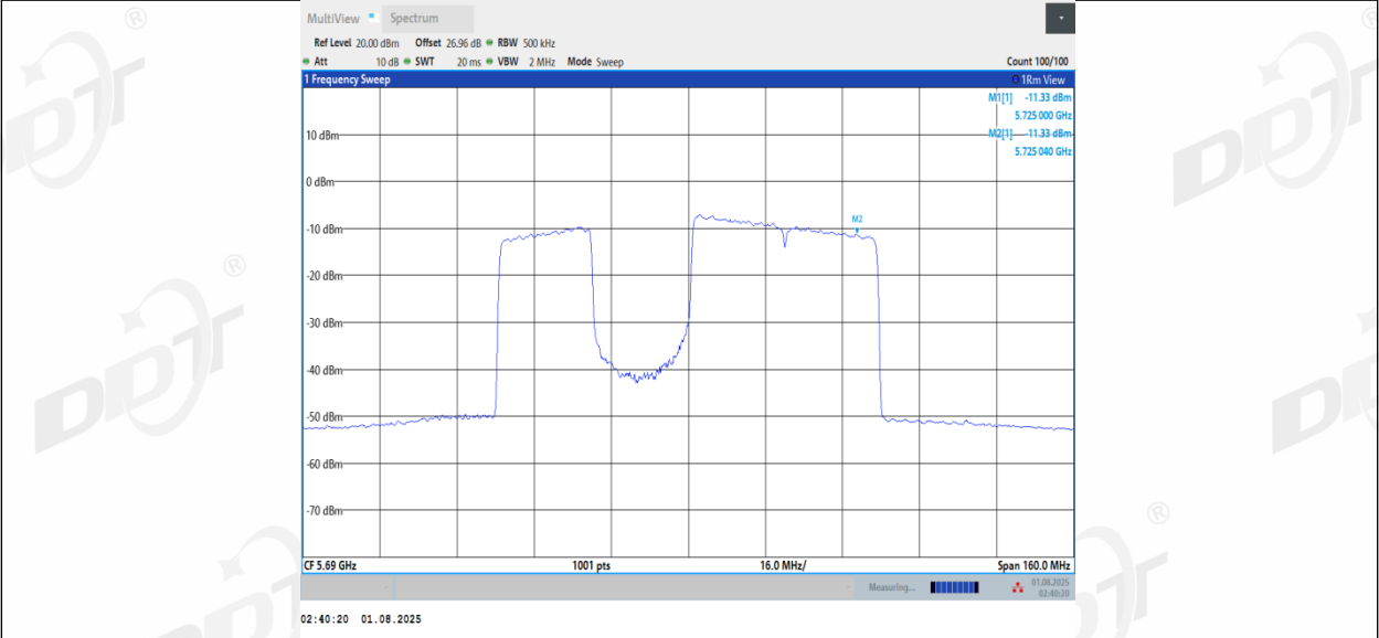
11BE80MIMO_Ant1_5690_UNII-3_484+242_Non-OFDMA_3
