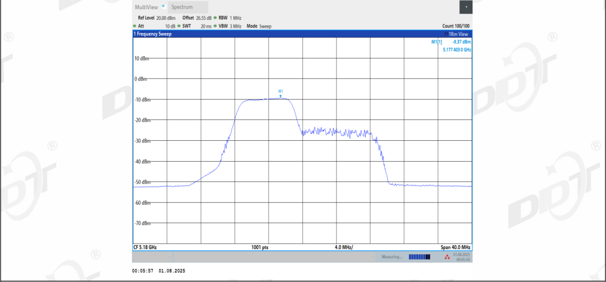
11BE20MIMO_Ant1_5180_52+26_OFDMA_2
