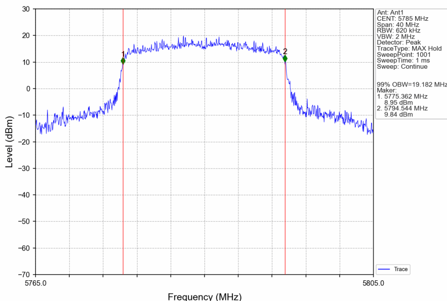
802.11ax(HEW20)_MCH_5785MHz_RU242_Left_Ant1_NTNV
