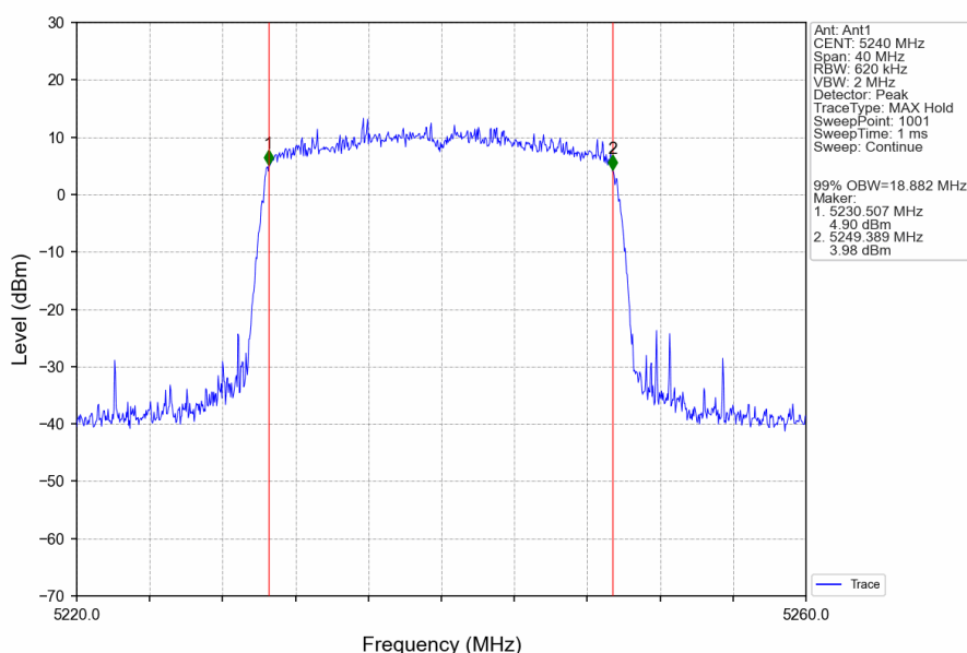
802.11ax(HEW20)_HCH_5240MHz_RU242_Left_Ant1_NTNV
