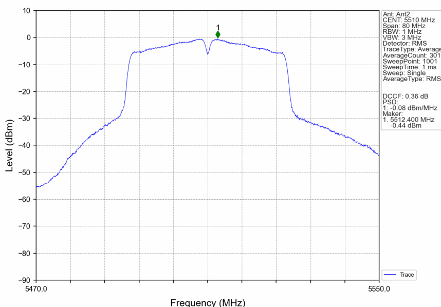
802.11ac(VHT40)_LCH_5510MHz_Ant2_NTNV
