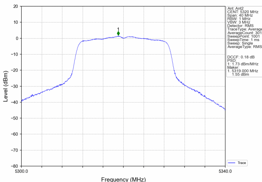
802.11ac(VHT20)_HCH_5320MHz_Ant2_NTNV
