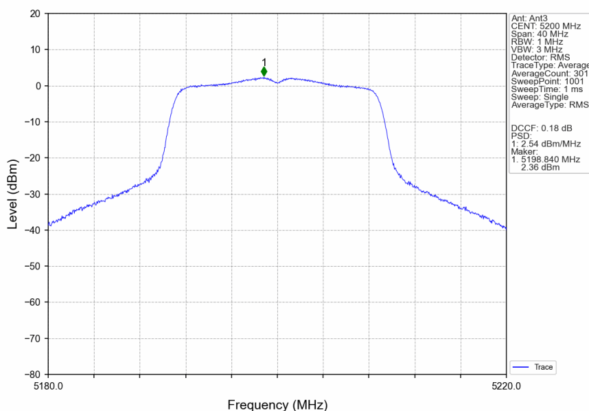
802.11ac(VHT20)_MCH_5200MHz_MIMO_NTNV
