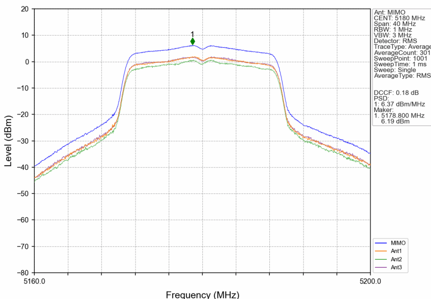
802.11ac(VHT20)_LCH_5180MHz_MIMO_NTNV
