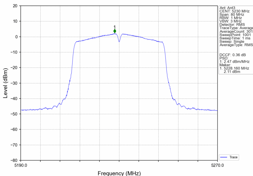
802.11n(HT40)_HCH_5230MHz_MIMO_NTNV
