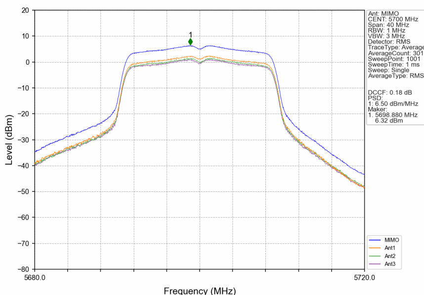
802.11n(HT20)_HCH_5700MHz_MIMO_NTNV
