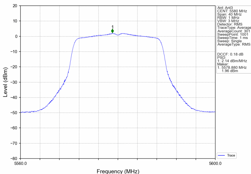
802.11ac(VHT20)_MCH_5580MHz_MIMO_NTNV
