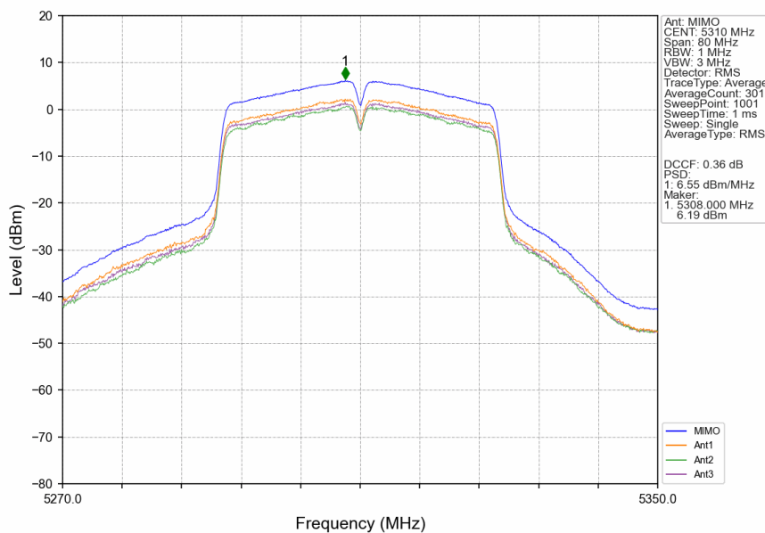
802.11ac(VHT40)_HCH_5310MHz_MIMO_NTNV
