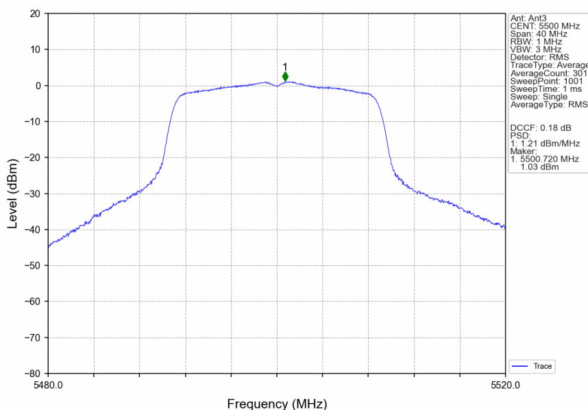
802.11ac(VHT20)_LCH_5500MHz_MIMO_NTNV
