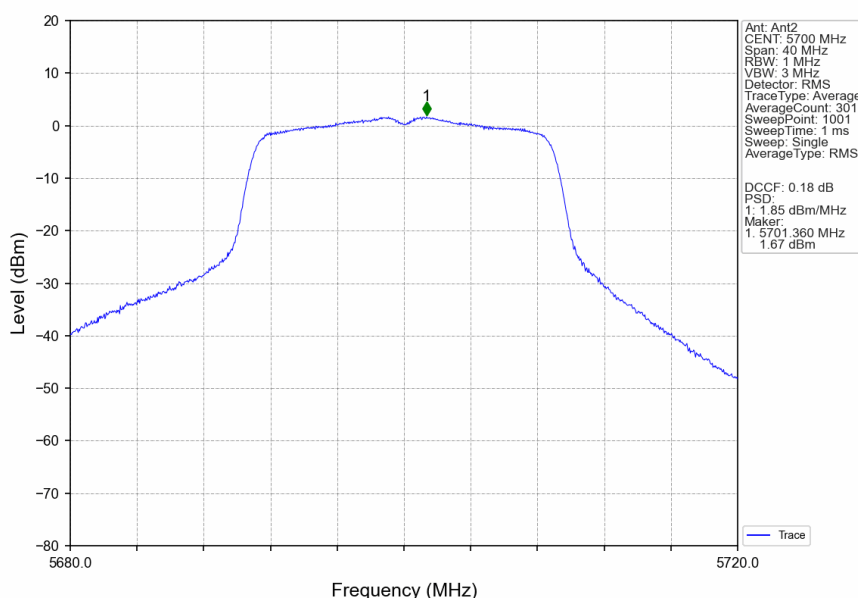
802.11ac(VHT20)_HCH_5700MHz_Ant2_NTNV
