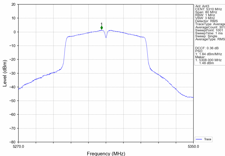
802.11ac(VHT40)_HCH_5310MHz_MIMO_NTNV
