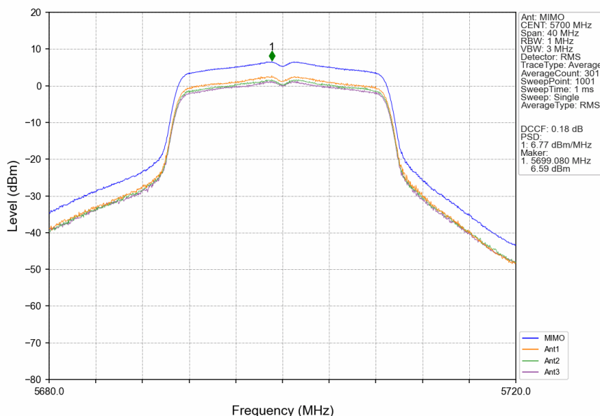
802.11ac(VHT20)_HCH_5700MHz_MIMO_NTNV
