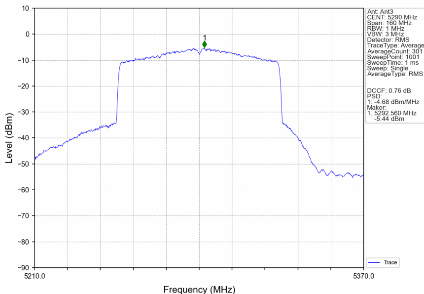
802.11ax(HEW80)_MCH_5290MHz_RU996_Left_MIMO_NTNV
