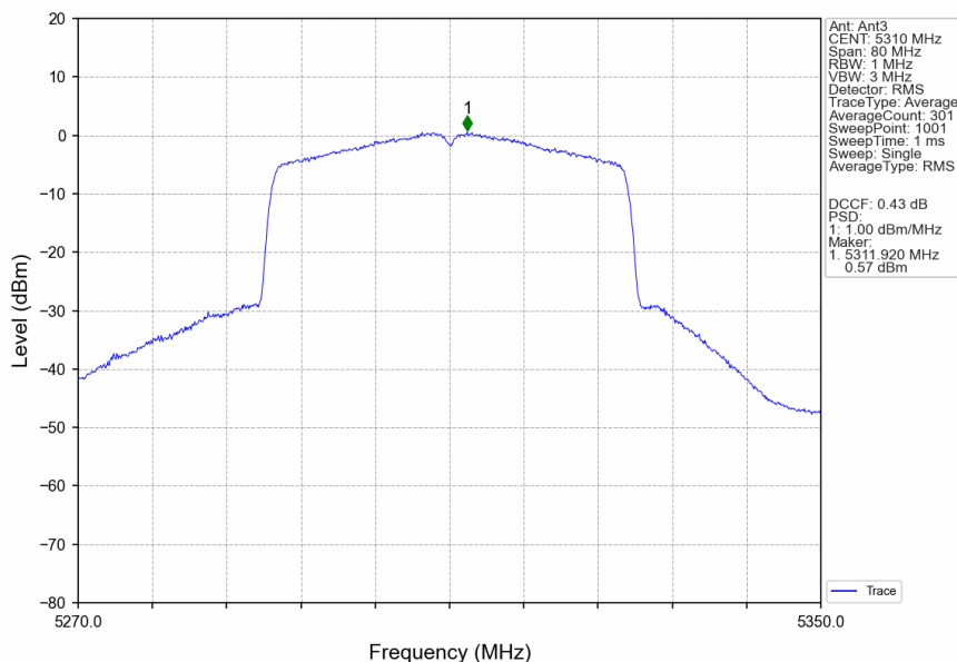
802.11ax(HEW40)_HCH_5310MHz_RU484_Left_MIMO_NTNV
