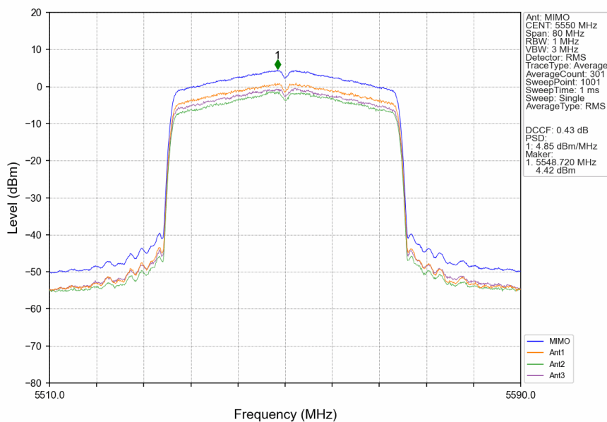
802.11ax(HEW40)_MCH_5550MHz_RU484_Left_MIMO_NTNV
