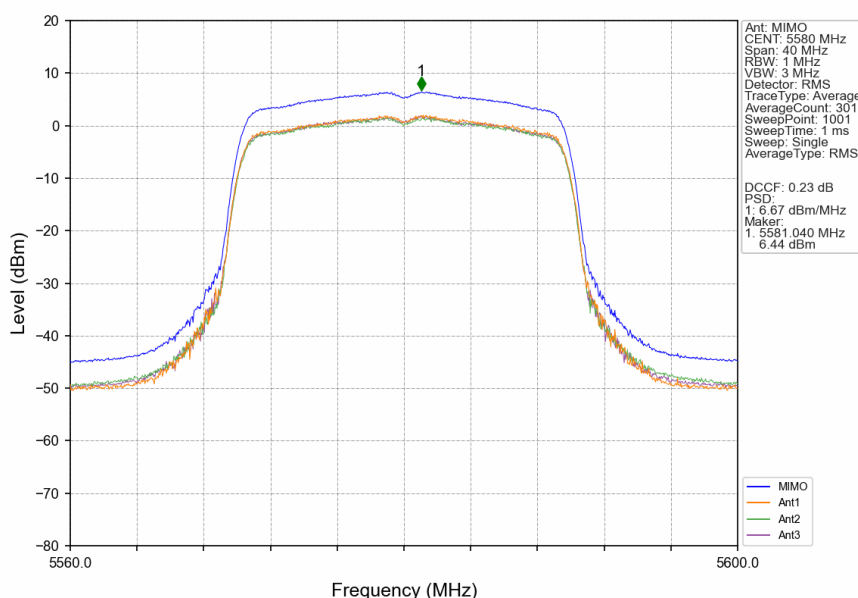
802.11ax(HEW20)_MCH_5580MHz_RU242_Left_MIMO_NTNV
