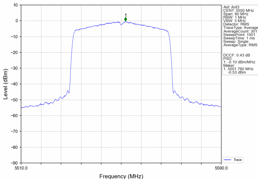
802.11ax(HEW40)_MCH_5550MHz_RU484_Left_MIMO_NTNV
