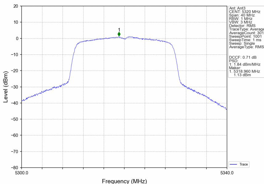
802.11ax(HEW20)_HCH_5320MHz_RU242_Left_MIMO_NTNV
