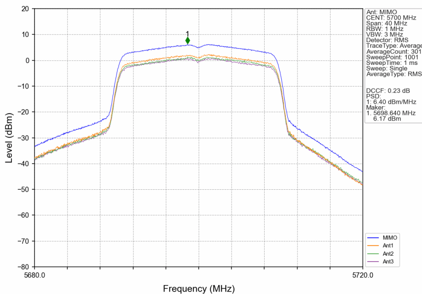
802.11ax(HEW20)_HCH_5700MHz_RU242_Left_MIMO_NTNV
