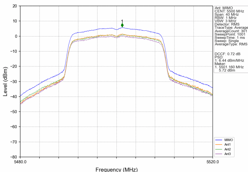
802.11ax(HEW20)_LCH_5500MHz_RU242_Left_MIMO_NTNV
