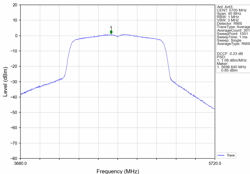
802.11ax(HEW20)_HCH_5700MHz_RU242_Left_MIMO_NTNV
