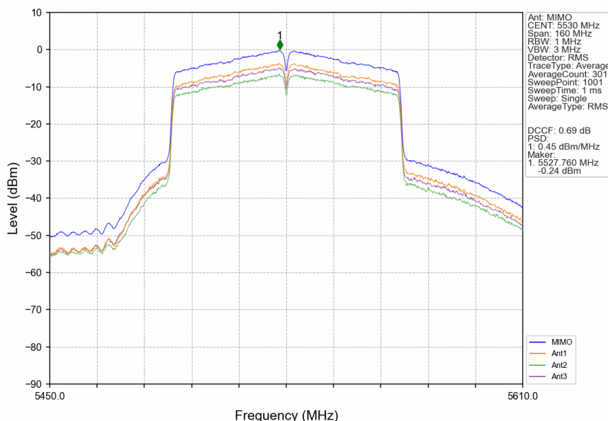
802.11ac(VHT80)_LCH_5530MHz_MIMO_NTNV
