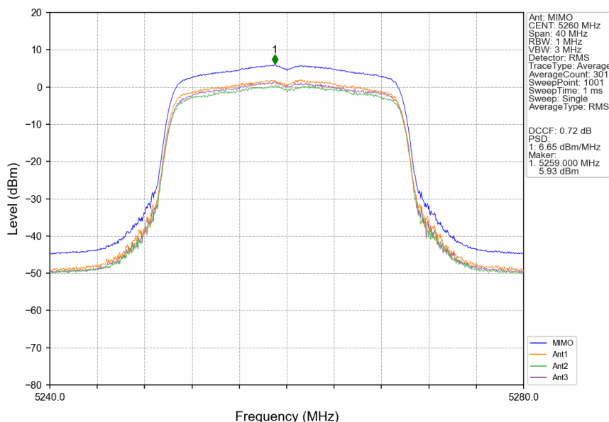
802.11ax(HEW20)_LCH_5260MHz_RU242_Left_MIMO_NTNV
