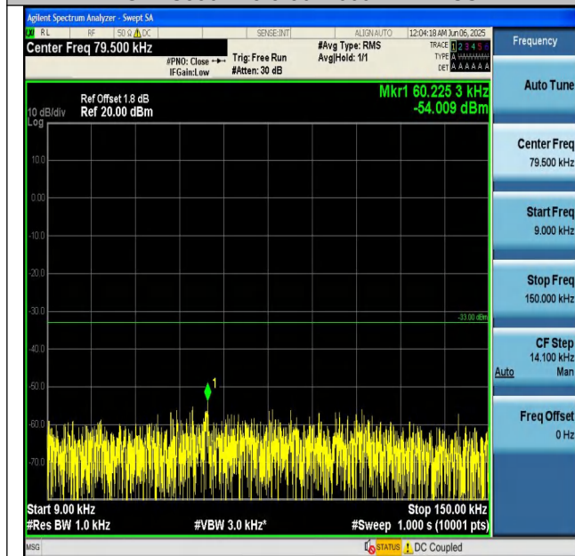
GPRS850-190-5-0.009~0.15MHz-PASS
