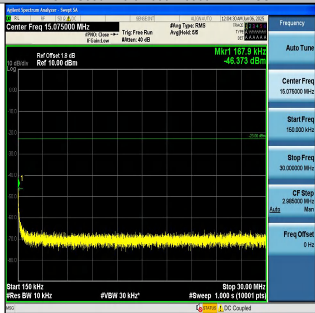
GPRS850-190-5-0.15~30MHz-PASS
