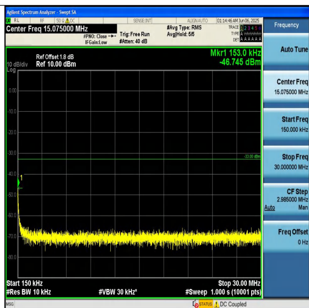
EGPRS1900-512-2-0.15~30MHz-PASS
