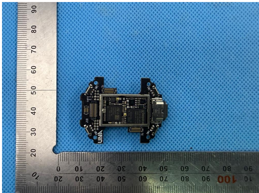
INTERNAL VIEW OF EUT (FIGURE 10)
