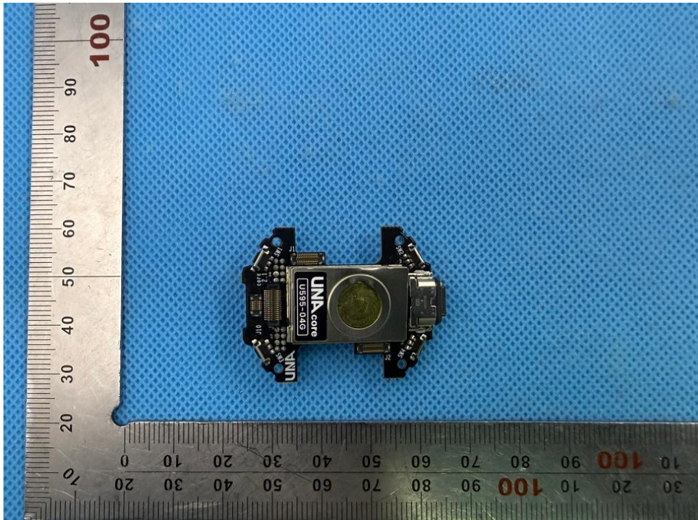
INTERNAL VIEW OF EUT (FIGURE 9)
