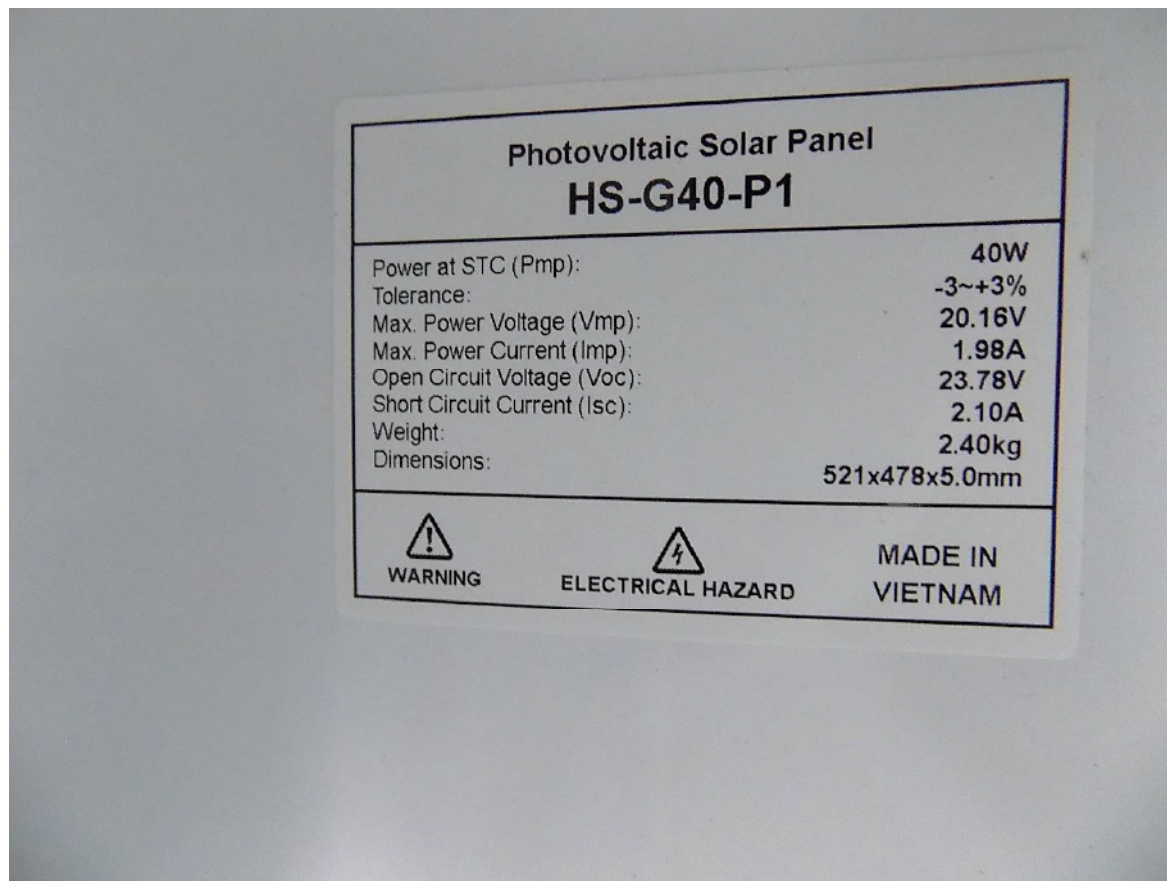
Figure 63 – External Photo of EUT View 4
