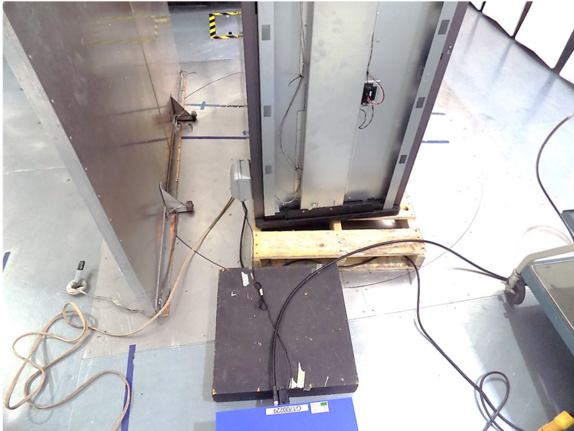
Figure 57: AC Main Conducted Emissions Side View
