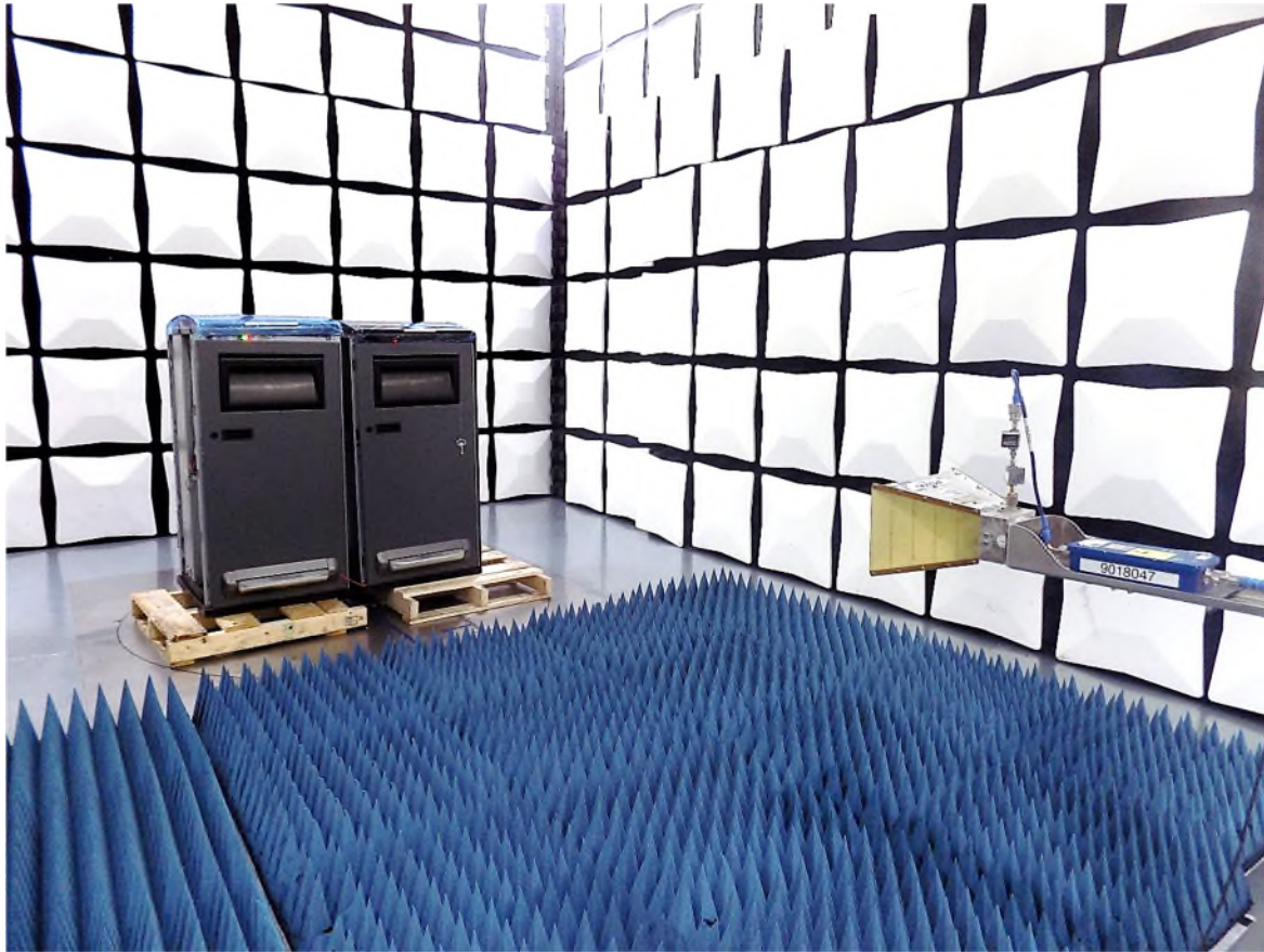
Figure 55: Radiated Emissions 1000 – 18000 MHz
