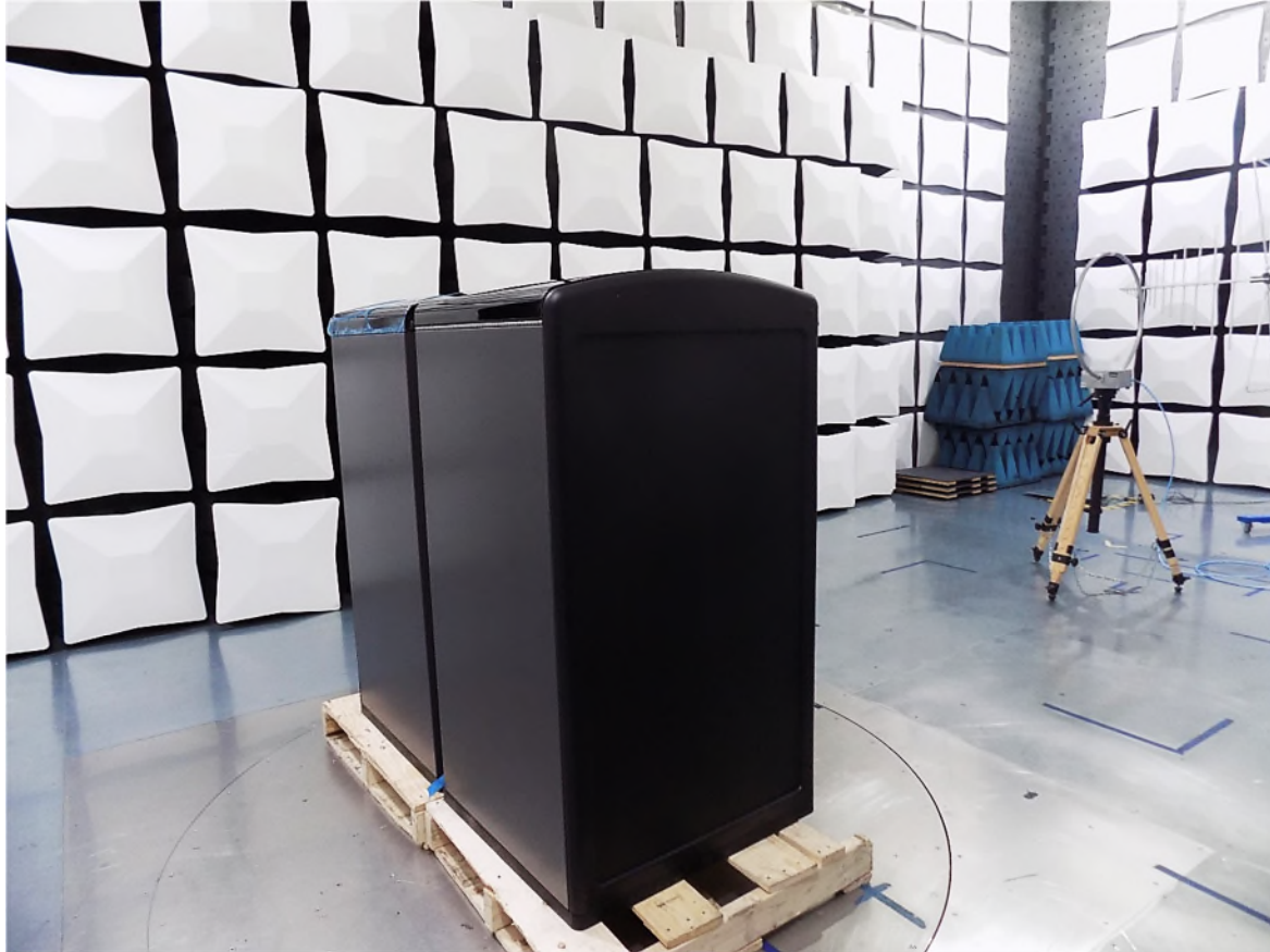
Figure 52: Radiated Emissions 9 kHz – 30 MHz View 1
