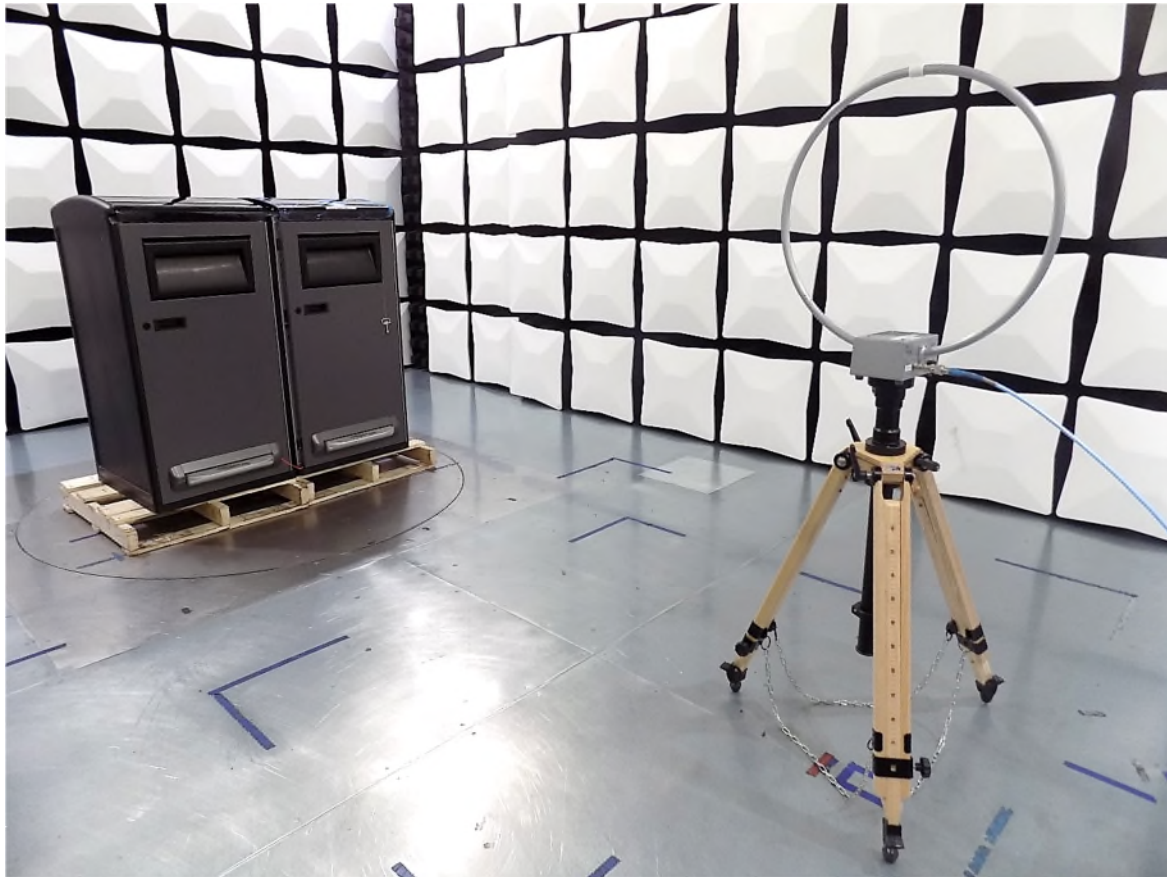
Figure 53: Radiated Emissions 9 kHz – 30 MHz View 2
