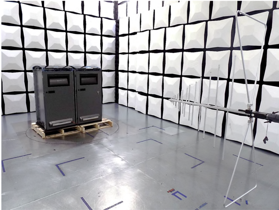
Figure 54: Radiated Emissions 30 – 1000 MHz
