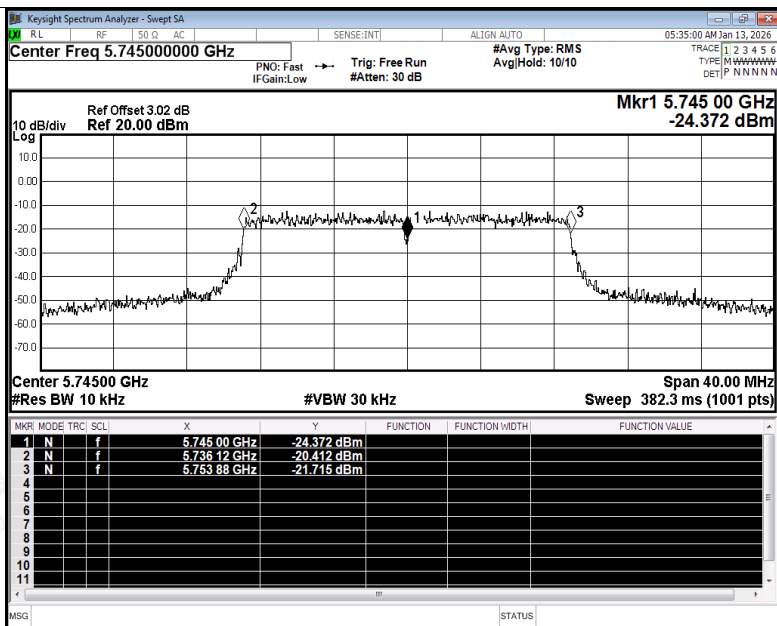
Freq. Stability NVNT ac20 5745MHz Ant1
