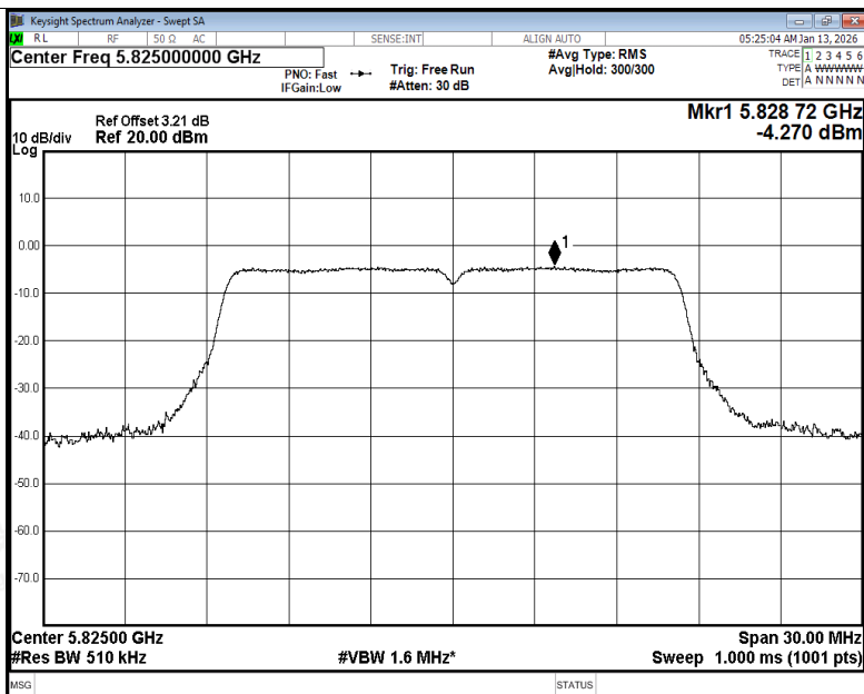
PSD NVNT a 5825MHz Ant1
