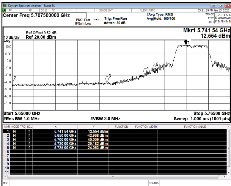
Restrict Band NVNT a 5745MHz Ant1 Peak
