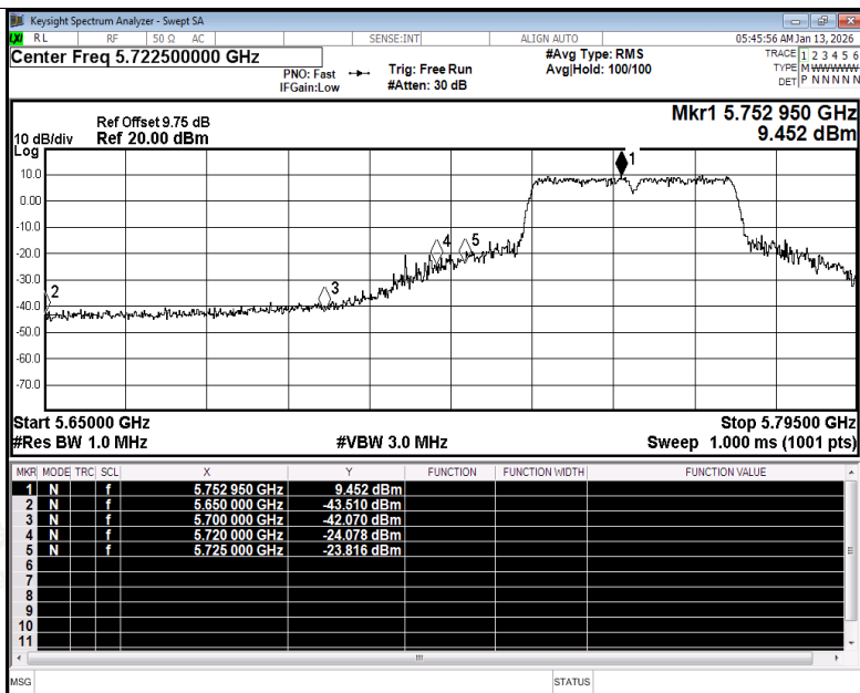
Restrict Band NVNT ac40 5755MHz Ant1 Peak
