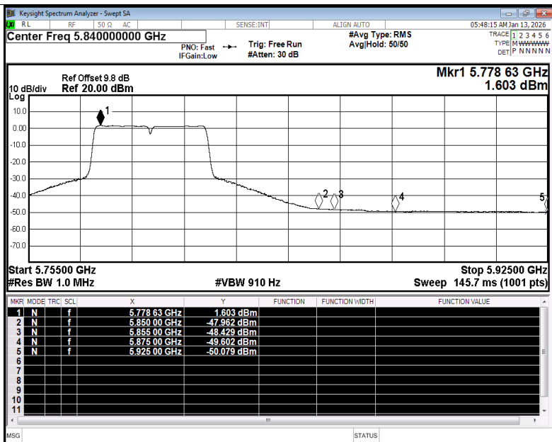
Restrict Band NVNT ac40 5795MHz Ant1 Average
