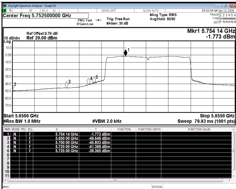
Restrict Band NVNT ac80 5775MHz Ant1 Average
