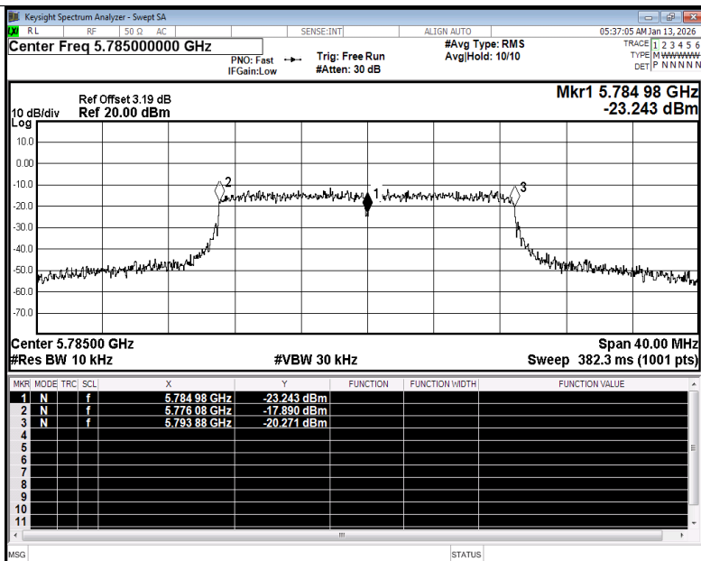
Freq. Stability NVNT ac20 5785MHz Ant1
