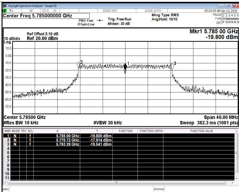
Freq. Stability NVNT a 5785MHz Ant1
