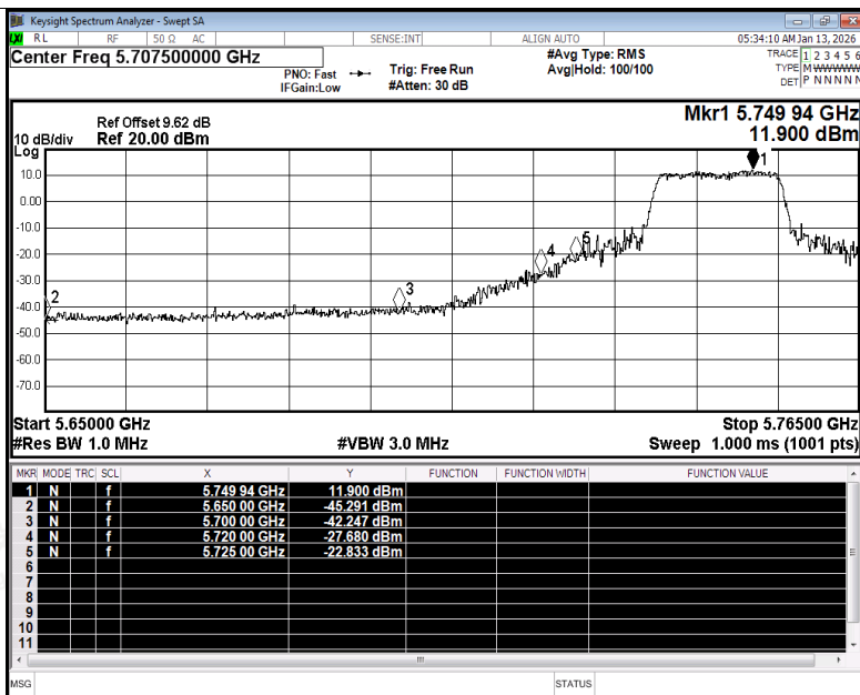
Restrict Band NVNT ac20 5745MHz Ant1 Peak
