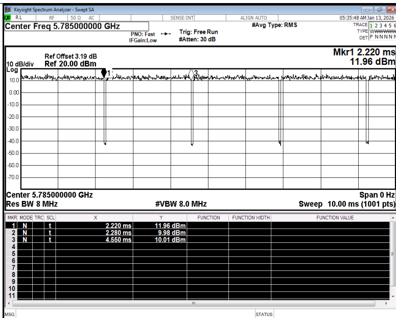
Duty Cycle NVNT ac20 5785MHz Ant1
