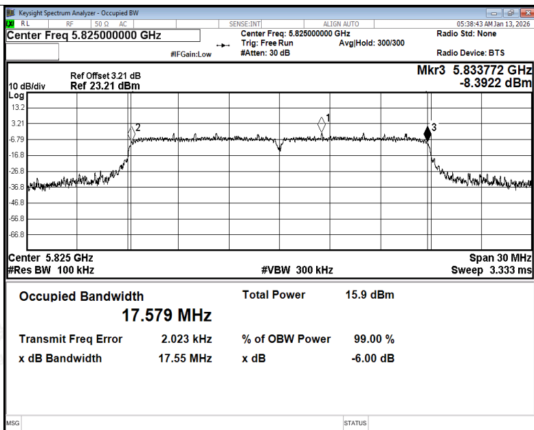
-6dB Bandwidth NVNT ac20 5825MHz Ant1
