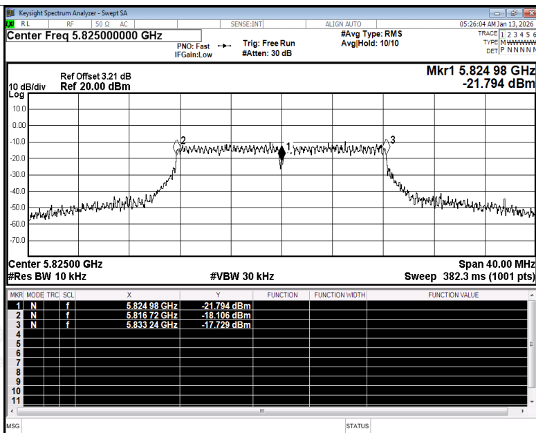
Freq. Stability NVNT a 5825MHz Ant1
