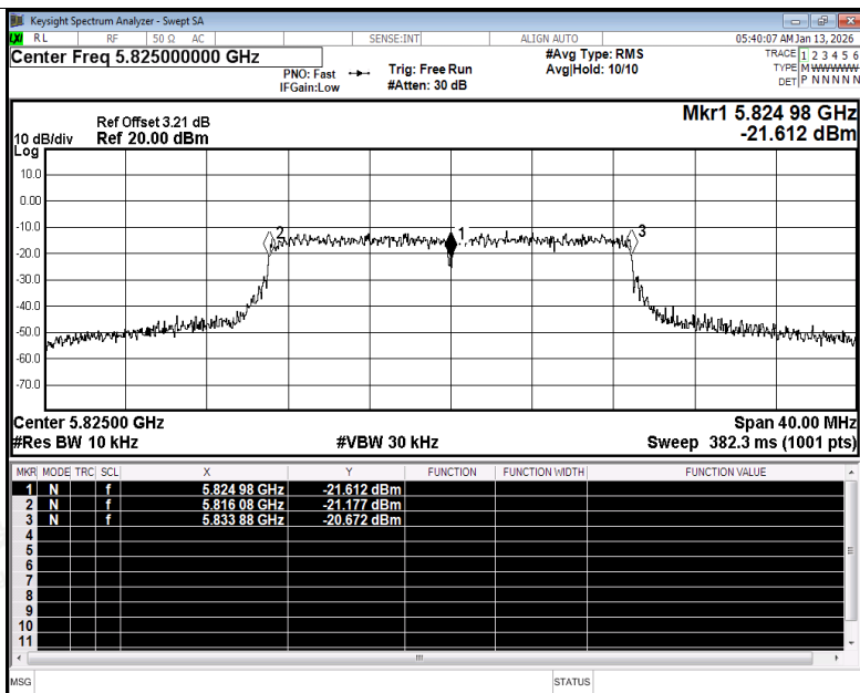
Freq. Stability NVNT ac20 5825MHz Ant1
