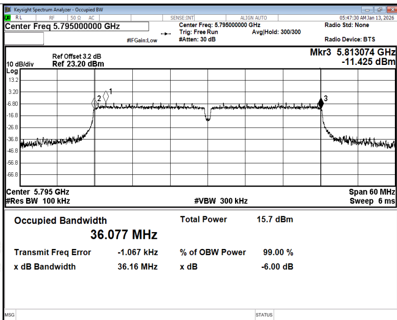
-6dB Bandwidth NVNT ac40 5795MHz Ant1
