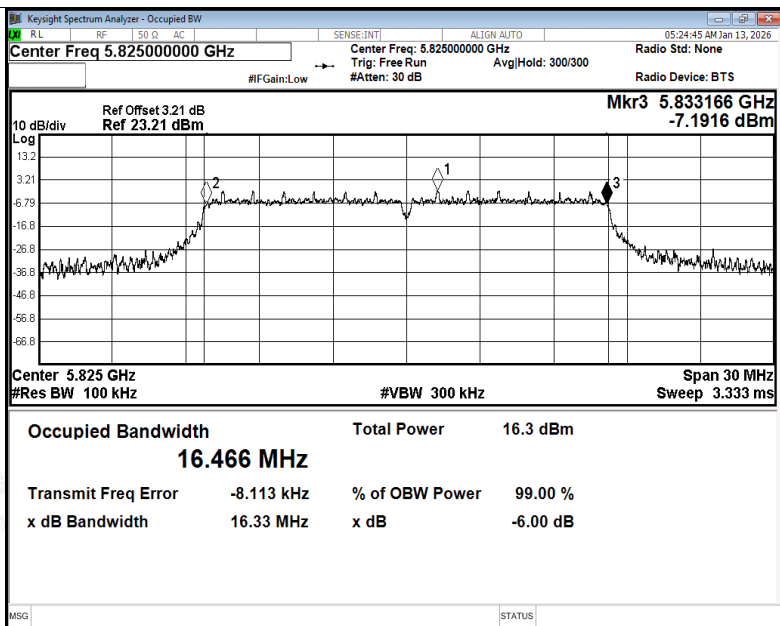
-6dB Bandwidth NVNT a 5825MHz Ant1
