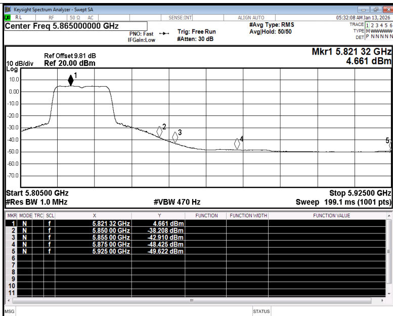
Restrict Band NVNT n20 5825MHz Ant1 Average
