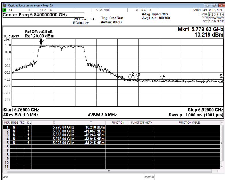
Restrict Band NVNT ac40 5795MHz Ant1 Peak
