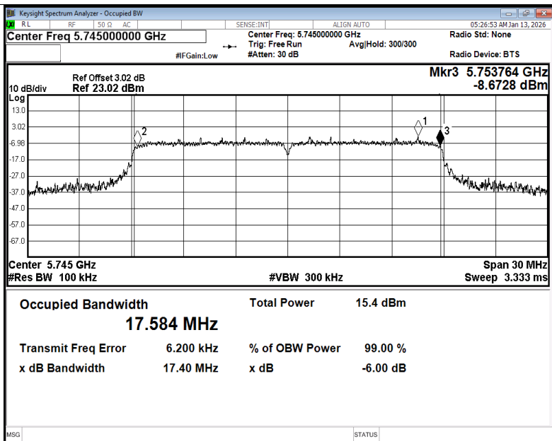
-6dB Bandwidth NVNT n20 5745MHz Ant1
