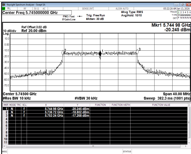
Freq. Stability NVNT a 5745MHz Ant1
