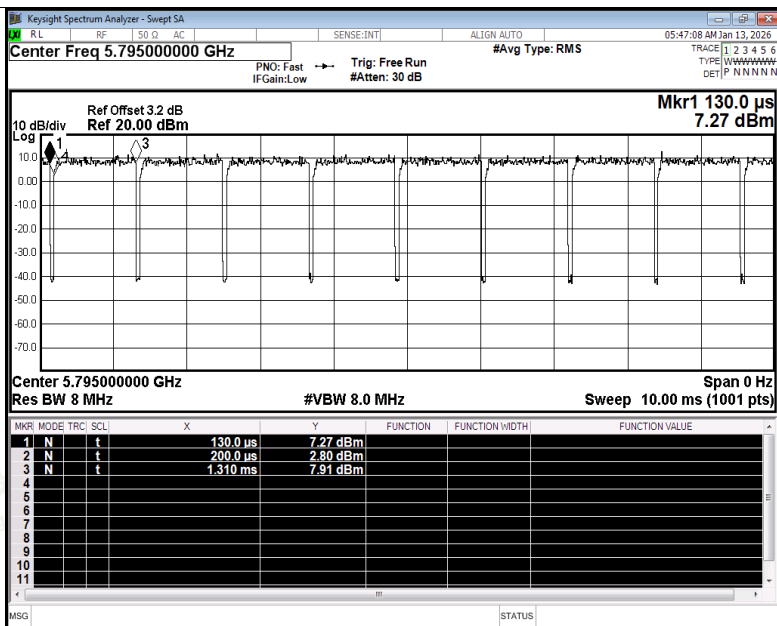
Duty Cycle NVNT ac40 5795MHz Ant1
