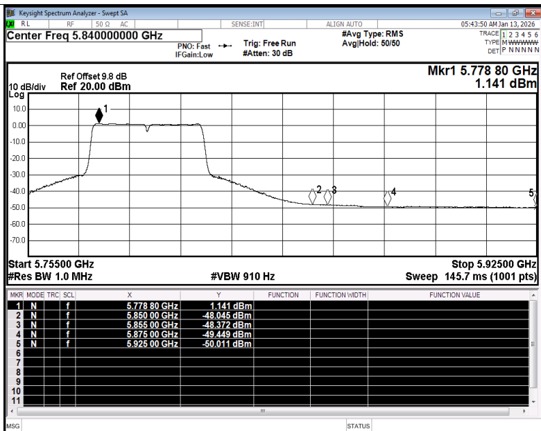
Restrict Band NVNT n40 5795MHz Ant1 Average
