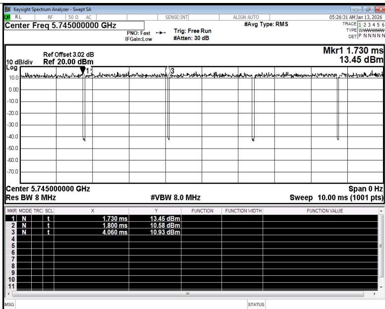
Duty Cycle NVNT n20 5745MHz Ant1
