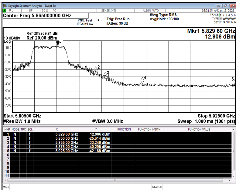
Restrict Band NVNT n20 5825MHz Ant1 Peak
