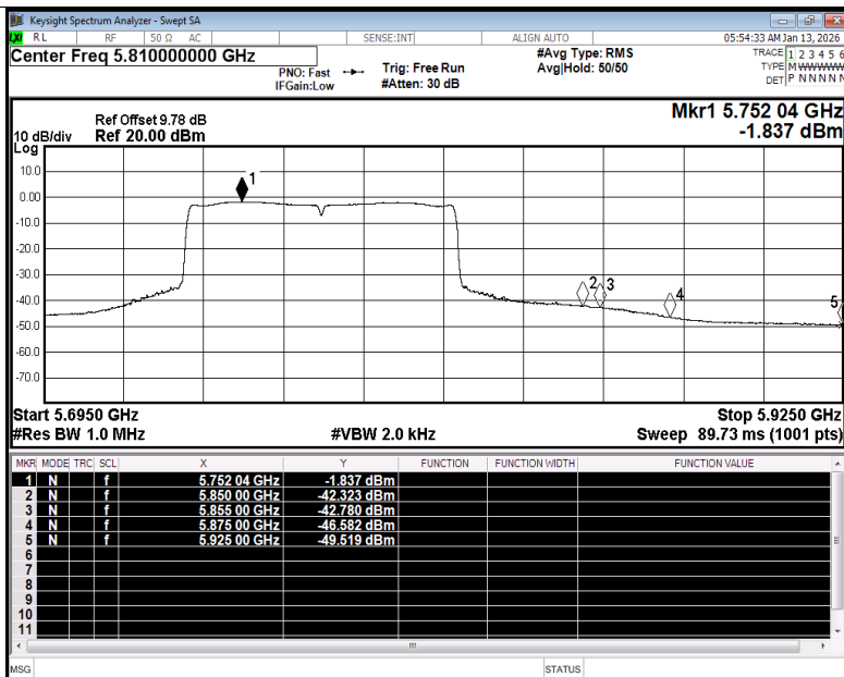
Restrict Band NVNT ac80 5775MHz Ant1 Average
