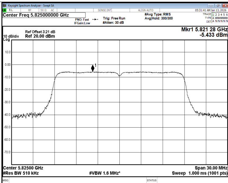
PSD NVNT n20 5825MHz Ant1
