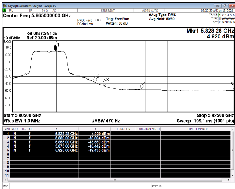
Restrict Band NVNT ac20 5825MHz Ant1 Average
