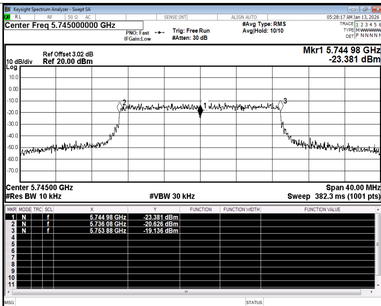
Freq. Stability NVNT n20 5745MHz Ant1
