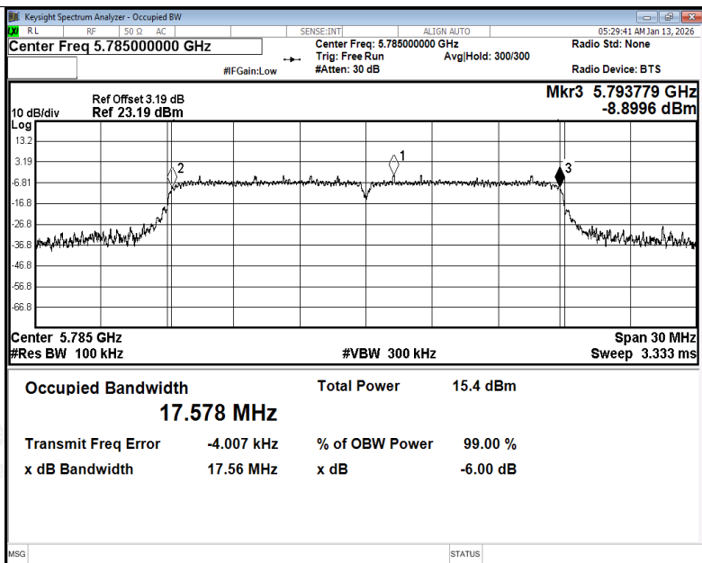
-6dB Bandwidth NVNT n20 5785MHz Ant1
