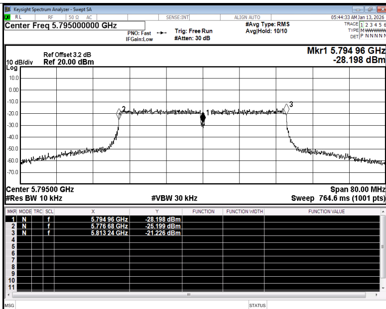
Freq. Stability NVNT n40 5795MHz Ant1
