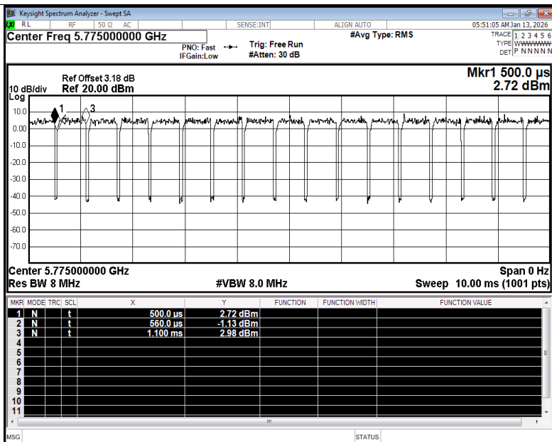
Duty Cycle NVNT ac80 5775MHz Ant1
