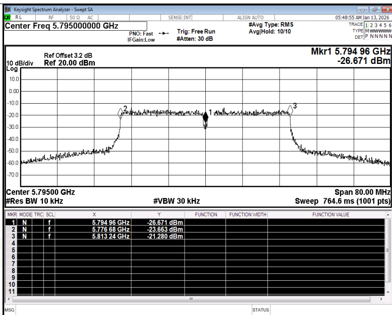
Freq. Stability NVNT ac40 5795MHz Ant1
