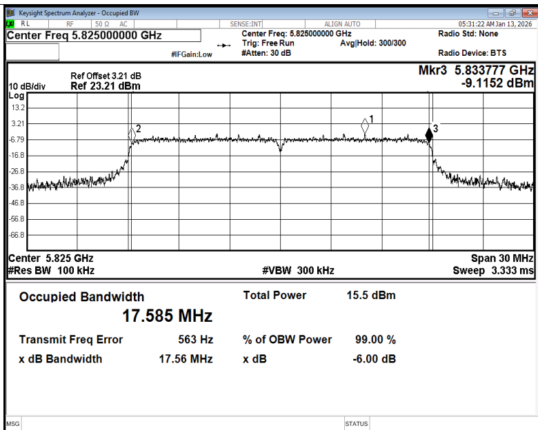
-6dB Bandwidth NVNT n20 5825MHz Ant1
