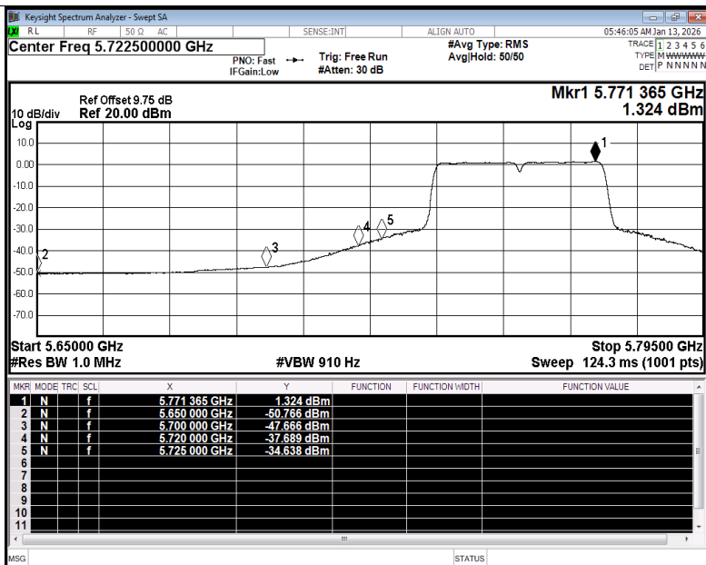
Restrict Band NVNT ac40 5755MHz Ant1 Average
