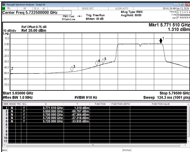
Restrict Band NVNT n40 5755MHz Ant1 Average
