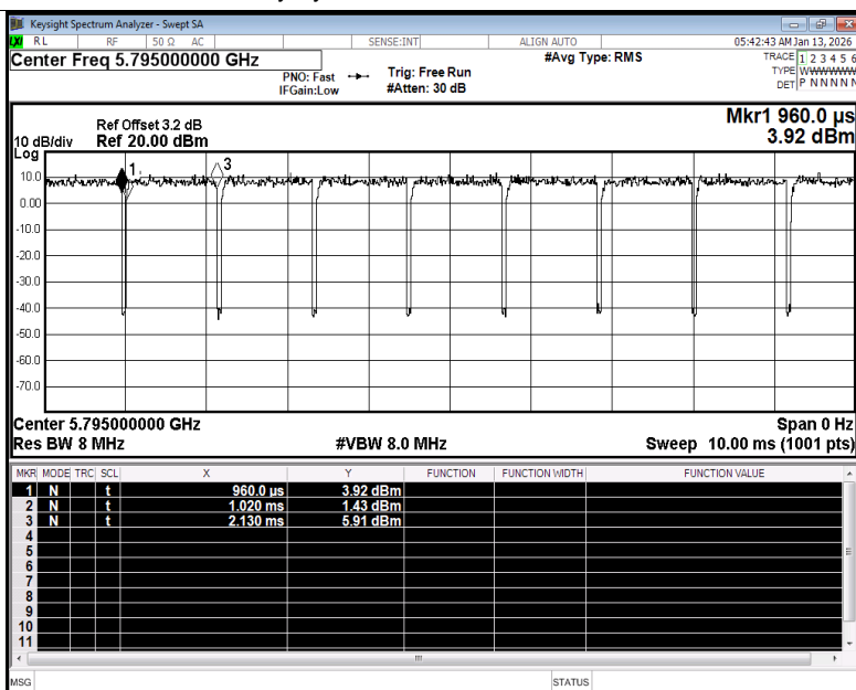
Duty Cycle NVNT n40 5795MHz Ant1
