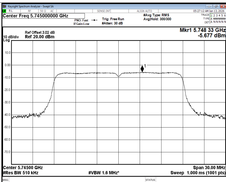
PSD NVNT n20 5745MHz Ant1
