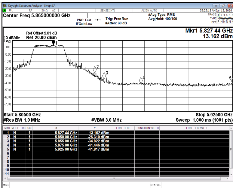
Restrict Band NVNT a 5825MHz Ant1 Peak
