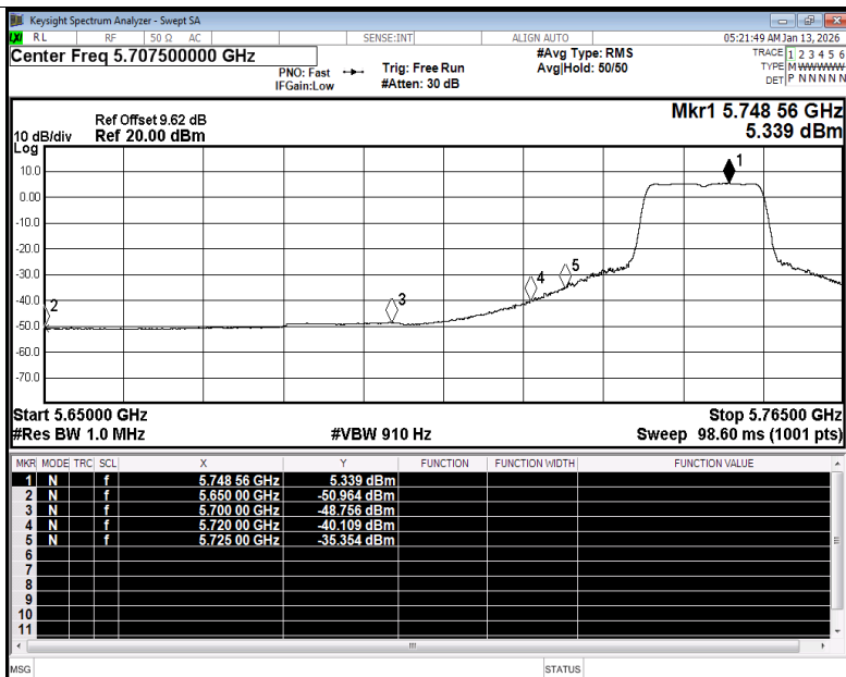
Restrict Band NVNT a 5745MHz Ant1 Average
