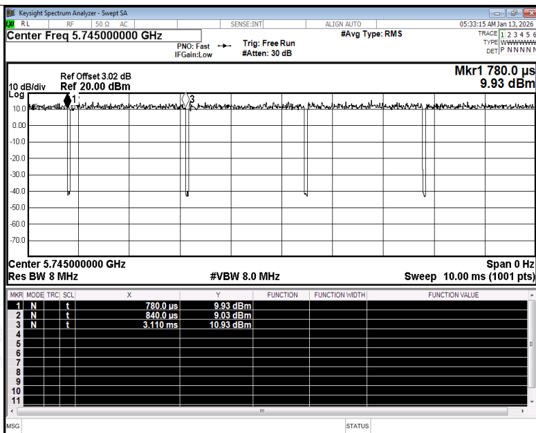
Duty Cycle NVNT ac20 5745MHz Ant1
