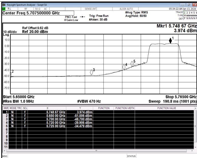
Restrict Band NVNT ac20 5745MHz Ant1 Average
