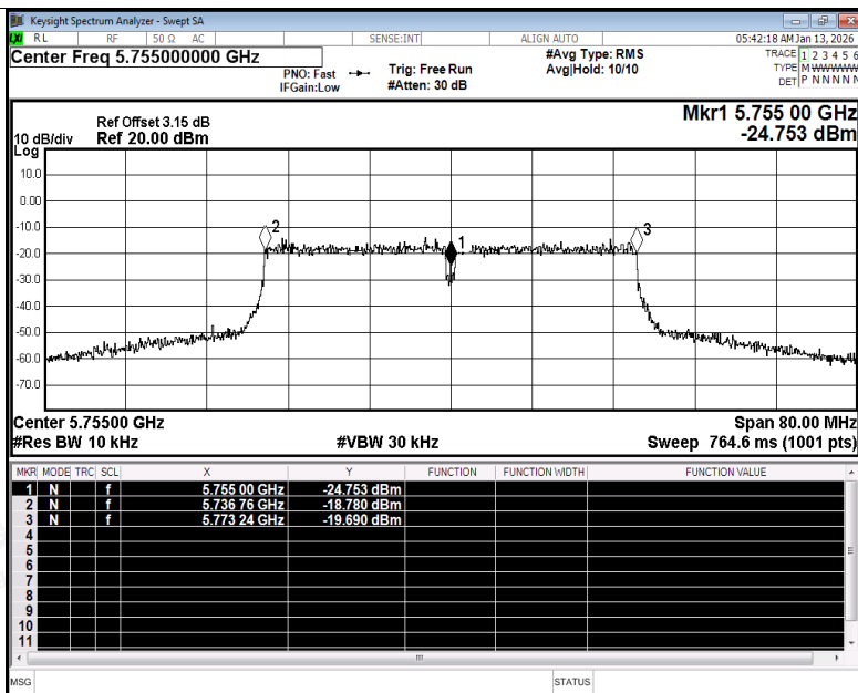
Freq. Stability NVNT n40 5755MHz Ant1
