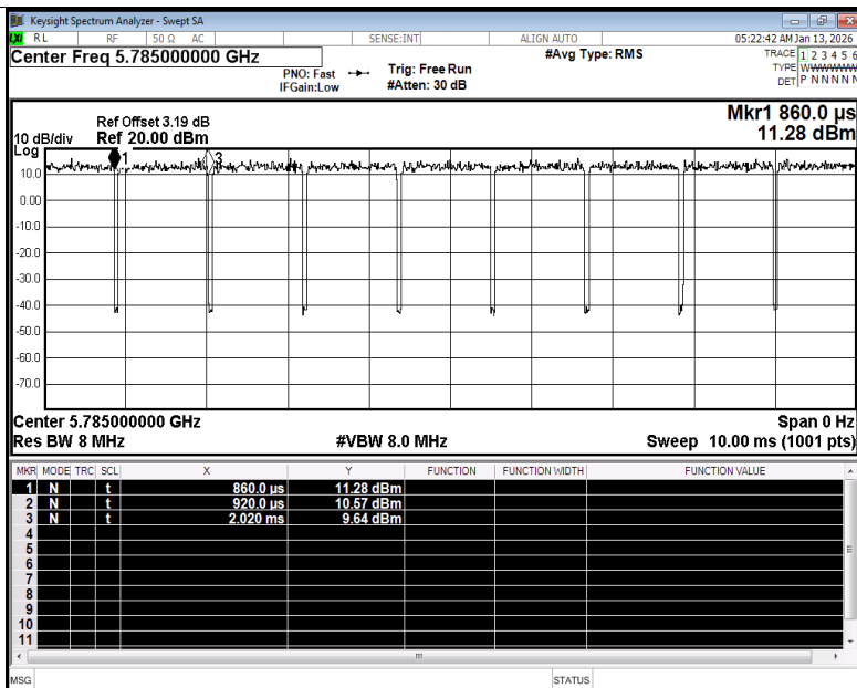
Duty Cycle NVNT a 5785MHz Ant1
