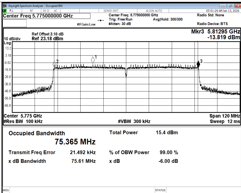
-6dB Bandwidth NVNT ac80 5775MHz Ant1
