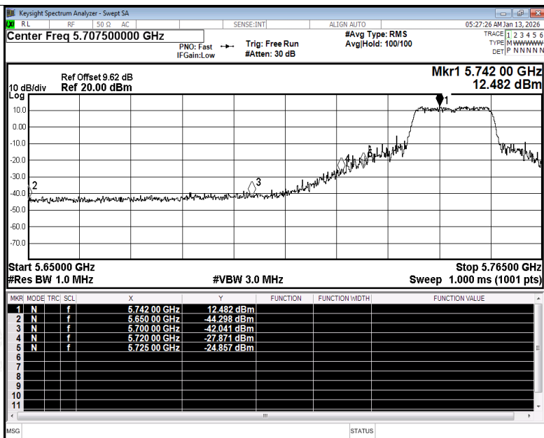
Restrict Band NVNT n20 5745MHz Ant1 Peak
