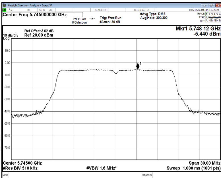
PSD NVNT a 5745MHz Ant1
