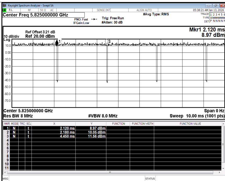
Duty Cycle NVNT ac20 5825MHz Ant1
