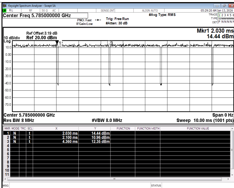
Duty Cycle NVNT n20 5785MHz Ant1
