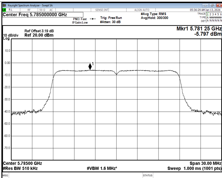
PSD NVNT ac20 5785MHz Ant1
