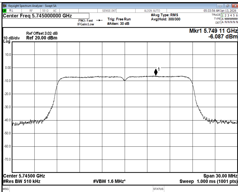
PSD NVNT ac20 5745MHz Ant1
