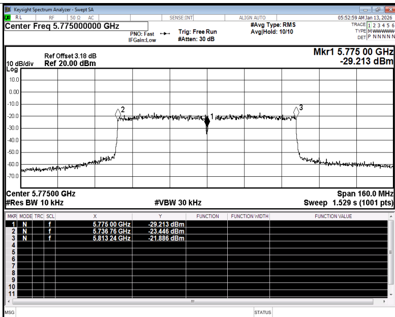
Freq. Stability NVNT ac80 5775MHz Ant1
