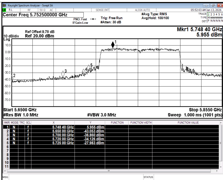
Restrict Band NVNT ac80 5775MHz Ant1 Peak
