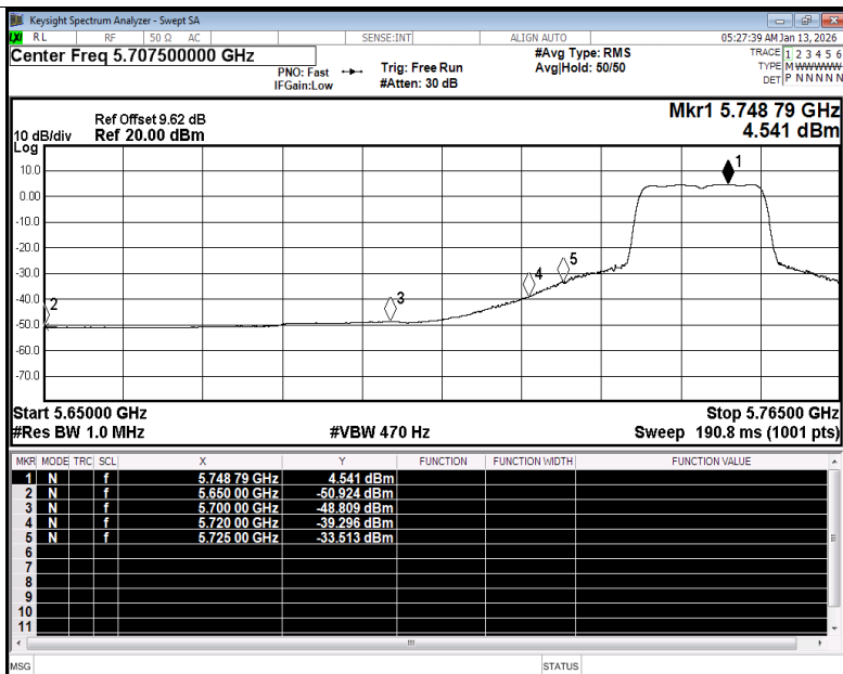
Restrict Band NVNT n20 5745MHz Ant1 Average
