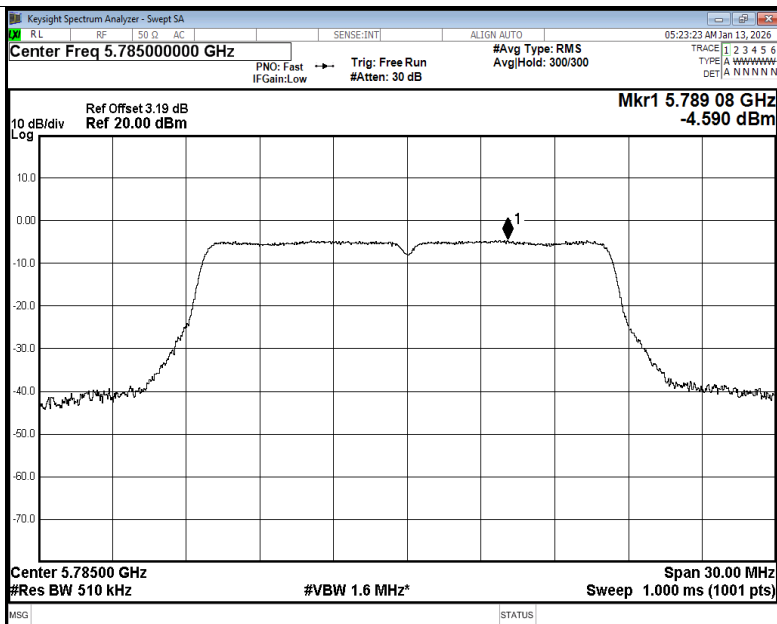
PSD NVNT a 5785MHz Ant1
