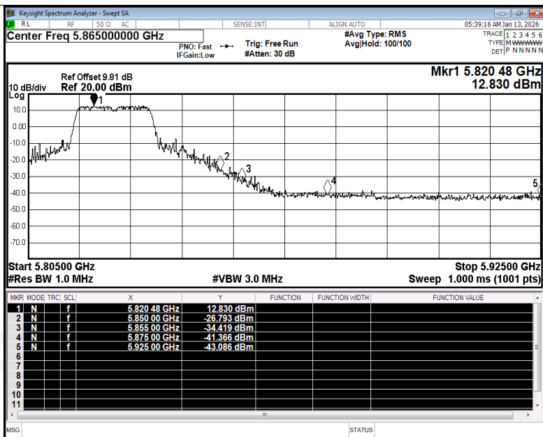
Restrict Band NVNT ac20 5825MHz Ant1 Peak
