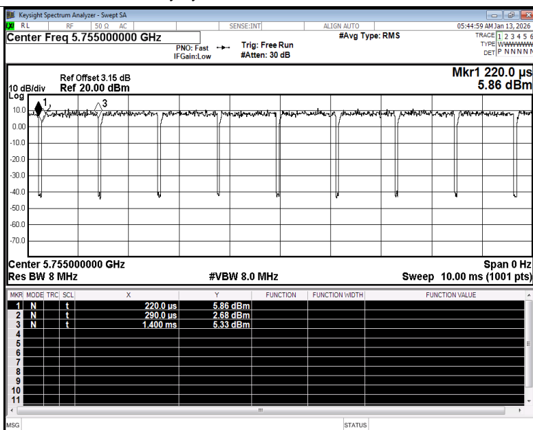
Duty Cycle NVNT ac40 5755MHz Ant1
