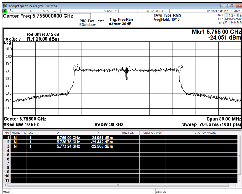
Freq. Stability NVNT ac40 5755MHz Ant1
