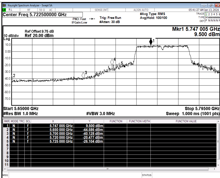
Restrict Band NVNT n40 5755MHz Ant1 Peak
