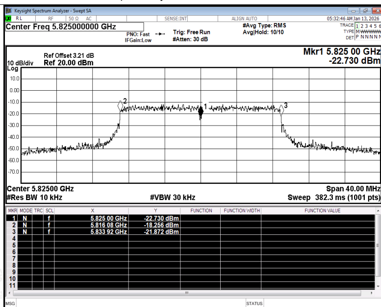
Freq. Stability NVNT n20 5825MHz Ant1
