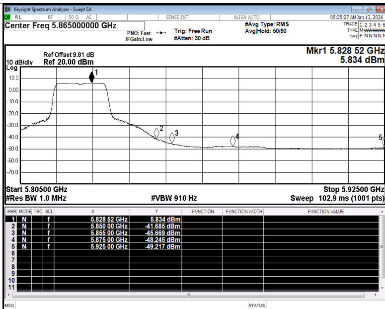
Restrict Band NVNT a 5825MHz Ant1 Average
