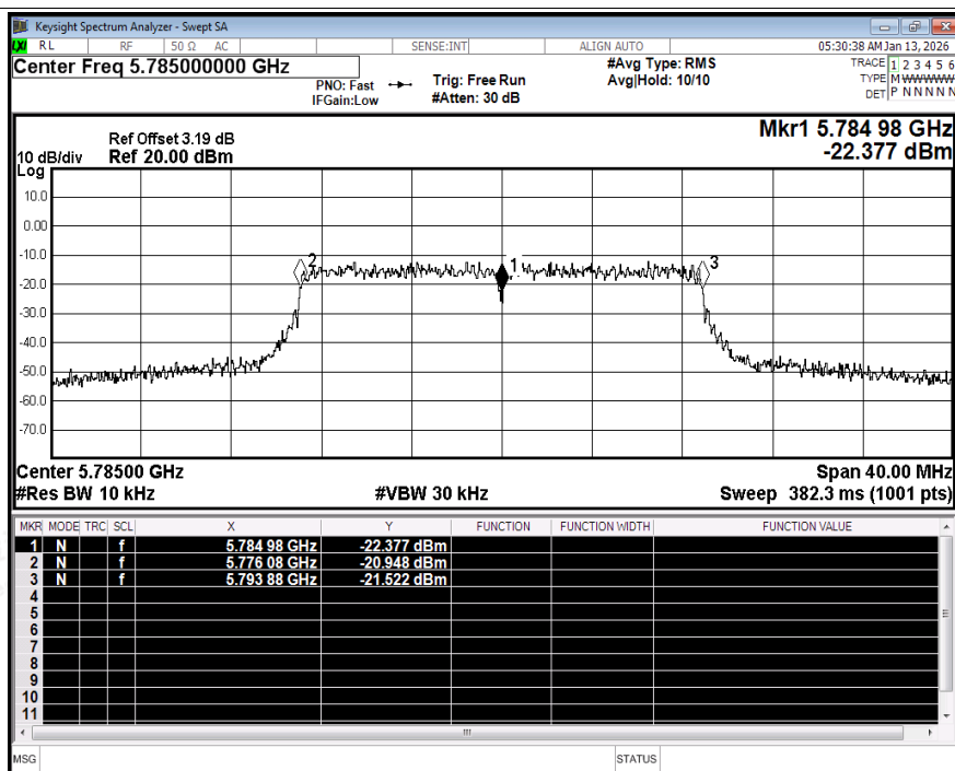
Freq. Stability NVNT n20 5785MHz Ant1
