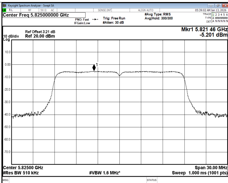
PSD NVNT ac20 5825MHz Ant1
