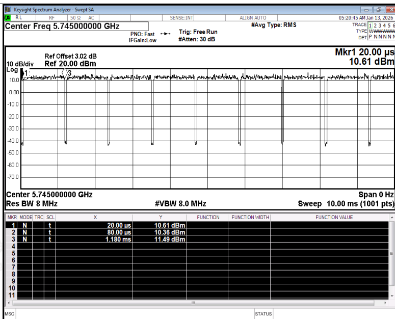
Duty Cycle NVNT a 5745MHz Ant1
