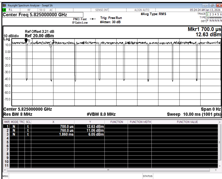
Duty Cycle NVNT a 5825MHz Ant1
