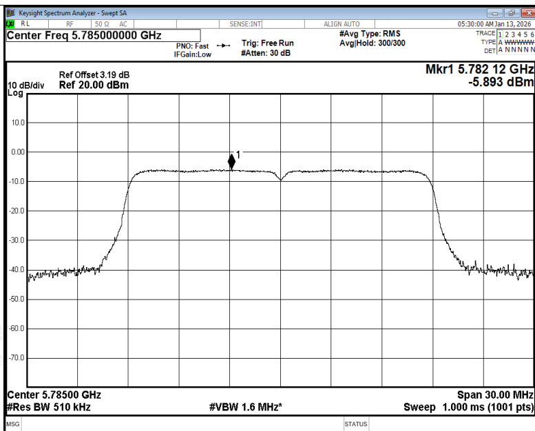
PSD NVNT n20 5785MHz Ant1
