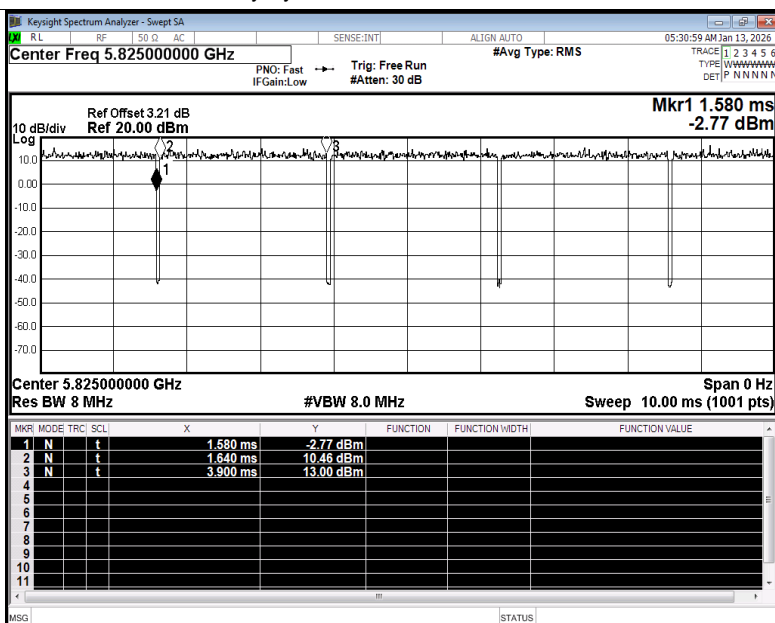
Duty Cycle NVNT n20 5825MHz Ant1
